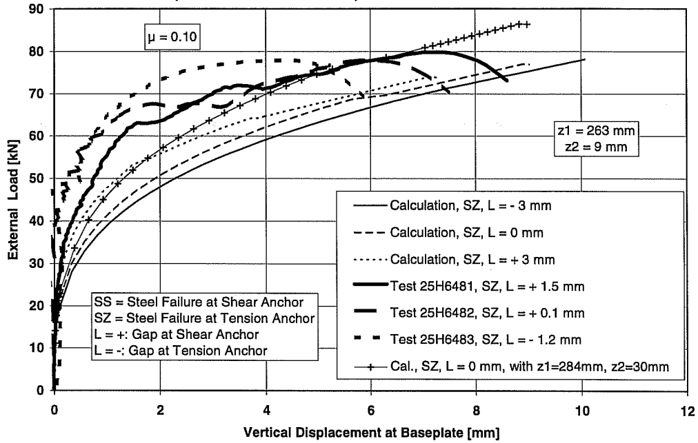
Series 25H648, Sleeve M16, e = 18 inches (457.2 mm), f_c = 32.4 \text{ N/mm}^2 Vertical Displacement at Center of Baseplate in Calculation and Test
