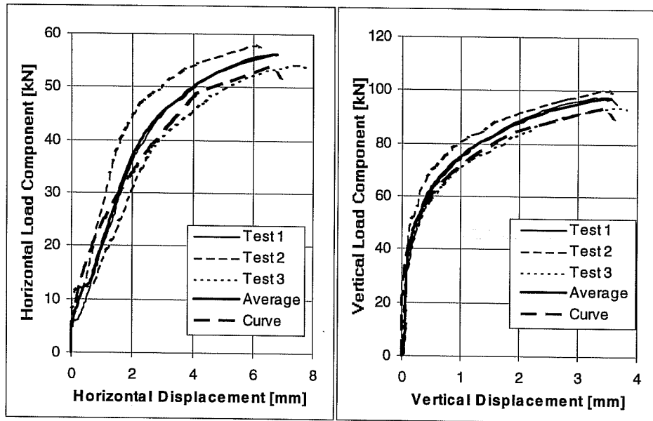
Load-Displacement Curves of Series 23m543. UC1 Anchors 5/8 inches, h_{ef} = 7 inches (178 mm), c_1 \geq 11 inches (279 mm). f_c = 32.4 N/mm 2 , Loading Angle 30° from Anchor Axis
