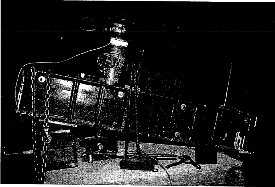
Test Setup of Series 2.3, Oblique Tension Tests at 15° with Steel Failure
