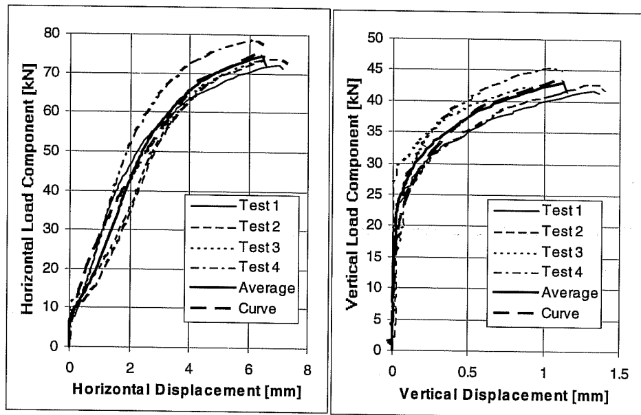
Load-Displacement Curves of Series 23m546. UC1 Anchors 5/8 inches, hef = 7 inches (178 mm), c1 3 11 inches (279 mm). f c = 32.4 N/mm 2 , Loading Angle 60° from Anchor Axis
