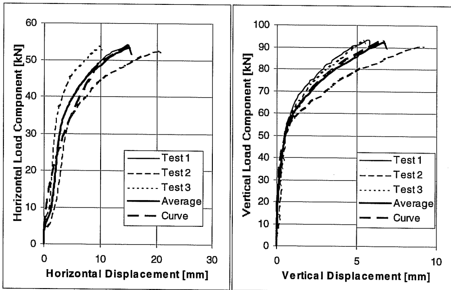
Load-Displacement Curves of Series 23m533. UC1 Anchors 5/8 inches, hef = 7 inches (178 mm), c1 = 11 inches (279 mm). f_c = 20.7 \text{ N/mm}^2 , Loading Angle 30^\circ from Anchor Axis
