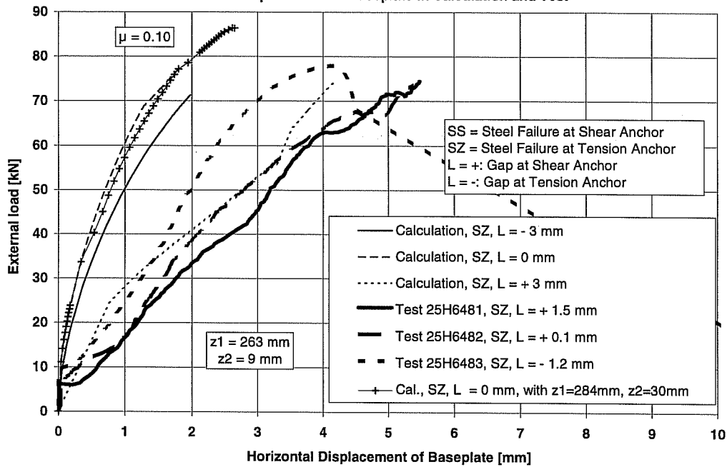
Series 25H648, Sleeve M16, e = 18 inches (457.2 mm), f_c = 32.4 \text{ N/mm}^2 Horizontal Displacement of Baseplate in Calculation and Test
