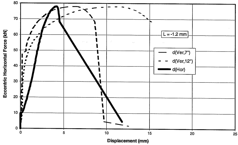
Test 25H6483, Sleeve M16, e = 18 inches (457.2 mm) Steel Failure of Tension Anchor - Results of Displacement Measurement -
