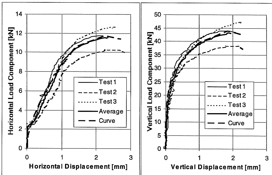
Load-Displacement Curves Series 23m341. UC1 Anchors 3/8 inches, hef = 7 inches (178 mm), c1 3 11 inches (279 mm). f c = 32.4 N/mm 2 , Loading Angle 15° from Anchor Axis
