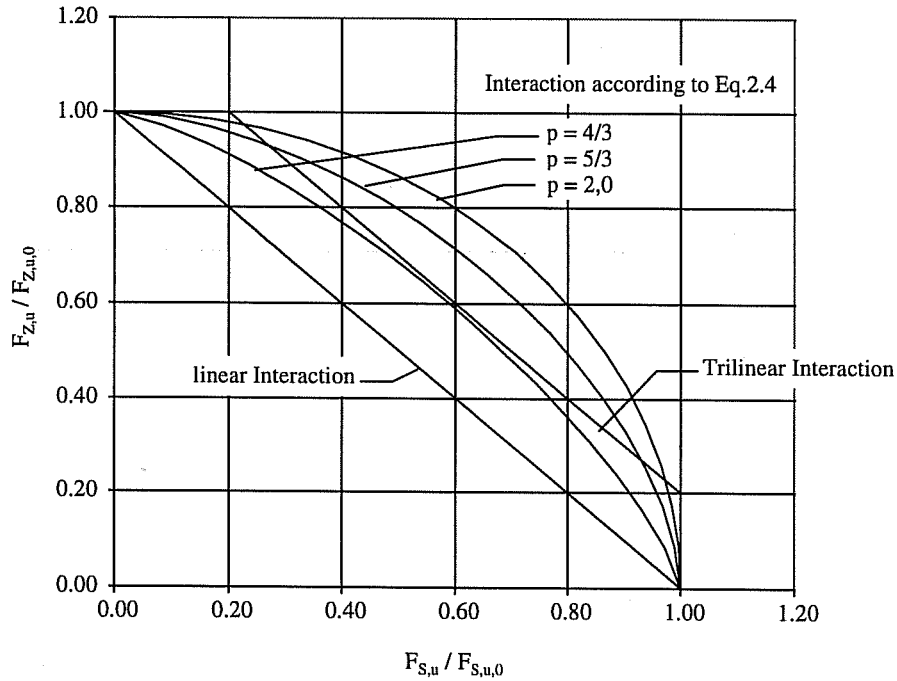
Figure 2.1 Tension and shear interaction for anchors at ultimate capacity
