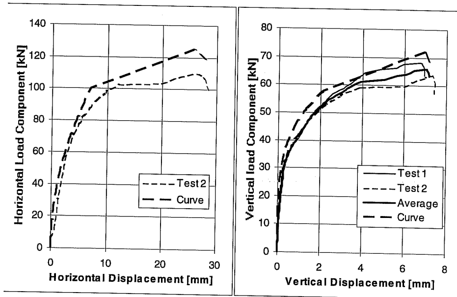
Load-Displacement Curves of Series 23m746. UC1 Anchor 5/8 inches, hef = 7 inches (178 mm), c1 3 11 inches (279 mm). f c = 32.4 N/mm 2 . Loading Angle 60° from Anchor Axis Through-Sleeve Installation
