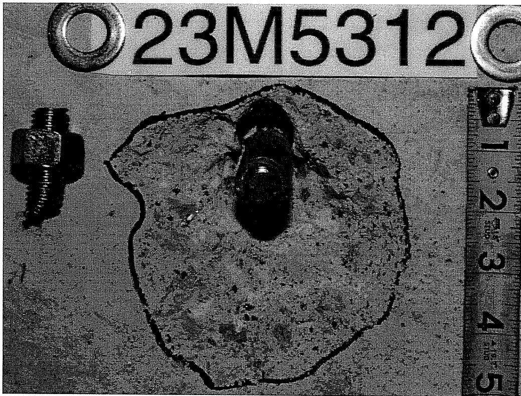
Failure Picture of Test 23M5312, UC1 5/8", Oblique Tension 15°
