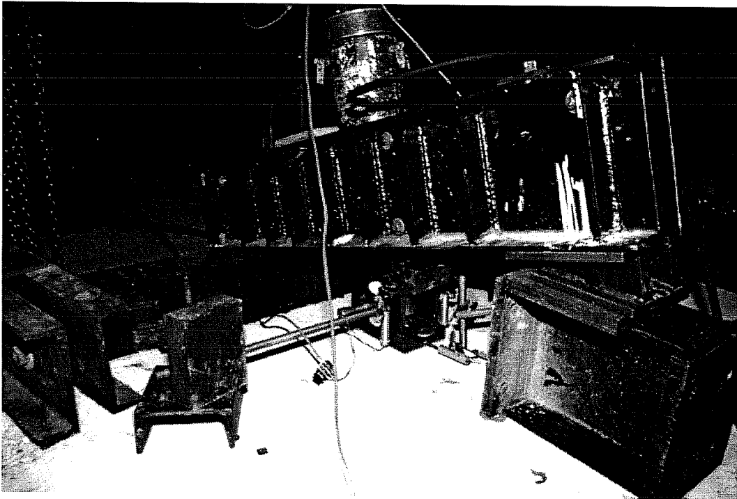
Test Setup of Series 2.4, Oblique Tension Tests at 15° with Concrete Failure Breakout
