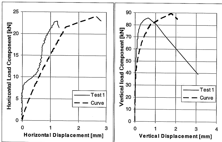
Load-Displacement Curves of Series 24a541. UC1 5/8 inches, h_{ef} = 3.5 inches (178 mm), c_1 \geq 11 inches (279 mm). f_c = 32.4 N/mm 2 , Loading Angle 15° from Anchor Axis
