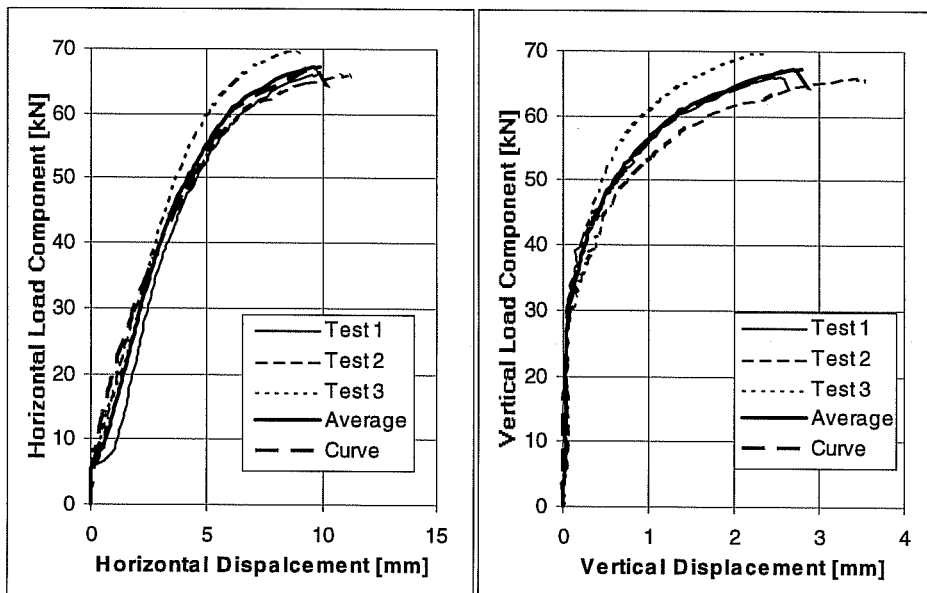
Load-Displacement Curves of Series 23m534, UC1 Anchors 5/8 inches, hef = 7 inches (178 mm), c1 3 11 inches (279 mm), f c = 20.7 N/mm 2 , Loading Angle 45° from Anchor Axis
