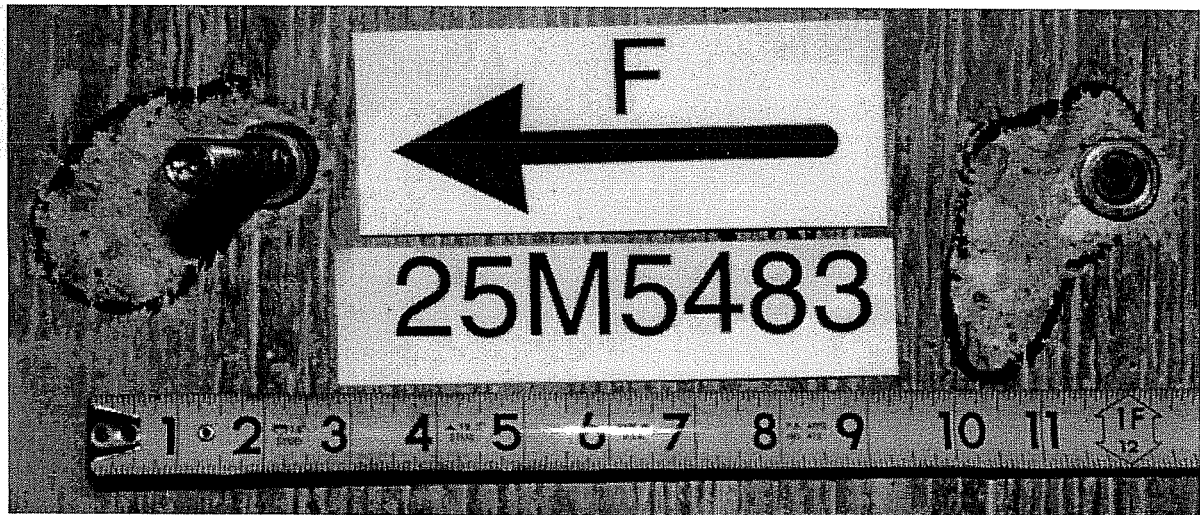
Failure Picture of Test 25M5483 (Failure of Tension Anchor), UC1 5/8", h_{ef} = 7 inches (178 mm), e = 18 inches (457.2 mm)
