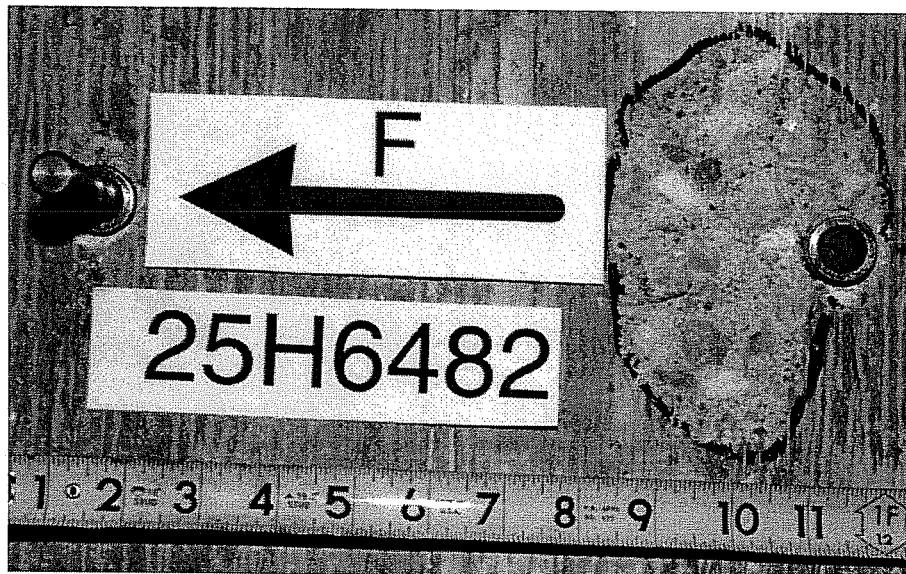
Failure Picture of Test 25H6482 (Failure of Tension Anchor), Sleeve M16, h_{ef} = 7 inches (178 mm), e = 18 inches (457.2 mm)
