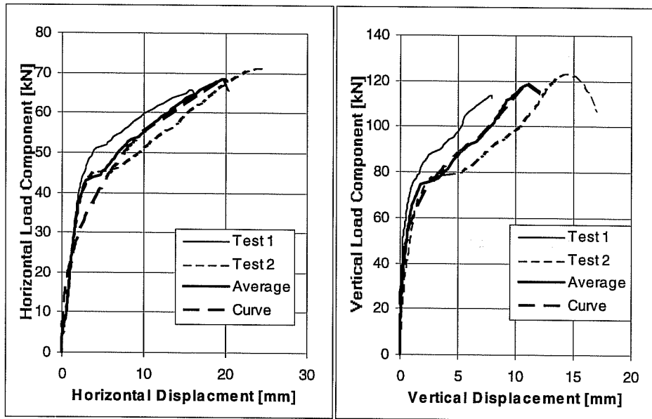
Load-Displacement Curves of Series 23h743, Sleeve Anchors M16, h_{ef} = 7 inches (178 mm) c_1 \geq 11 inches (279 mm), f_c = 32.4 N/mm 2 , Loading Angle 30° from Anchor Axis Through-Sleeve Installation
