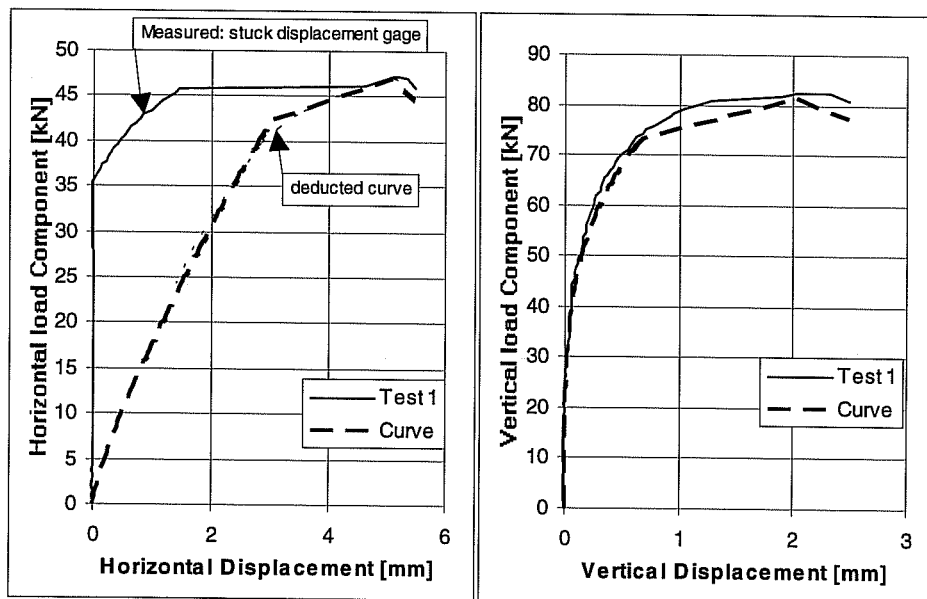
Load-Displacement Curves of Series 24a543, UC1 5/8 inches, hef = 3.5 inches (178 mm), c1 3 11 inches (279 mm), f c = 32.4 N/mm 2 , Loading Angle 30° from Anchor Axis
