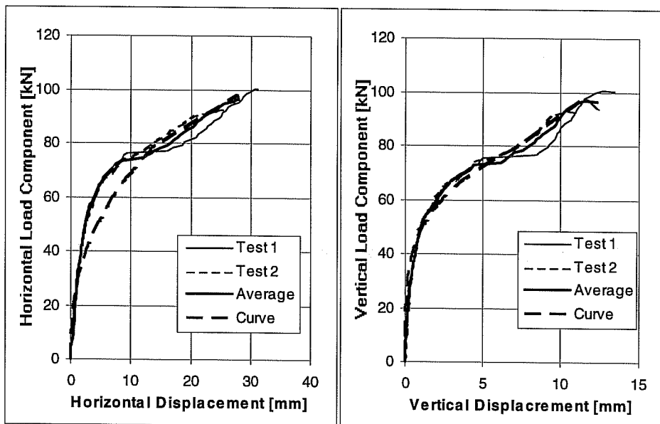
Load-Displacement Curves of Series 23h744, Sleeve Anchors M16, h_{set} = 7 inches (178 mm) c_1 \geq 11 inches (279 mm), f_c = 32.4 N/mm 2 , Loading Angle 45° from Anchor Axis Through-Sleeve Installation
