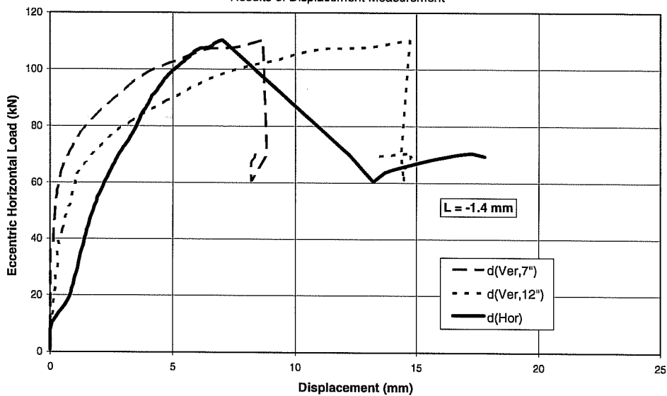
Test 25M5422, UC1 5/8", e = 12 inches (304.8 mm) Steel Failure of Shear Anchor - Results of Displacement Measurement -
