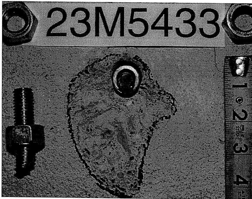
Failure Picture of Test 23M5433, UC1 5/8", Oblique Tension 30°
