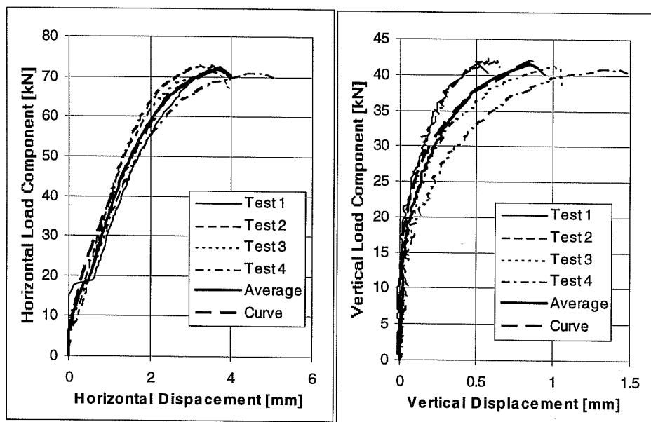
Load-Displacement Curves of Series 23h646. Sleeve M16, h_{ef} = 7 inches (178 mm), c_1 \geq 11 inches (279 mm), f_c = 32.4 N/mm 2 , Loading Angle 60° from Anchor Axis
