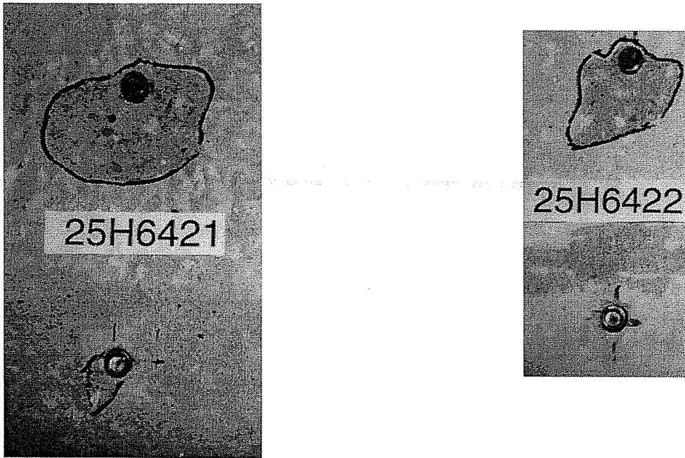
Failure Picture of Test 25H6421 (Both Anchors Failed Together) and 25H6422 (Shear Anchor Failed First), Sleeve M16, h_{ef} = 7 inches (178 mm), e = 12 inches (304.8 mm)
