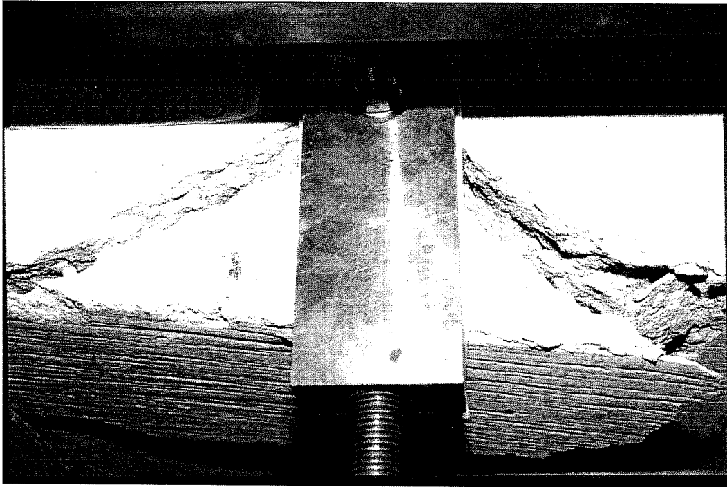
Failure Picture of Test 24M54S1, UC1 5/8", h_{ef} = 89 mm, c1 = 140 mm, Shear
