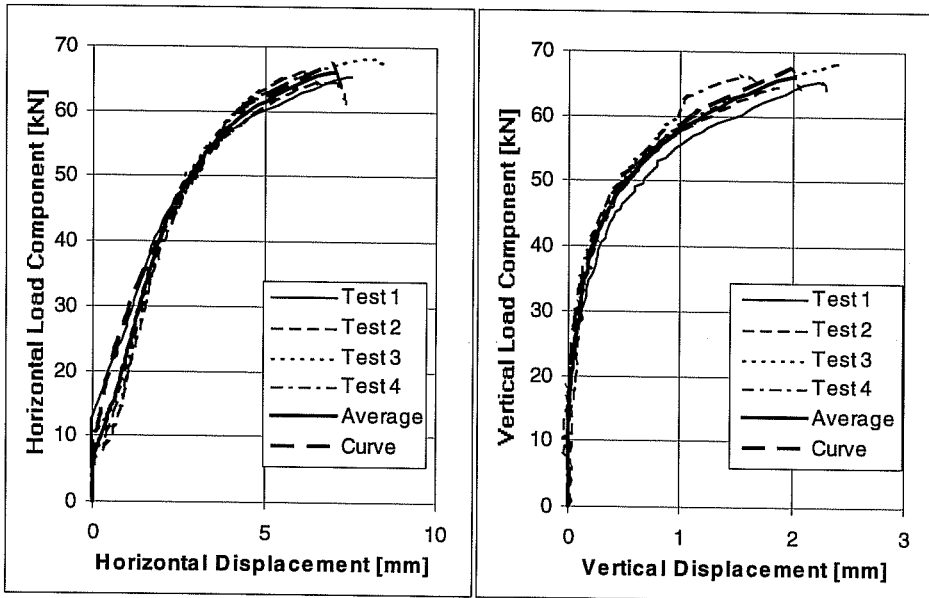
Load-Displacement Curves of Series 23m544, UC1 Anchors 5/8 inches, h_{ef} = 7 inches (178 mm), c_1 \approx 11 inches (279 mm), f_c = 32.4 N/mm 2 , Loading Angle 45° from Anchor Axis
