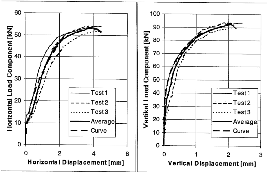
Load-Displacement Curves of Series 23h643. Sleeve M16, h_{ef} = 7 inches (178 mm), c_1 \geq 11 inches (279 mm). f_c = 32.4 N/mm 2 , Loading Angle 30° from Anchor Axis
