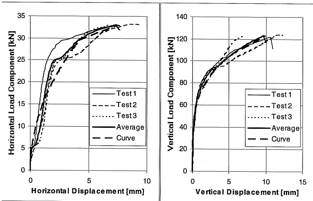
Load-Displacement Curves of Series 23h641. Sleeve M16, h_{ef} = 7 inches (178 mm), a_r \geq 11 inches (279 mm), f_c = 32.4 N/mm 2 , Loading Angle 15° from Anchor Axis
