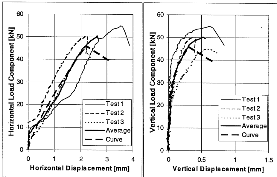
Load-Displacement Curves of Series 24m544, UC1 5/8 inches, hef = 3.5 inches (89 mm), c1 = 5.5 inches (140 mm), f_c = 32.4 \text{ N/mm}^2 , Loading Angle 45° from Anchor Axis
