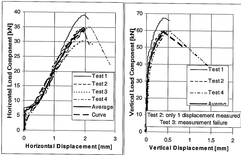
Load-Displacement Curves of Series 24m543. UC1 Anchors 5/8 inches, h_{ef} = 3.5 inches (89 mm), c_1 = 5.5 inches (140 mm), f_c = 32.4 N/mm 2 , Loading Angle 30° from Anchor Axis
