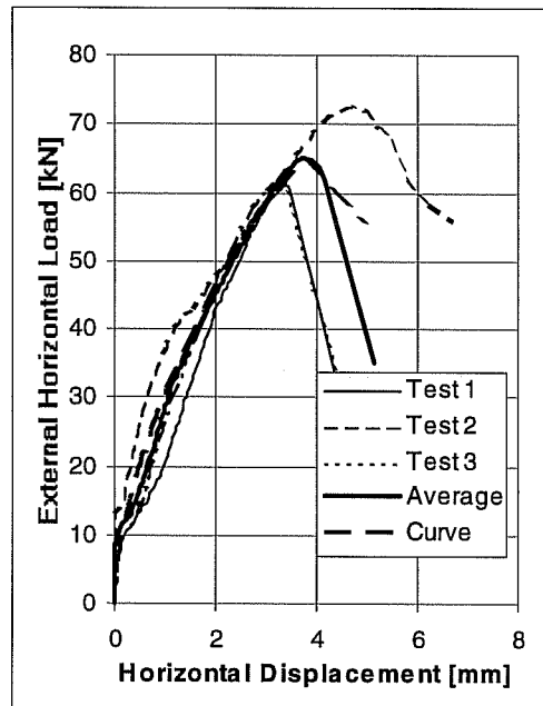
Load-Displacement Curves of Series 24m54T (Tension) and 24m54S (Shear) UC1 Anchors 5/8 inches, hef = 3.5 inches (89 mm), c1 = 5.5 inches (140 mm), fc = 32.4 N/mm 2
