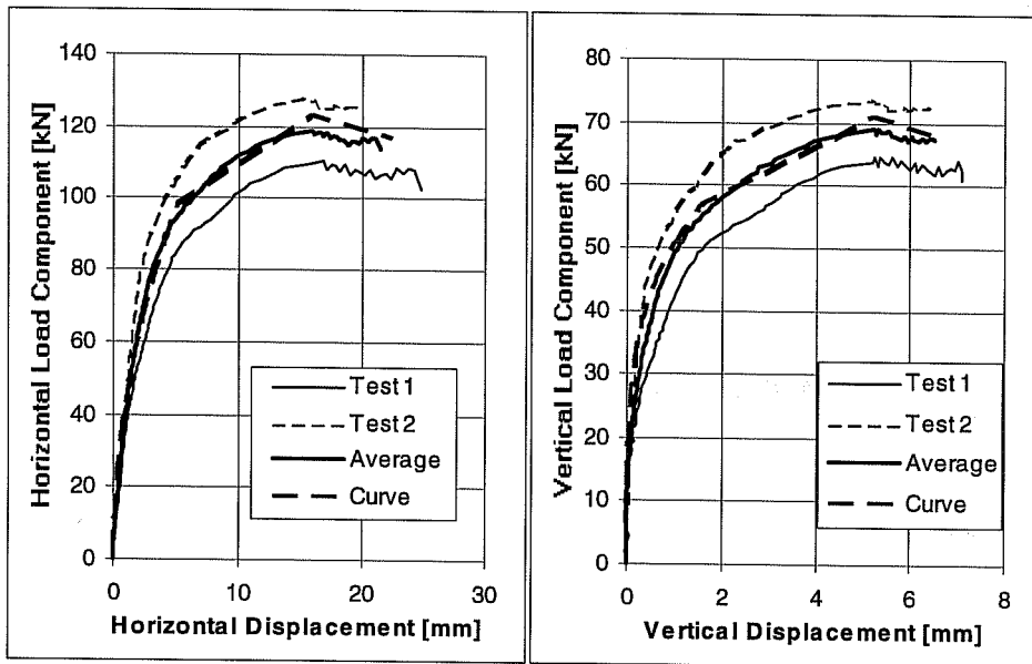
Load-Displacement Curves of Series 23h746, Sleeve Anchors M16, h_{ef} = 7 inches (178 mm) c_1 \geq 11 inches (279 mm), f_c = 32.4 N/mm 2 , Loading Angle 60° from Anchor Axis Through-Sleeve Installation
