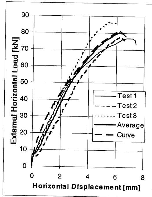
Load-Displacement Curves of Series 23m53T (Tension) and 23m53S (Shear) UC1 Anchors 5/8 inches, hef = 7 inches (178 mm), c1 = 11 inches (279 mm), fc = 20.7 N/mm 2
