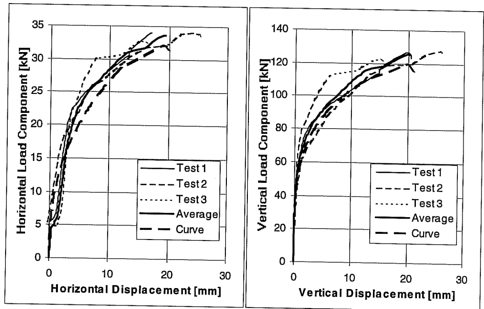
Load-Displacement Curves of Series 23m531, UC1 Anchors 5/8 inches, h_{ef} = 7 inches (178 mm), c_1 \geq 11 inches (279 mm), f_c = 20.7 \text{ N/mm}^2 , Loading Angle 15^\circ from Anchor Axis
