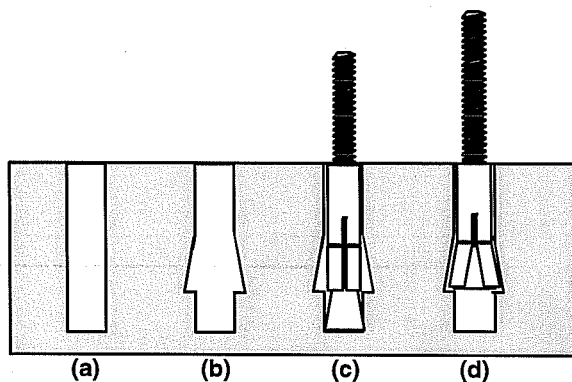
Figure 3.5 Installation Sequence for Undercut Anchors: (a) drill cylindrical hole; b) undercut; c) place anchor in hole; and d) expand anchor
