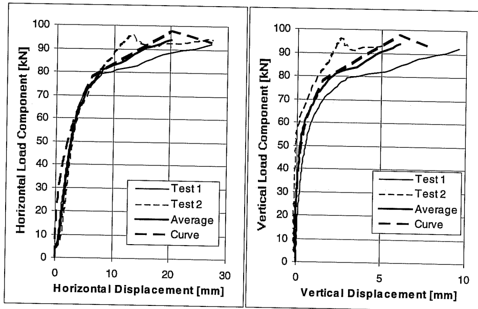
Load-Displacement Curves of Series 23m744. UC1 Anchor 5/8 inches, h_{ef} = 7 inches (178 mm), c_1 \geq 11 inches (279 mm). f_c = 32.4 \text{ N/mm}^2 , Loading Angle 45^\circ from Anchor Axis Through-Sleeve Installation
