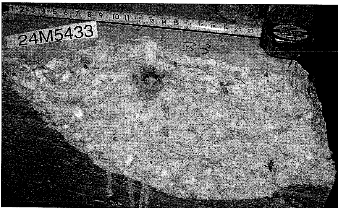
Failure Picture of Test 24M5433, UC1 5/8", h_{ef} = 89 mm, c1 = 140 mm, Oblique Tension 30^\circ
