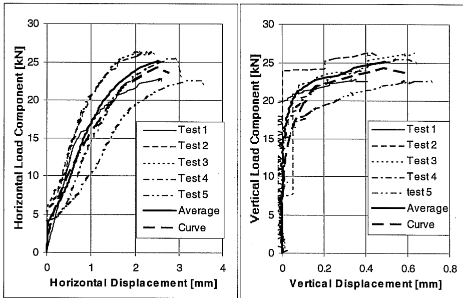
Load-Displacement Curves of Series 23m344. UC1 Anchors 3/8 inches, hef = 7 inches (178 mm), c1 3 11 inches (279 mm). f_c = 32.4 \text{ N/mm}^2 . Loading Angle 45° from Anchor Axis
