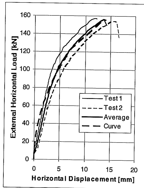
Load-Displacement Curves of Series 23m54T (Tension) and 23m74S (Shear) UC1 Anchor 5/8 inches, h_{ef} = 7 inches (178 mm), c_1 \geq 11 inches (279 mm), f_c = 32.4 N/mm 2 Shear with Through-Sleeve Installation
