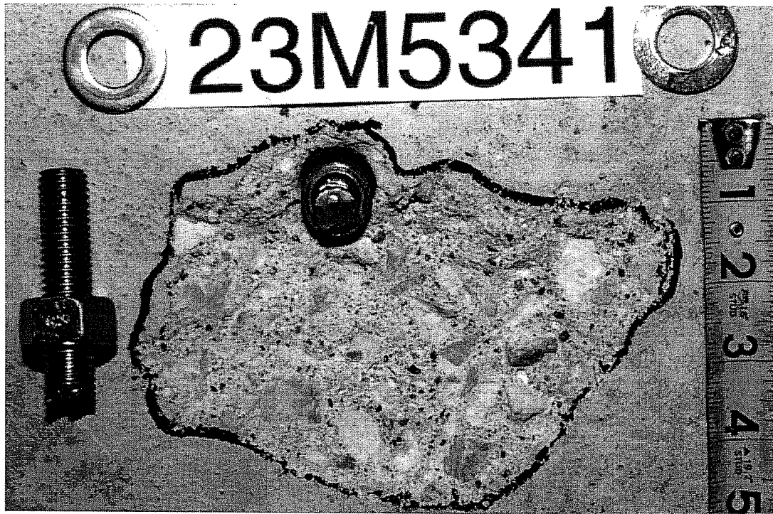
Failure Picture of Test 23M5341, UC1 5/8", Oblique Tension 45°
