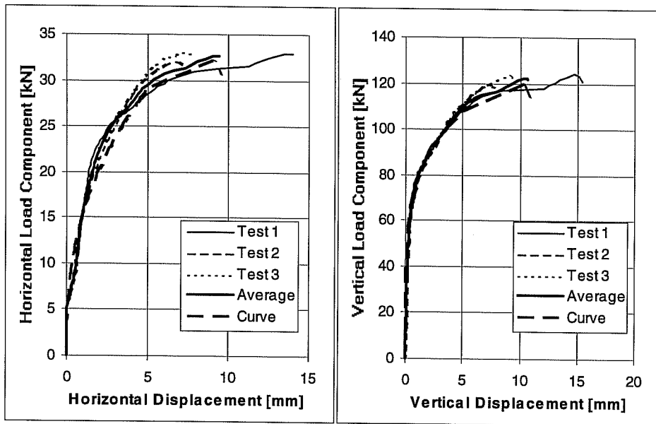
Load-Displacement Curves of Series 23m541. UC1 Anchor 5/8", h_{ef} = 7 inches (178 mm), c_1 \geq 11 inches (279 mm). f_u = 32.4 N/mm 2 , Loading Angle 15° from Anchor Axis
