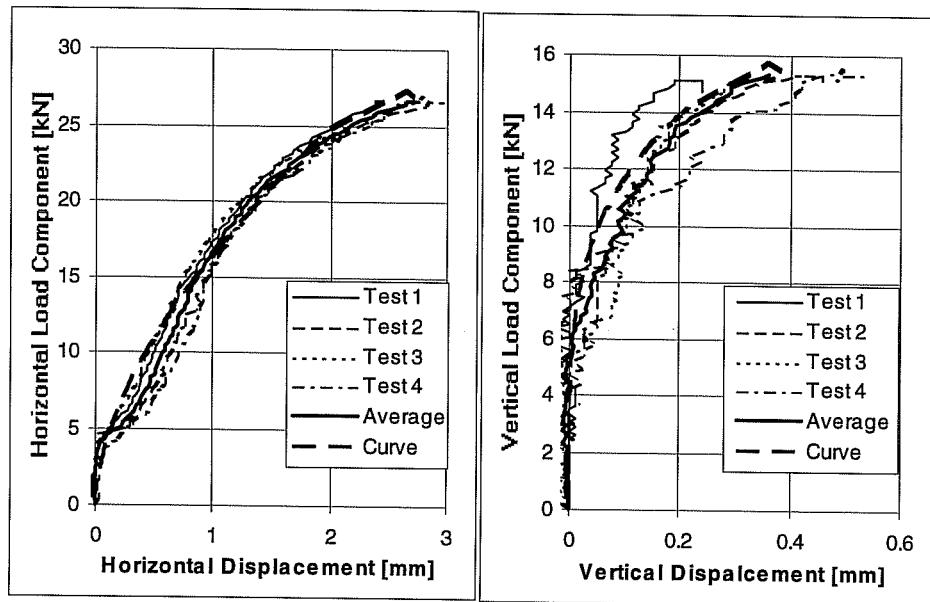
Load-Displacement Curves of Series 23m346, UC1 Anchors 3/8 inches, hef = 7 inches (178 mm), c1 3 11 inches (279 mm), f c = 32.4 N/mm 2 , Loading Angle 60° from Anchor Axis
