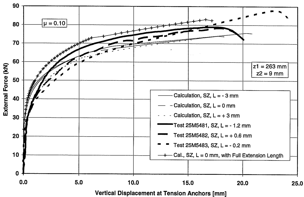
Vertical Displacement at Tension Anchors in Calculation and Tests
