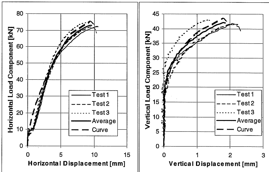
Load-Displacement Curves of Series 23m536. UC1 Anchors 5/8 inches, hef = 7 inches (178 mm), c1 3 11 inches (279 mm). f c = 20.7 N/mm 2 , Loading Angle 60° from Anchor Axis
