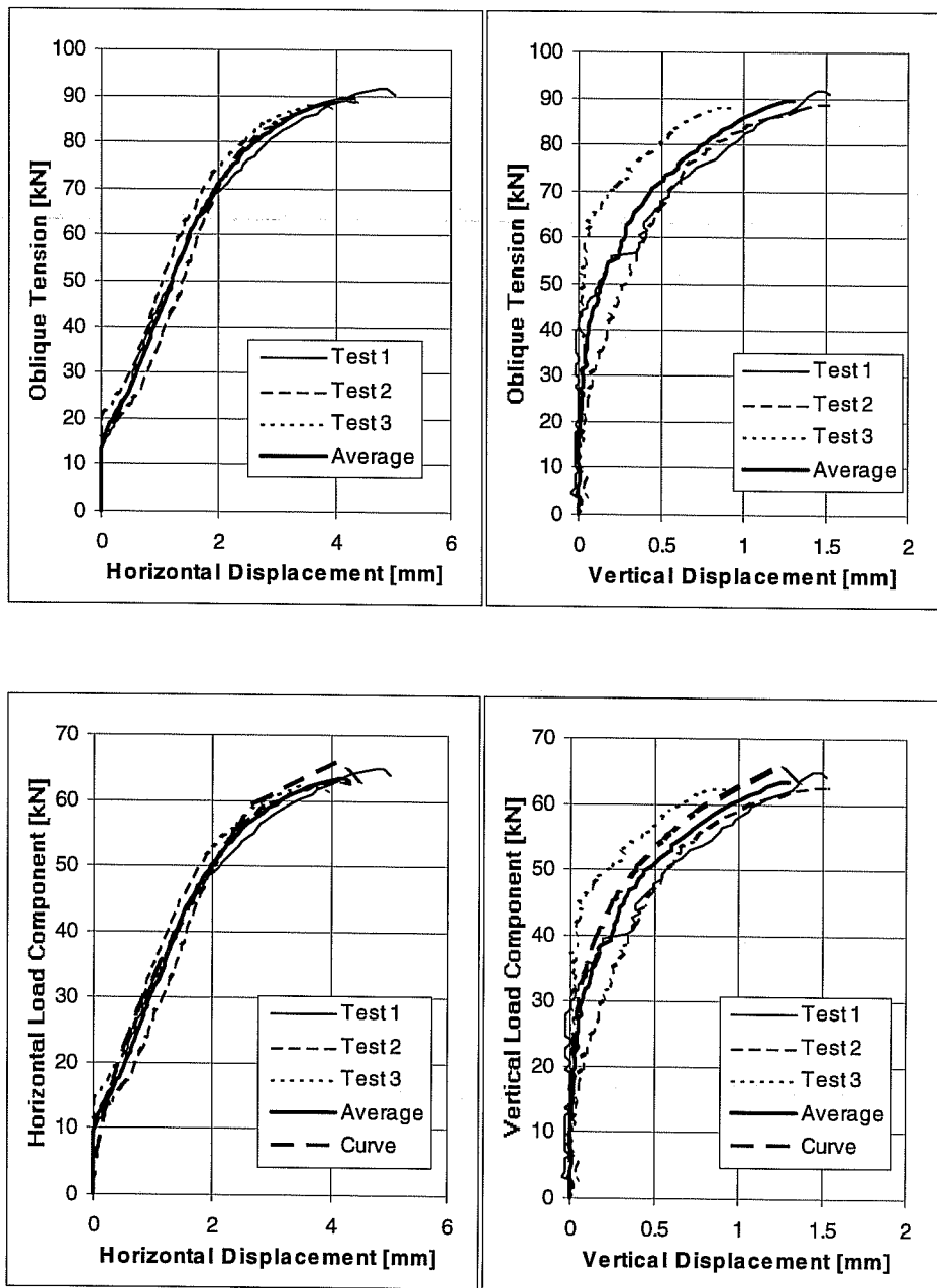
Load-Displacement Curves of Series 23h644. Sleeve M16, h_{ef} = 7 inches (178 mm), c_1 \geq 11 inches (279 mm). f_e = 32.4 N/mm 2 , Loading Angle 45° from Anchor Axis
