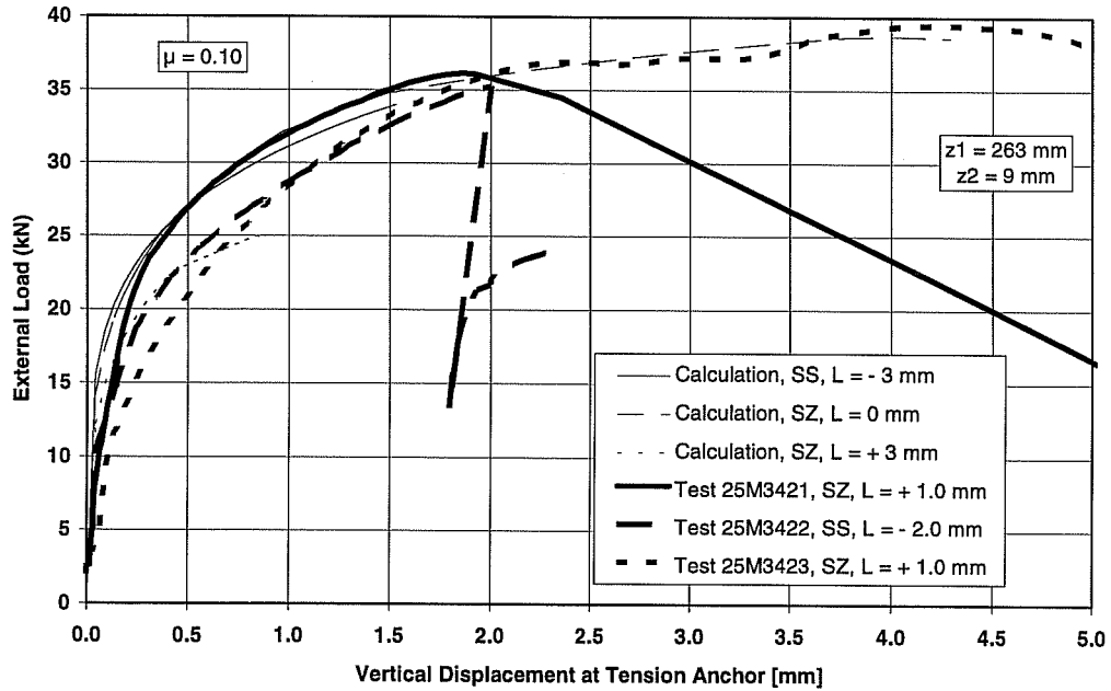
Vertical Displacement at Tension Anchor in Calculation and Test
