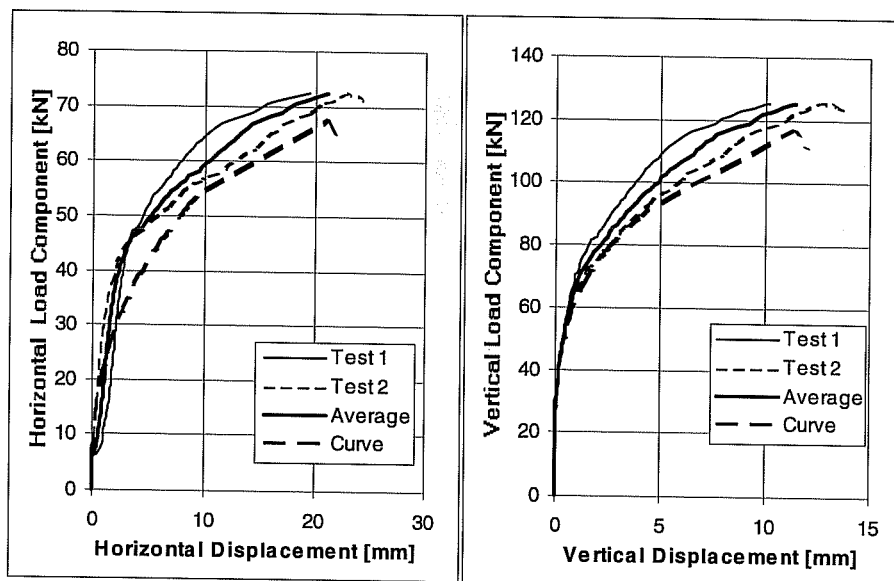
Load-Displacement Curves of Series 23m743. UC1 Anchor 5/8 inches, hef = 7 inches (178 mm), c1 = 11 inches (279 mm), fc = 32.4 N/mm 2 , Loading Angle 30° from Anchor Axis Through-Sleeve Installation
