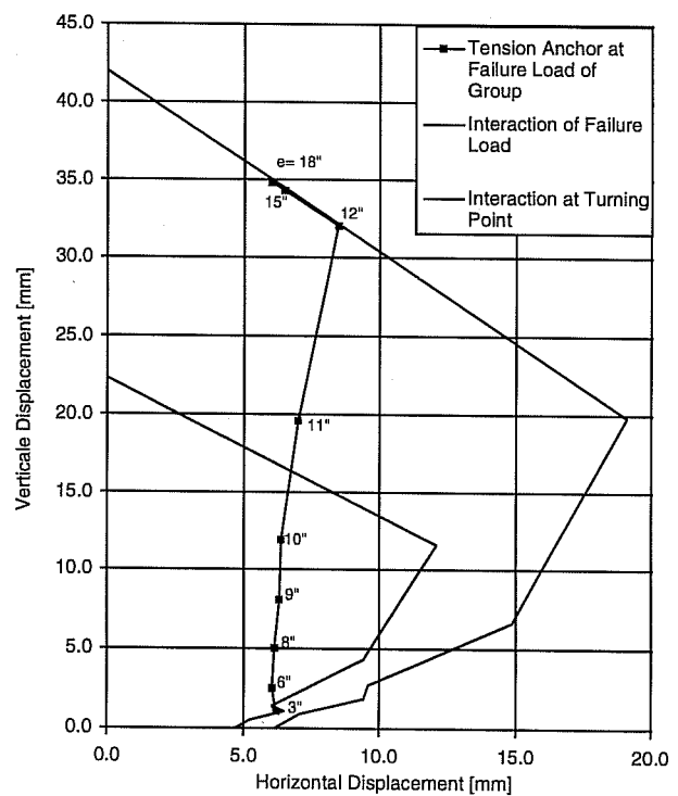
Figure 4.10 Deformation state of the tension anchor at maximum load of the group, plotted on the displacement interaction diagram
