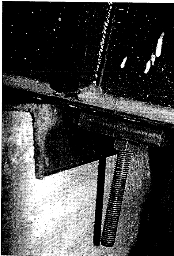
Bearing Support of Series 2.3, Oblique Tension Tests at 15° with Steel Failure
