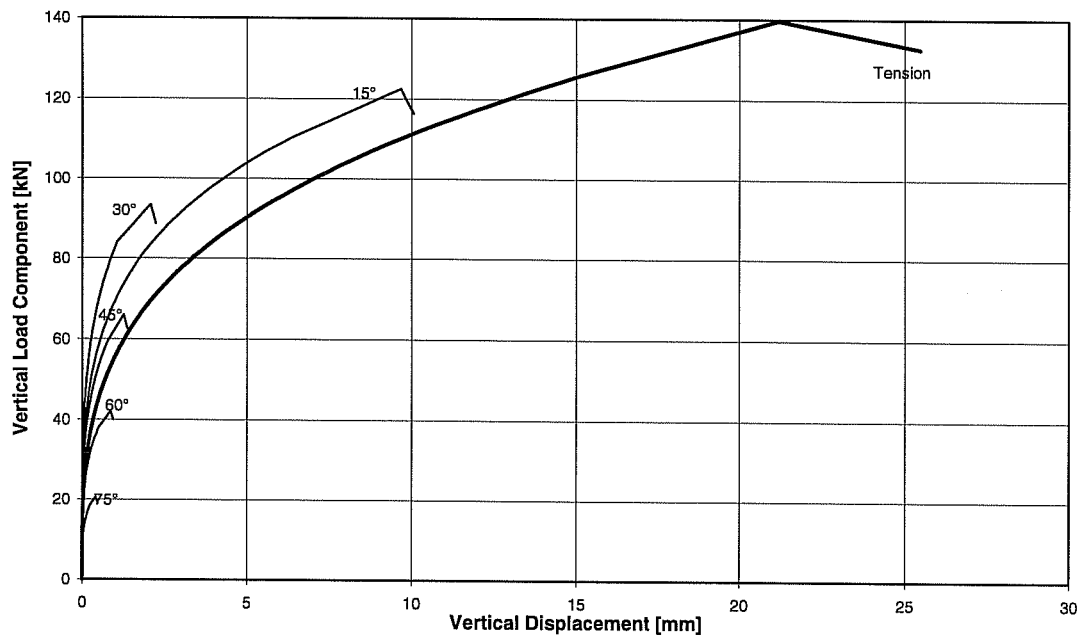
Mathematical Description of Load-Displacement Curves of Series 23H64
