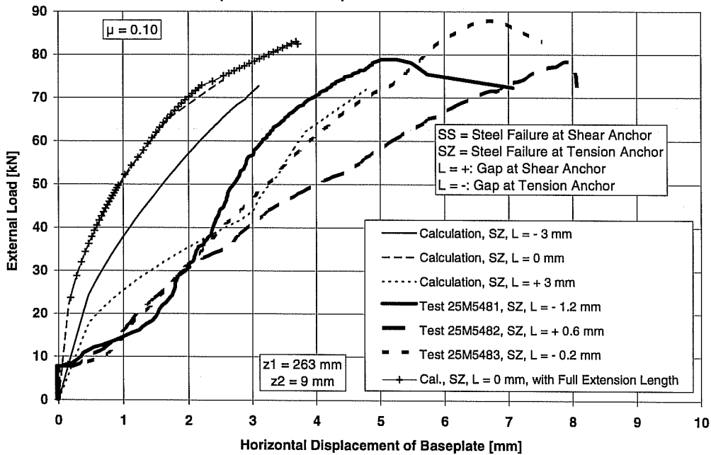
Series 25M548, UC1 5/8", e = 18 inches (457.2 mm), f_c = 32.4 \text{ N/mm}^2 Horizontal Displacement of Baseplate in Calculation and Test
