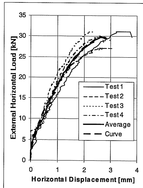
Load-Displacement Curves of Series 23m34T (Tension) and 23m34S (Shear) UC1 Anchors 5/8 inches, hef = 7 inches (178 mm), c1 3 11 inches (279 mm), fc = 32.4 N/mm 2
