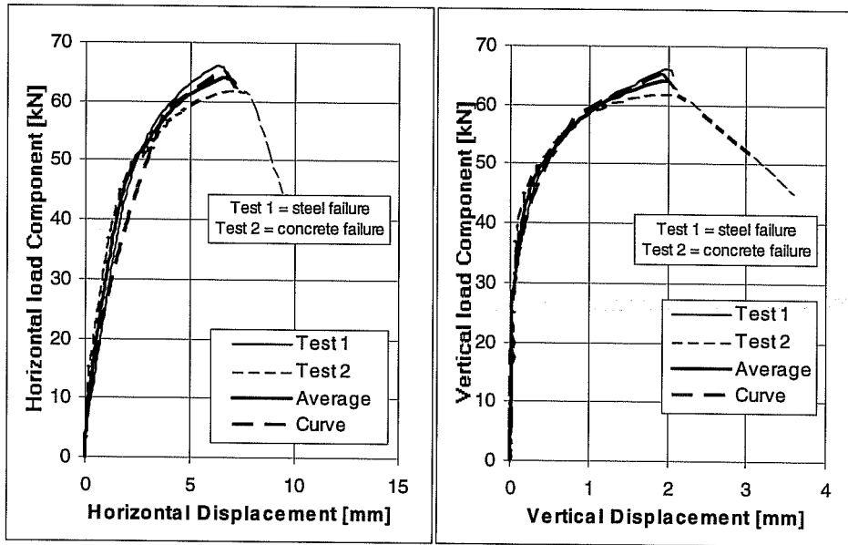
Load-Displacement Curves of Series 24a544. UnUC1 5/8 inches, h_{ef} = 3.5 inches (89 mm), c_1 \approx 11 inches (279 mm), f_c = 32.4 N/mm 2 , Loading Angle 45° from Anchor Axis
