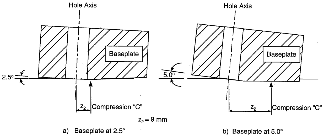
Figure 4.1 Location of the resultant compression between the baseplate and the concrete
