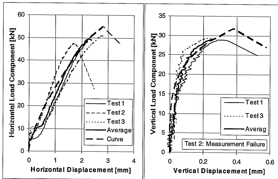
Load-Displacement Curves of Series 24m546. UC1 5/8 inches, h_{ef} = 3.5 inches (89 mm), c_1 = 5.5 inches (140 mm). f_c = 32.4 N/mm 2 , Loading Angle 60° from Anchor Axis
