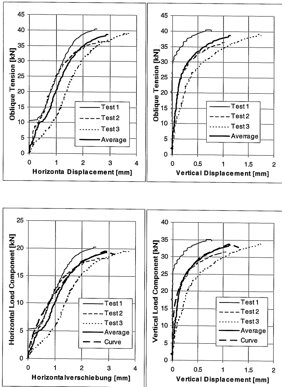
Load-Displacement Curves of Series 23m343. UC1 3/8 inches, hef = 7 inches (178 mm), c1 = 11 inches (279 mm). f_c = 32.4 \text{ N/mm}^2 , Loading Angle 30° from Anchor Axis
