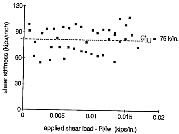
Figure 4.2 Comparison of initial cycle stiffness to incremental stiffnesses.
