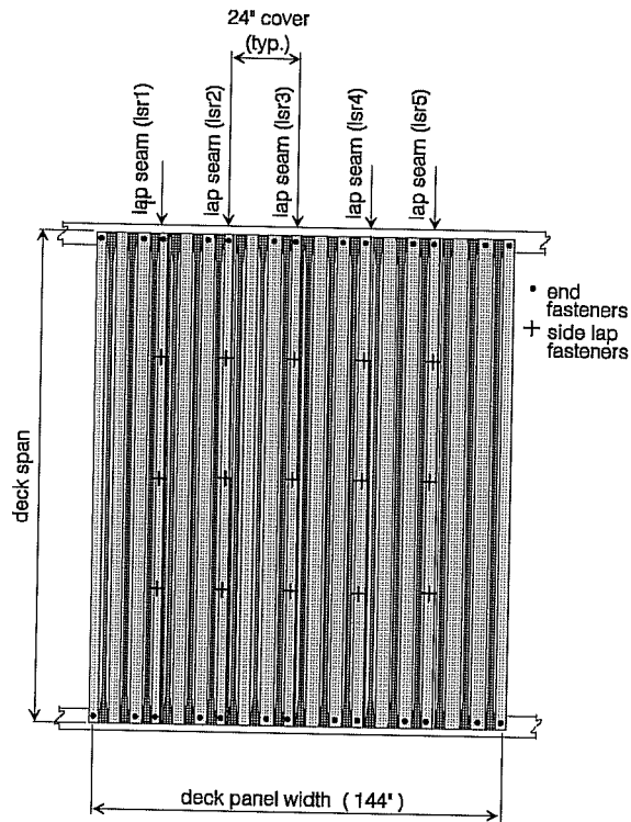
Figure 4.14 Twelve-ft. wide panel with standard end and side lap fasteners.
