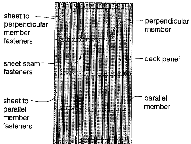
Figure 1.4 Attachment of deck panel to supporting structure.
