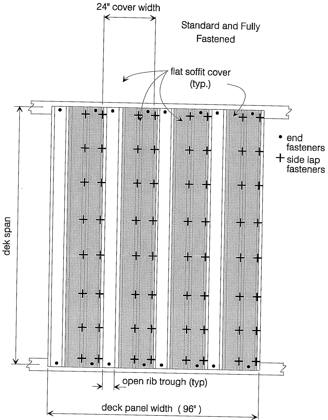
Figure 4.9 Fastener configurations - deck types LSM1524, LSM1724, and LSM 2224.
