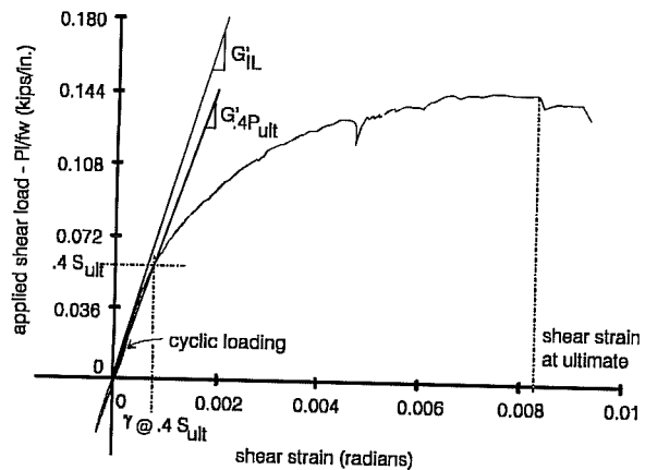
Figure 4.4 Shear load vs. shear strain - all loaded cycles.
