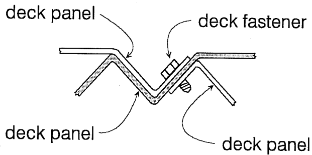
Figure 2.8 Side lap fastener arrangement for flat soffit decks.
