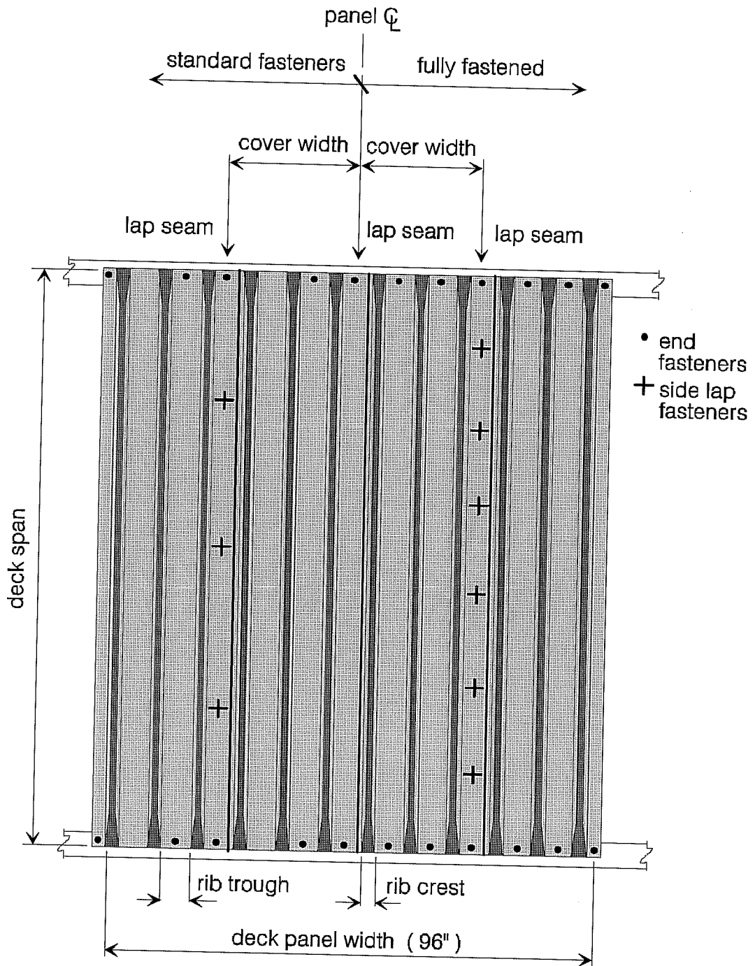
Figure 4.8 Fastener configuration - deck type BOS816.
