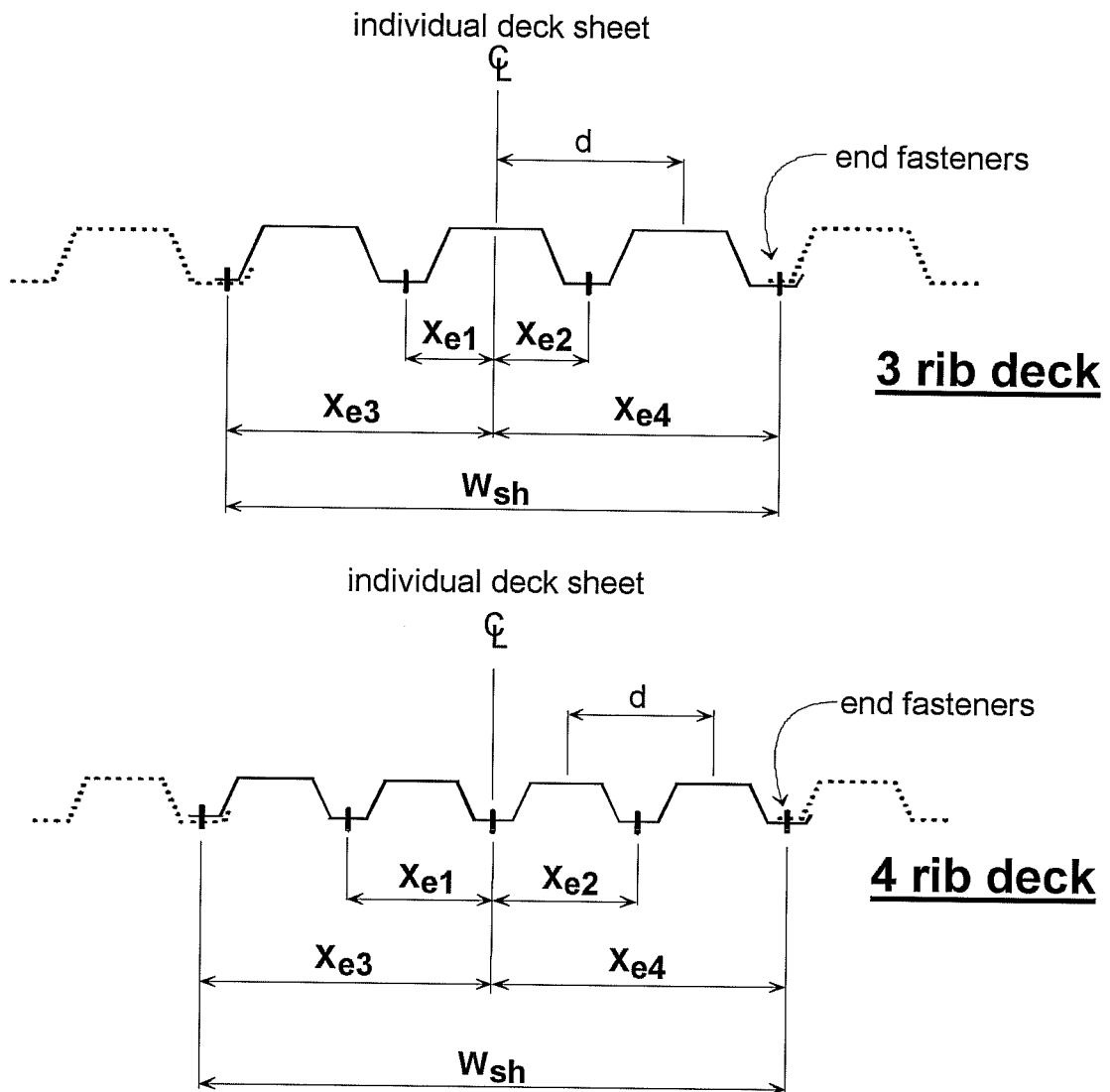
Figure A.1 Open profile diaphragm geometries.
