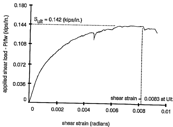
Figure 4.5 Shear load vs. shear strain - ultimate cycle.
