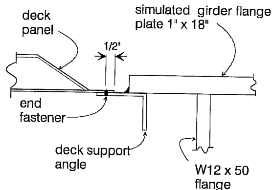
Figure 3.6 Rigid connection of deck support angle to simulated girder flange.
