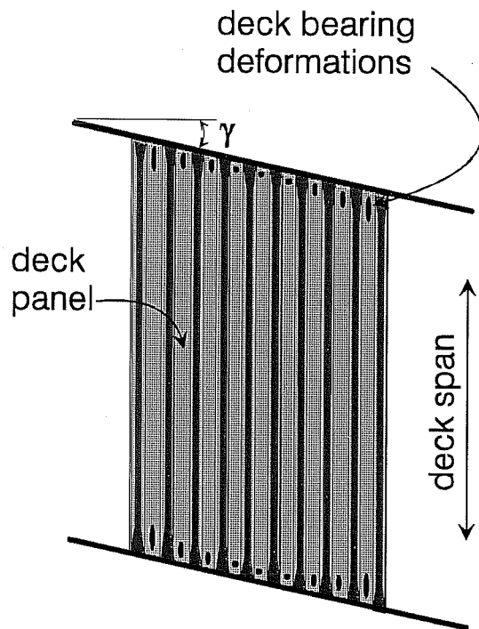
Figure 1.7 End fastener deck bearing deformations - parallel to span.
