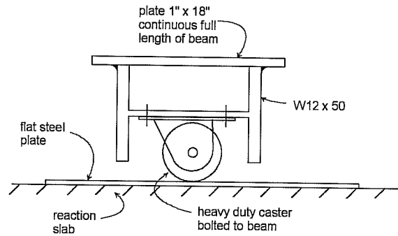
Figure 3.2 Cross section through deck support beams.
