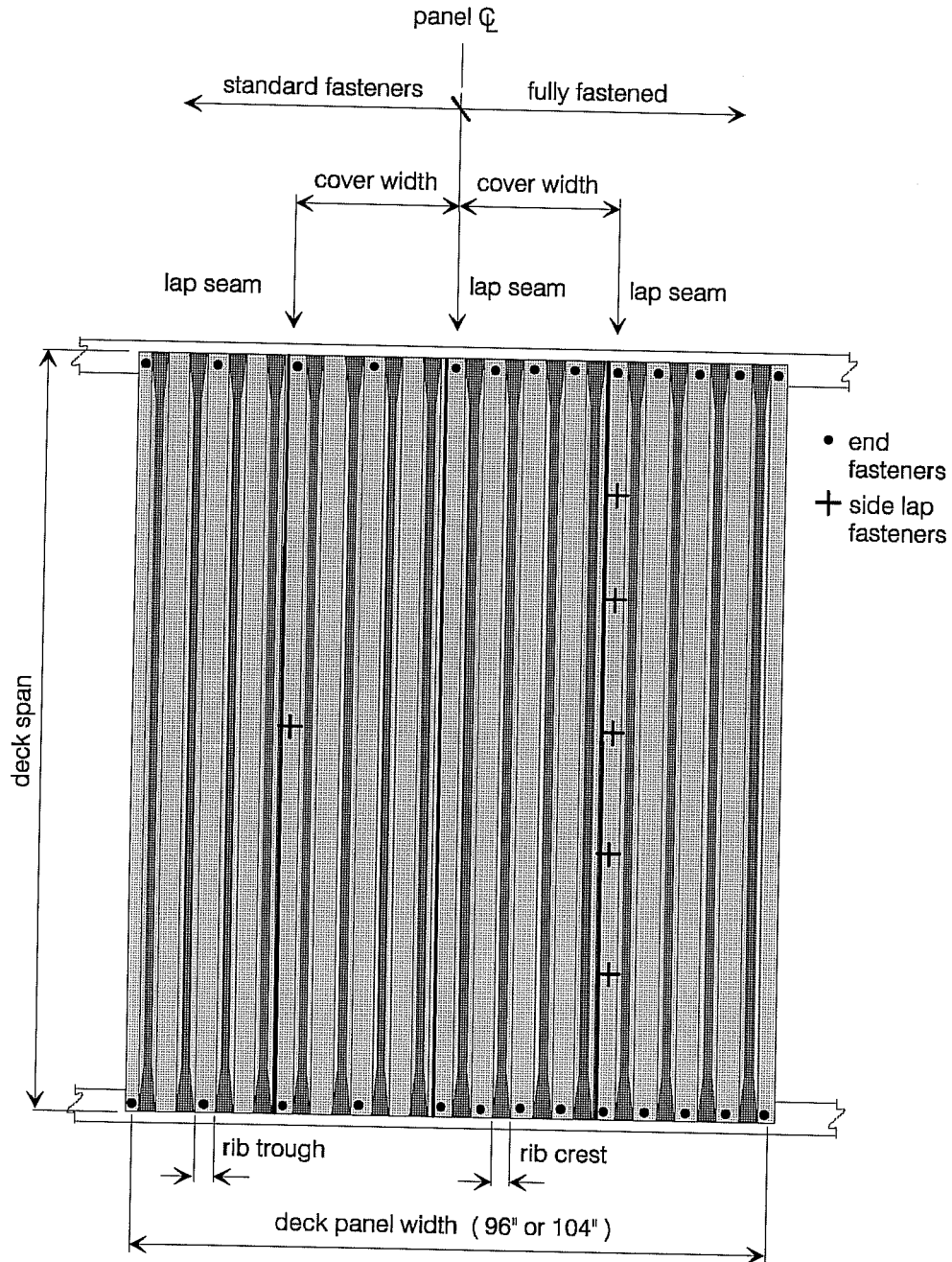
Figure 4.6 Fastener configurations - deck types BUBF18, BUBf16, and BUBF14.
