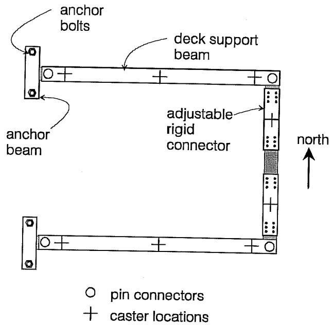
Figure 3.1 Plan of test frame.
