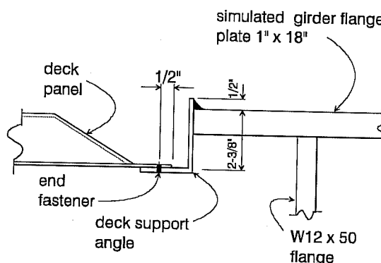
Figure 3.7 Welded eccentric connection of deck support angle to simulated girder flange.
