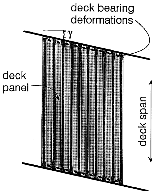
Figure 1.8 End fastener deck bearing deformations - perpendicular to span.
