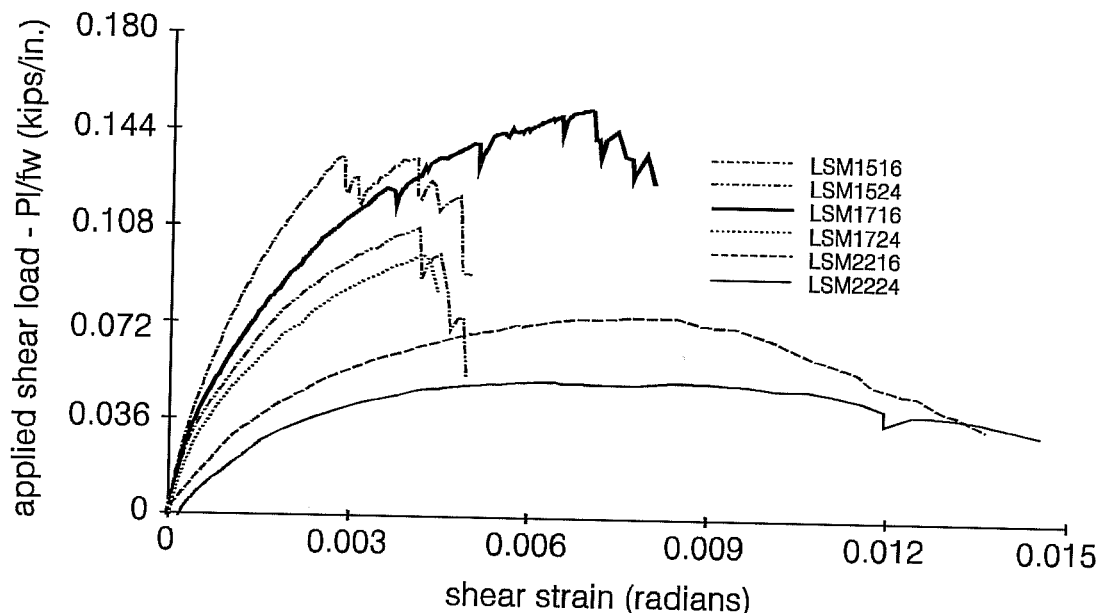
Figure 4.12 Shear load vs. shear strain - ultimate cycles for flat soffit profile decks.
