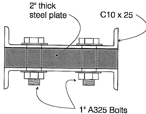
Figure 3.3 Cross section through adjustable connector strap.
