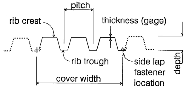
Figure 2.1 Typical open profile deck.
