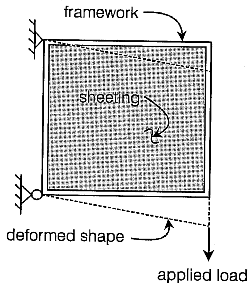
Figure 1.1 Fundamental shear diaphragm.
