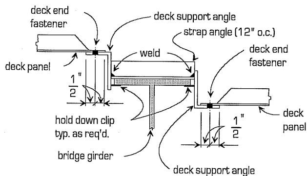
Figure 1.10 Deck support angles - welding to girders not permitted.
