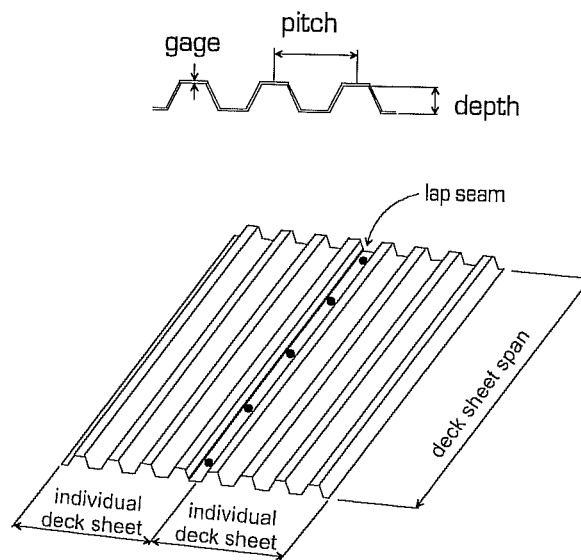
Figure 1.2 Typical steel deck sheeting layout and profile.
