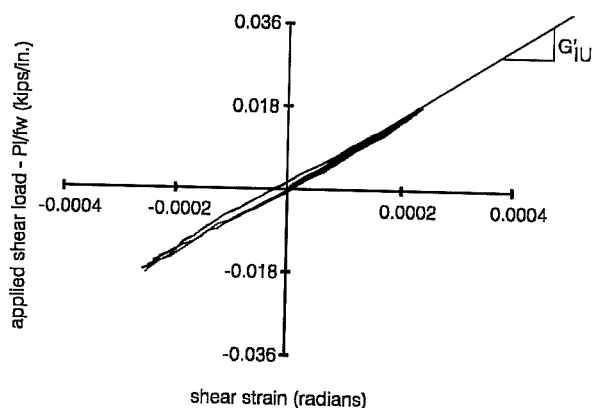
Figure 4.1 Shear load vs. shear strain - all unloaded cycles.
