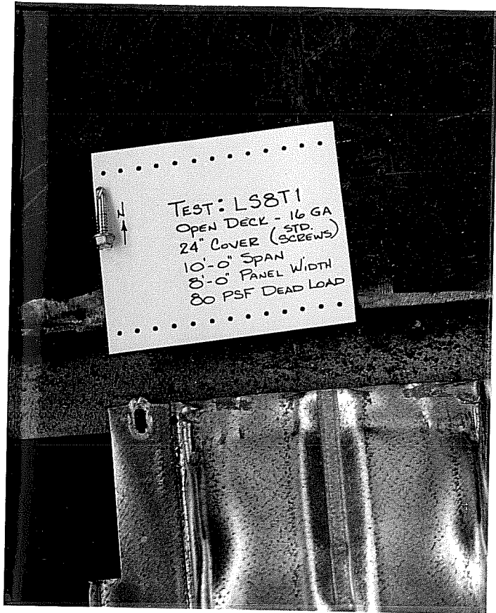
Figure 4.16 Tear-out of deck material at fastener location.
