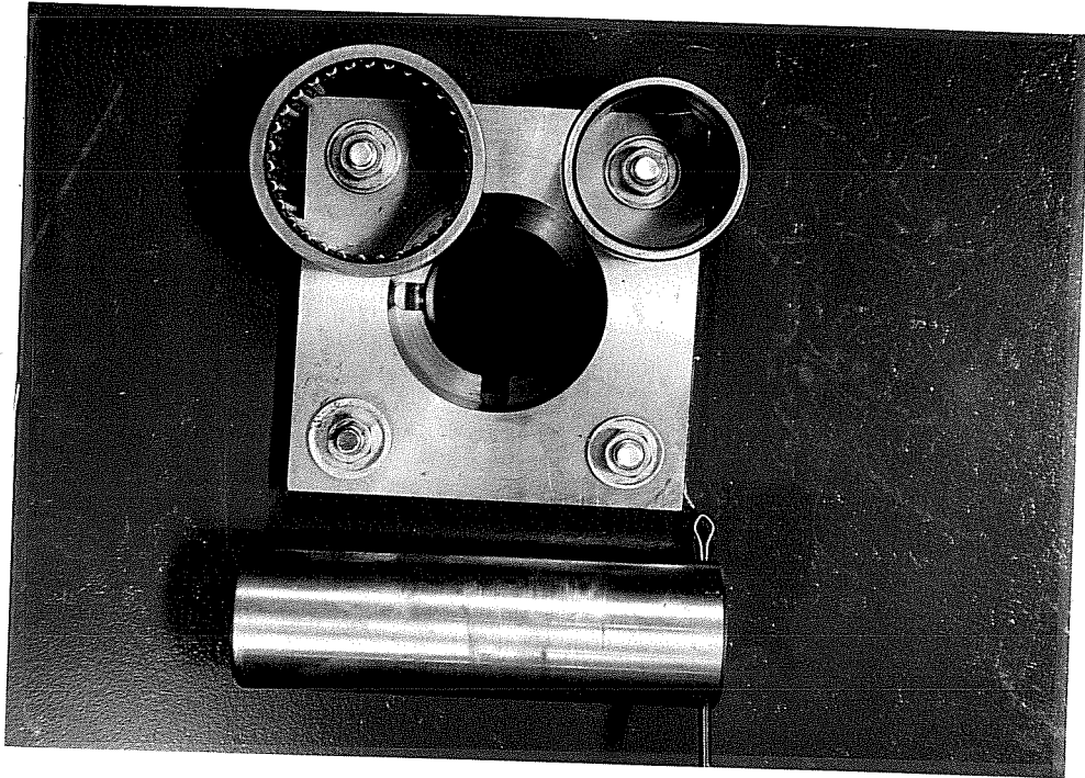
Figure 3.4 Blow-up of pin and bearing assembly.
