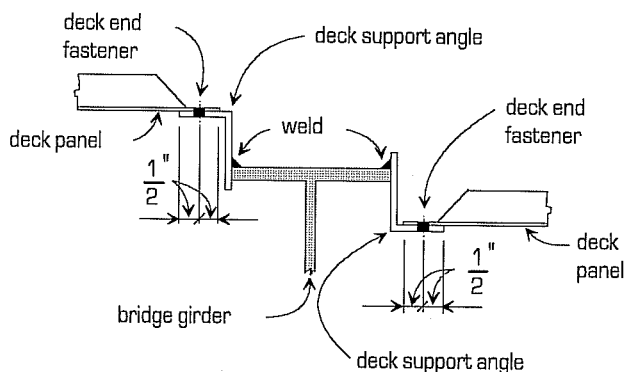
Figure 1.9 Deck support angles - welded to girders.
