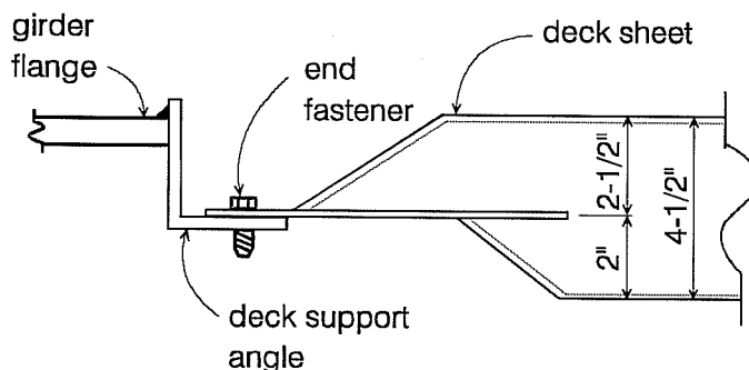
Figure 2.6 Flat soffit deck with 16" coverage.
