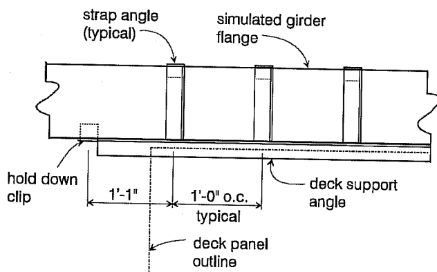
Figure 3.8 Plan of strap angles and deck support angle for non-welded connection.
