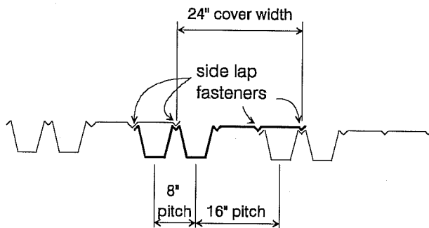
Figure 2.5 Flat soffit deck with 24" coverage.
