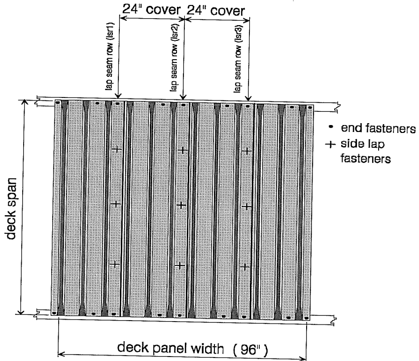
Figure 4.13 Eight-ft. wide panel with standard end and side lap fasteners.
