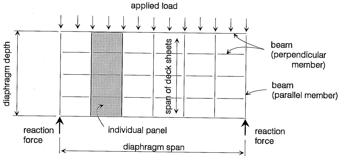
Figure 1.3 Relationship of sheeting arrangement to structural components.
