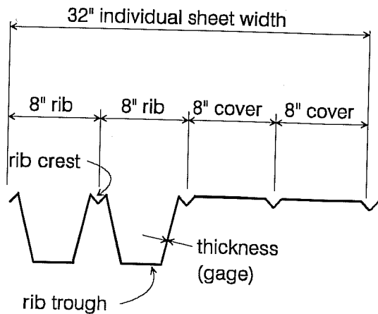
Figure 2.4 Typical flat soffit deck.
