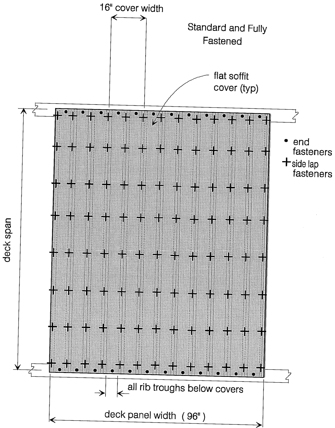
Figure 4.10 Fastener configurations - deck types LSM1516, LSM1716 and LSM2216.
