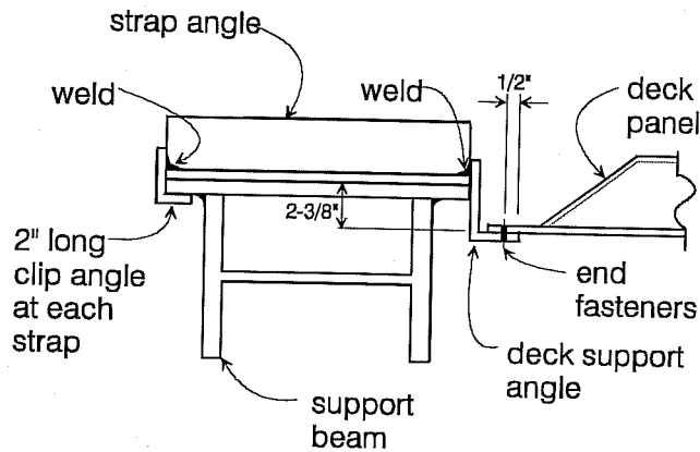
Figure 3.9 Non-welded eccentric connection of deck support angle to simulated girder flange.
