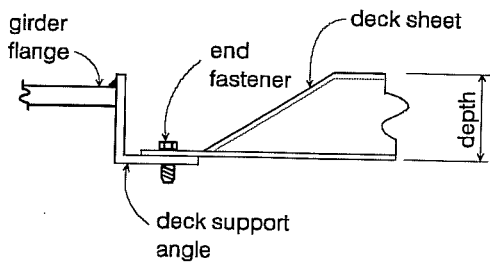
Figure 2.3 Support condition of open profile deck.
