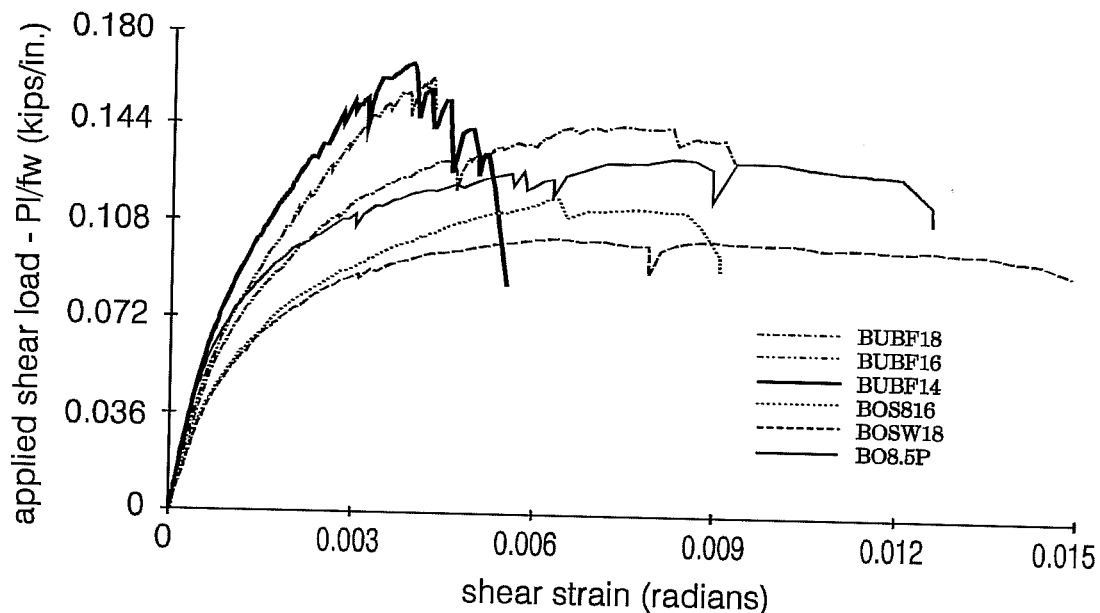
Figure 4.11 Shear load vs. shear strain - ultimate cycles for open profile decks.
