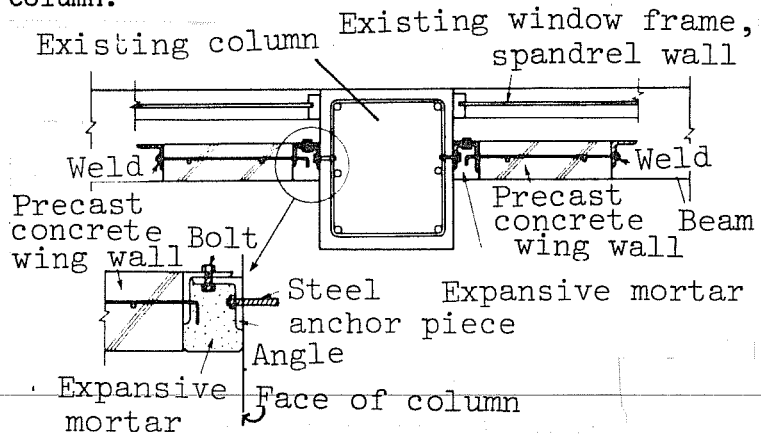
b. Wing wall design.
