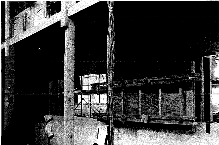
Fig. 2.33 Inside formwork in place after casting lower 4 ft of pier.
