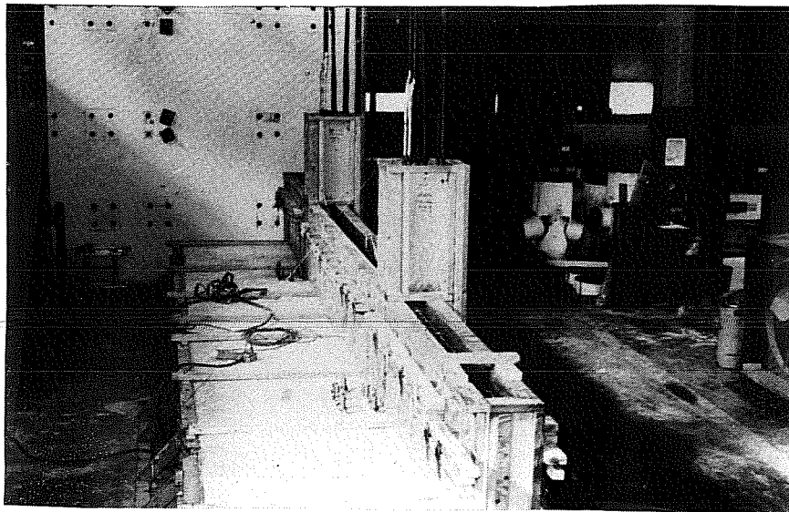
Fig. 2.17 Casting stage 2. Forms in place for first level beam and column
