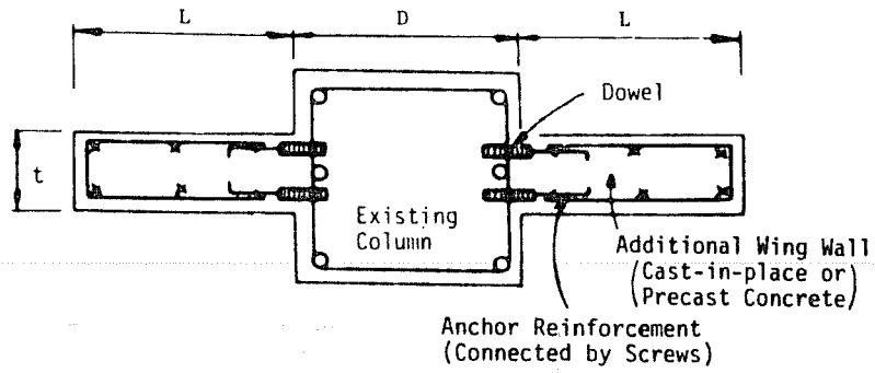
a. Wing wall section.
