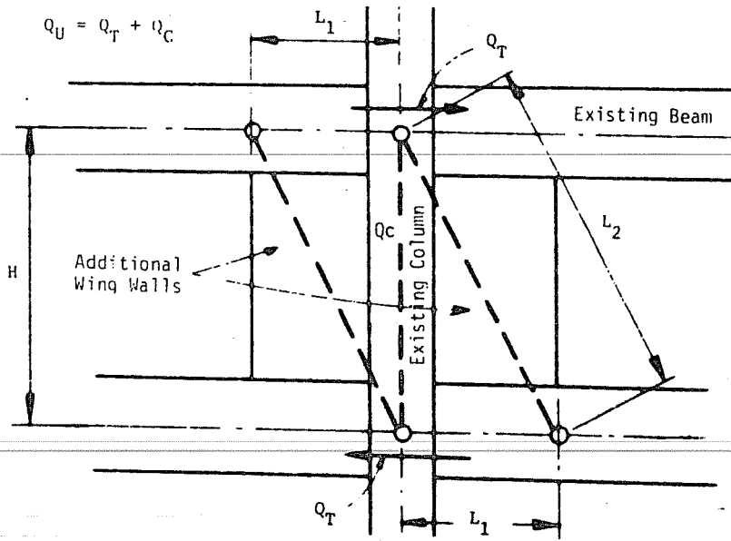
b. Precast panels as compression struts.
