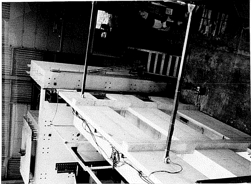
Fig. 2.48 Out-of-plane braces at third level.
