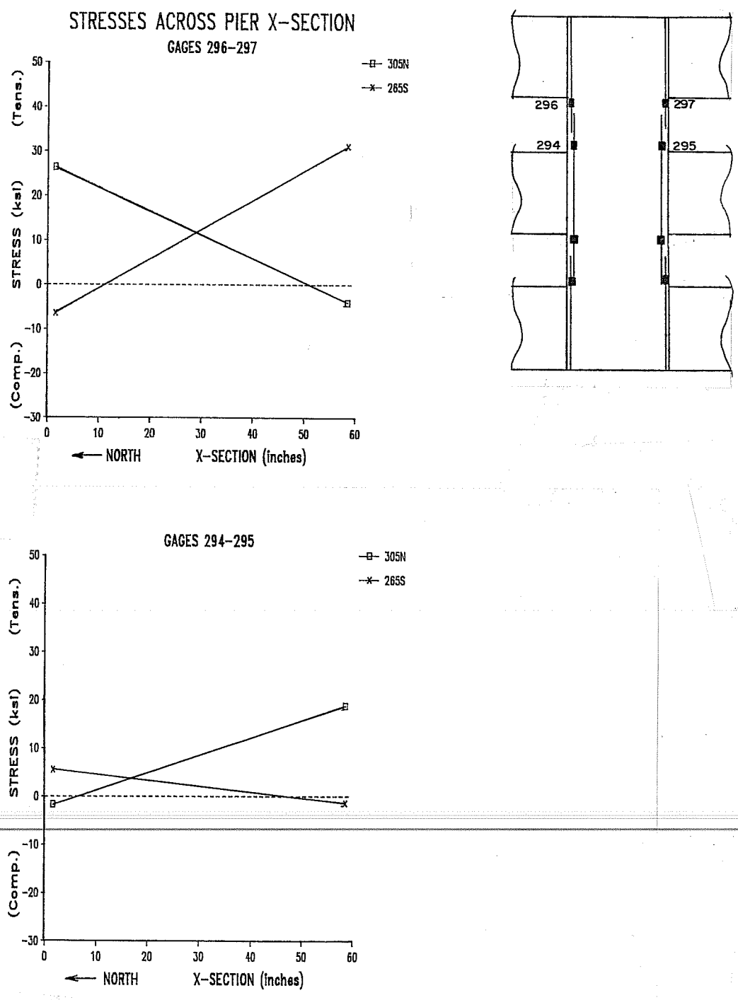
Fig. 4.8 Stress gradients across top and bottom cross sections of south column, second level
