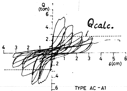
a. Lateral load ( Q ) vs. lateral deflection ( \delta ). Q_{calc} is the shear strength of the un-strengthened column.
