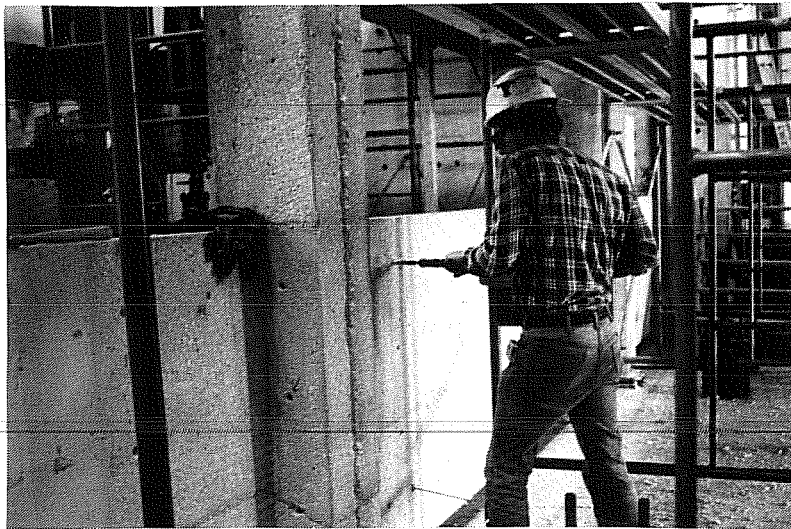
Fig. 2.24 Drilling holes for dowels
