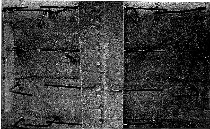
Fig. 2.28 Frame with dowels in place before constructing reinforcing cage.
