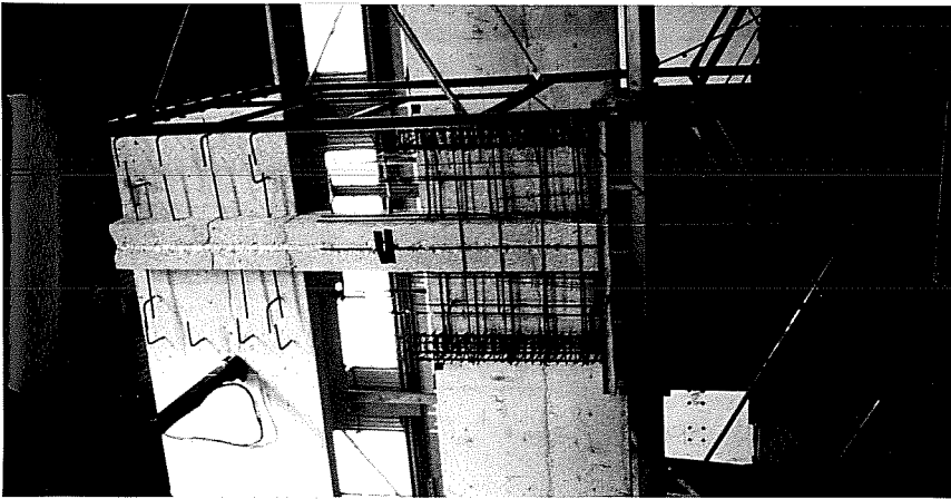
Fig. 2.34 Exterior formwork for casting stage 1.
