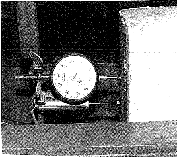
Fig. 2.54 LVDT (channel 182) and dial gage measuring vertical direction of the first level beam
