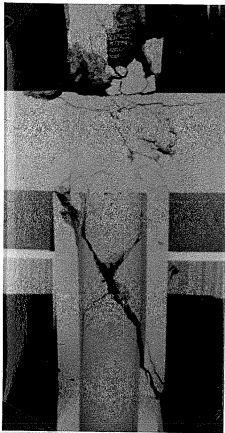
Fig. 1.2 Typical short column shear failure. Olive View Hospital, San Fernando 1971.
