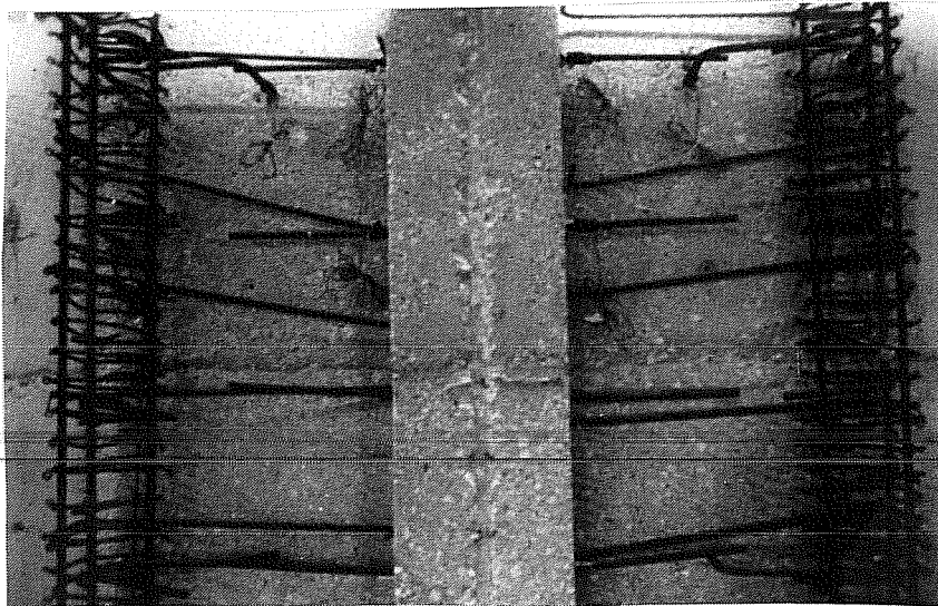
Fig. 2.29 Boundary elements in place with three or four longitudinal bars
