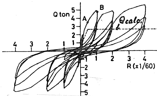
a. Lateral load (Q) vs. lateral deflection ( \delta ).
