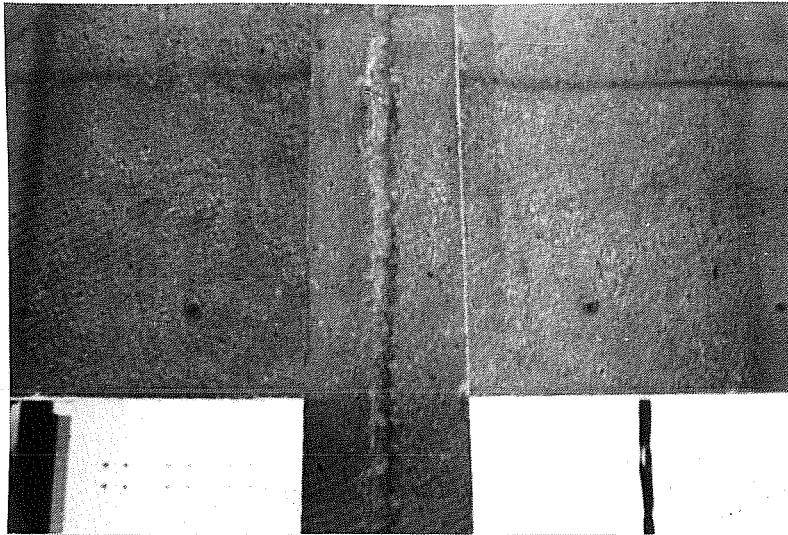
Fig. 2.23 Frame prepared by sandblasting surface and chipping groove in column face
