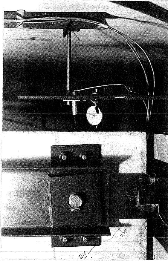
Fig. 2.55 LVDT (channel 180) measuring horizontal deflection of the first level beam
