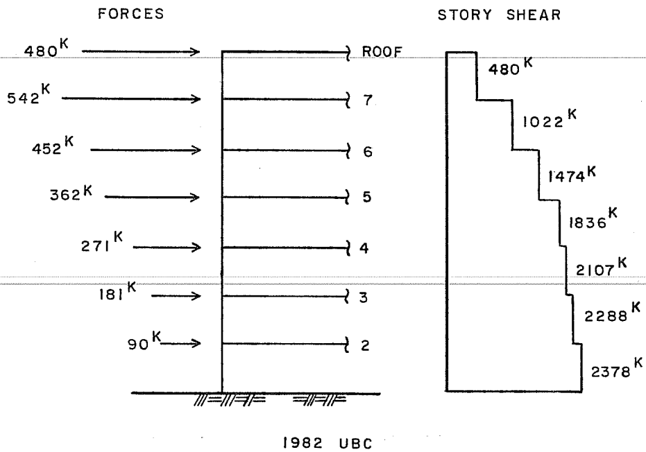
Fig. 2.3 Design loads for prototype building based on UBC earthquake regulations
