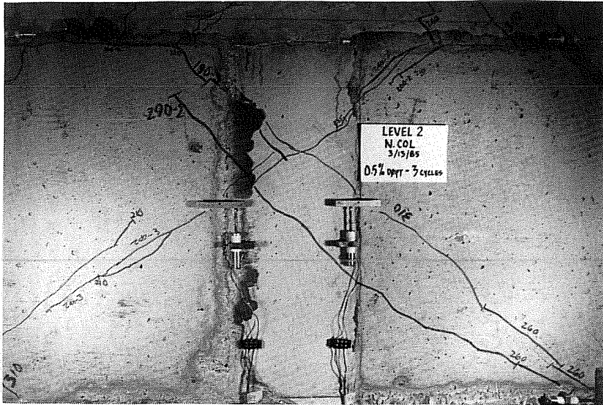
Fig. 3.14 Marked shear cracks on interior of north pier, second level, 0.5% drift
