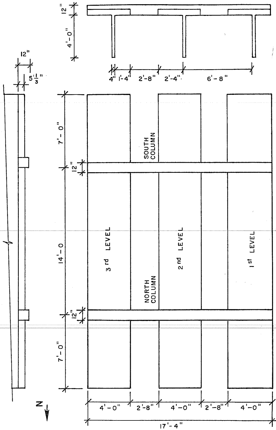
Fig. 2.9 Test Specimen (existing structure) - two bays between 3rd and 5th stories of exterior moment resisting frame
