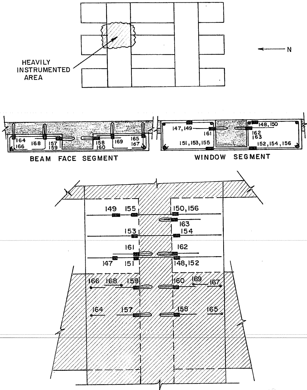
Fig. 2.51 Strain gage locations on dowels and transverse reinforcement in the pier
