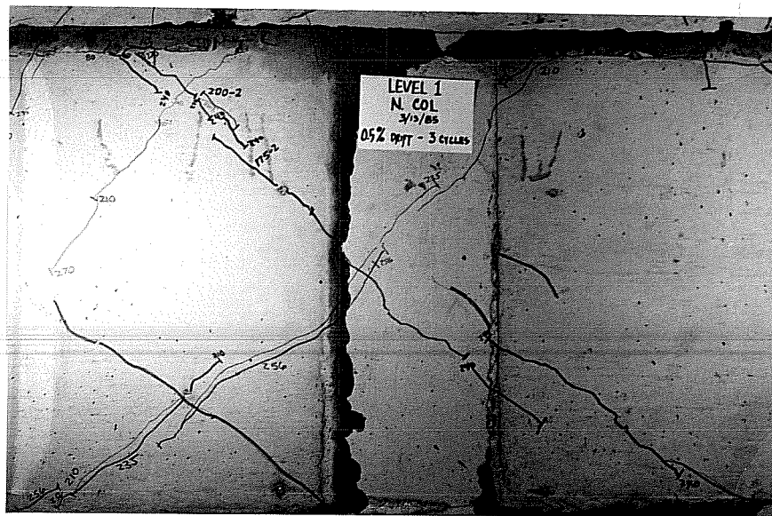
Fig. 3.15 Marked shear cracks on interior of north pier, first level, 0.5% drift.
