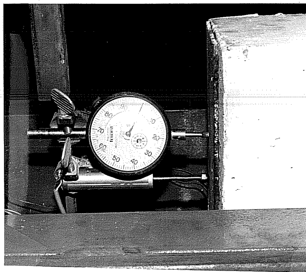
Fig. 2.54 LVDT (channel 182) and dial gage measuring vertical deflection of the first level beam.
