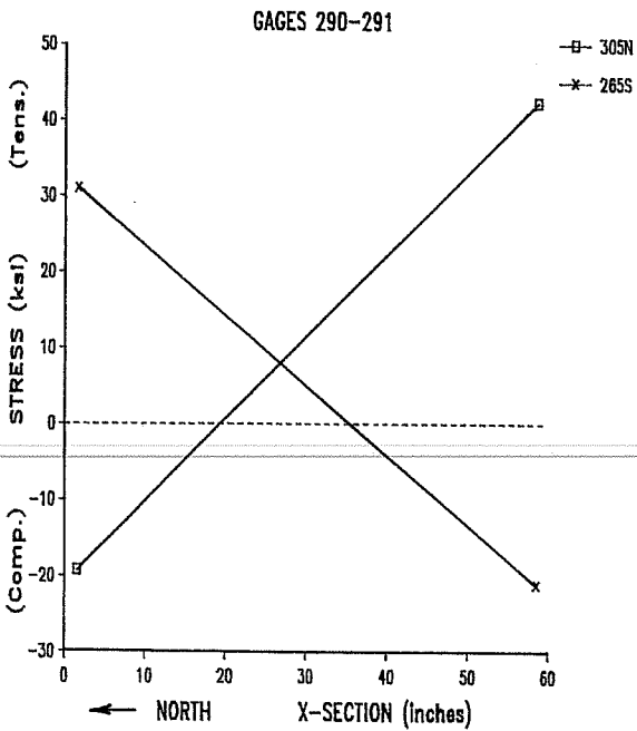
Fig. 4.7 Stress gradients across top and bottom cross sections of south column, first level
