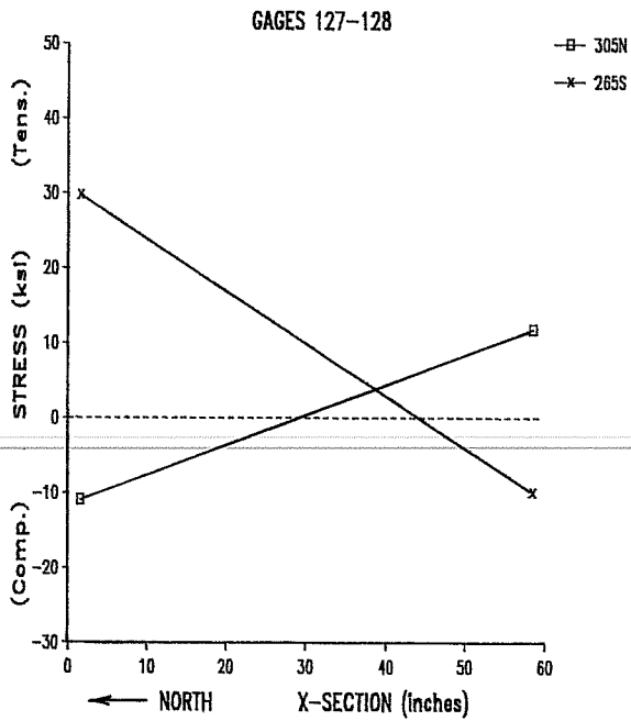
Fig. 4.5 Stress gradients across top and bottom cross sections of north pier, first level
