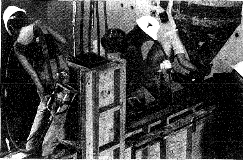
Fig. 2.18 Placing concrete in upper portion of beam form
