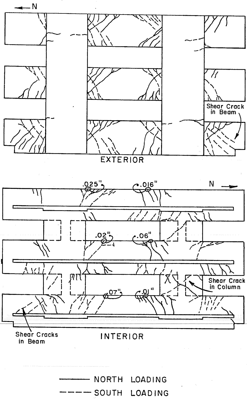
Fig. 3.8 Crack pattern after three cycles to 0.25% drift
