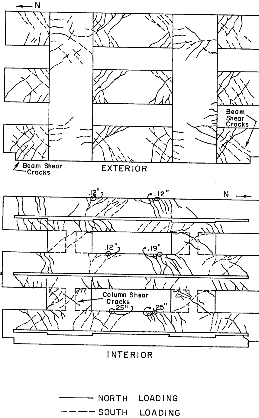
Fig. 3.11 Crack pattern after three cycles to 0.5% drift
