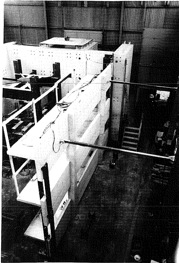
Fig. 2.20 The completed existing frame model
