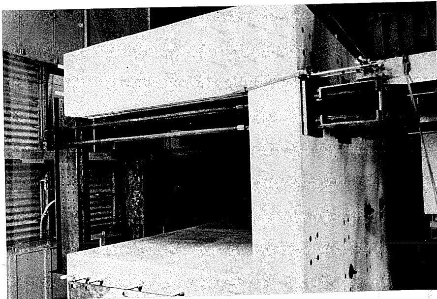
Fig. 2.39 Loading frame connection to reaction wall buttresses.
