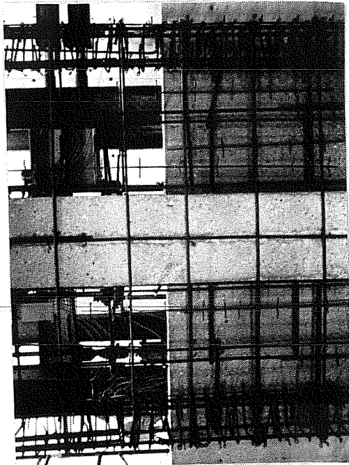
Fig. 2.30 Transverse and longitudinal steel in place
