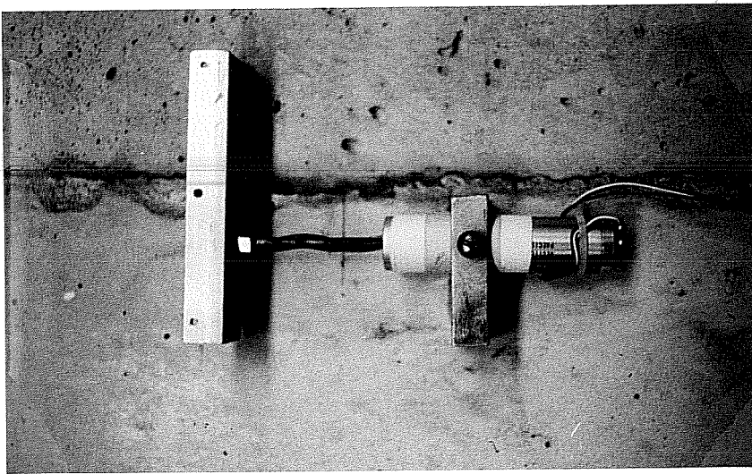
Fig. 2.56 LVDT (channel 188) used to measure slip between the original column and the pier.
