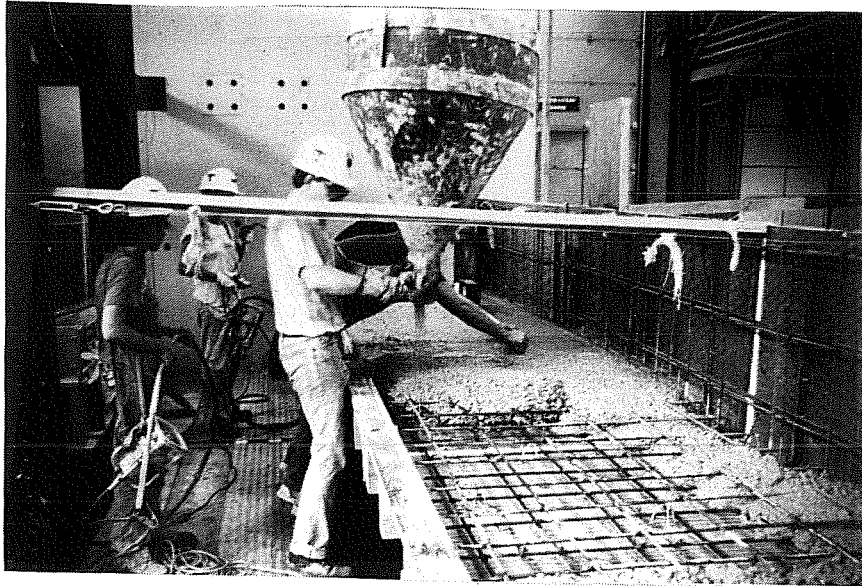
Fig. 2.16 Casting stage 3. Concrete placed to top of second level slab
