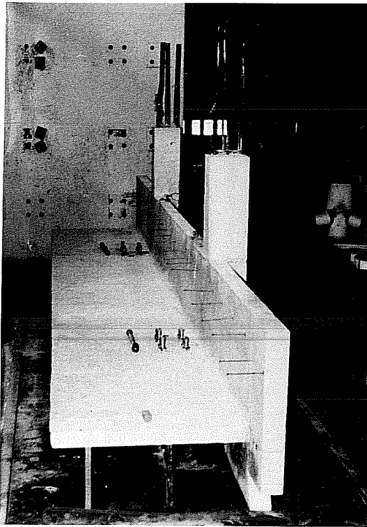
Fig. 2.19 Forms were stripped after casting stage 2.
