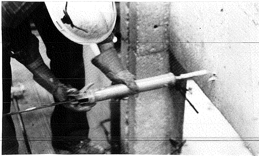
Fig. 2.26 Placing epoxy in dowel hole with caulking gun
