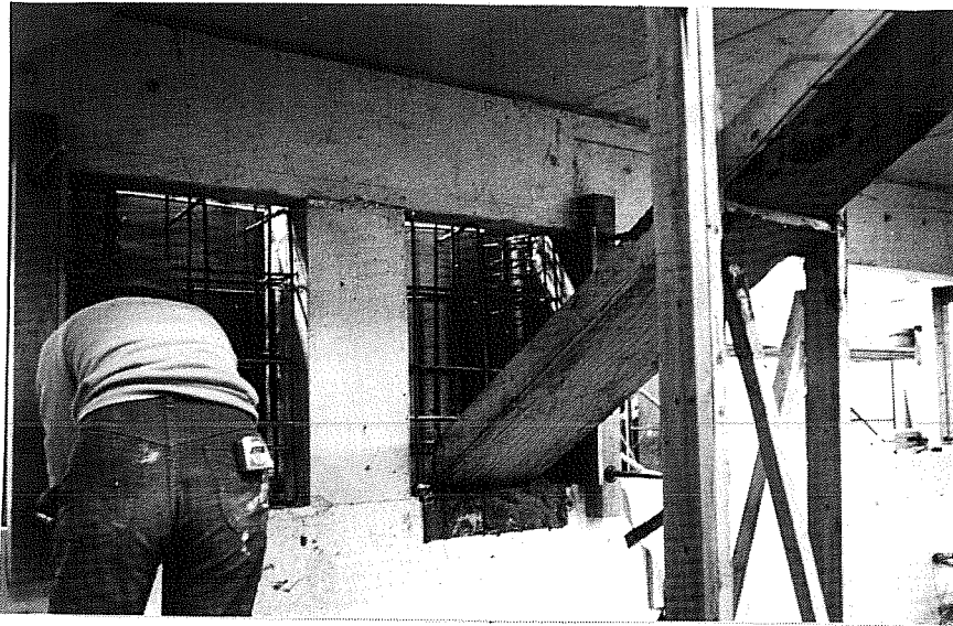
Fig. 2.32 Concrete was placed from the interior of the frame using a chute which emptied into the formwork
