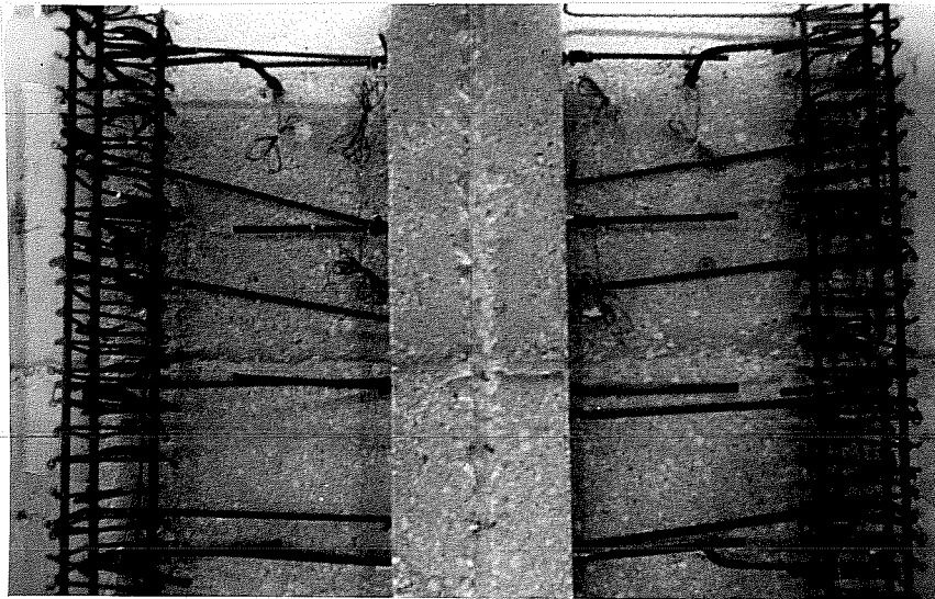
Fig. 2.29 Boundary elements in place with three of four longitudinal bars.
