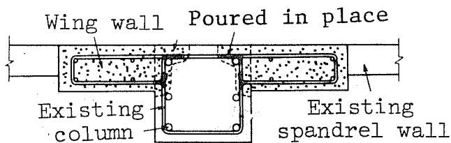
b. Wing wall design.
