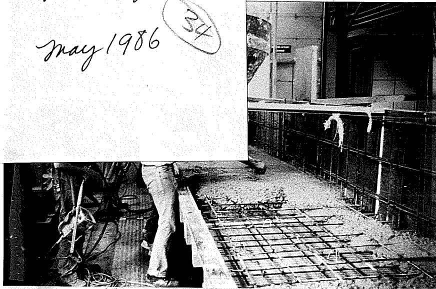
Fig. 2.16 Casting stage 3. Concrete placed to top of 2nd level slab.
