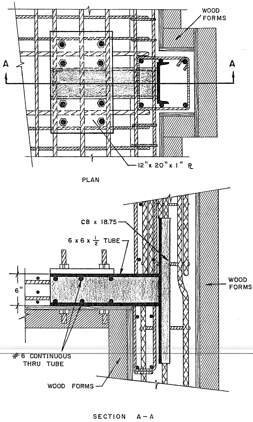
Fig. 2.41 Structural steel assembly embedded in drop panel - column area, shown in form-work before placing concrete
