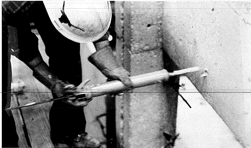
Fig. 2.26 Placing epoxy in dowel hole with caulking gun.
