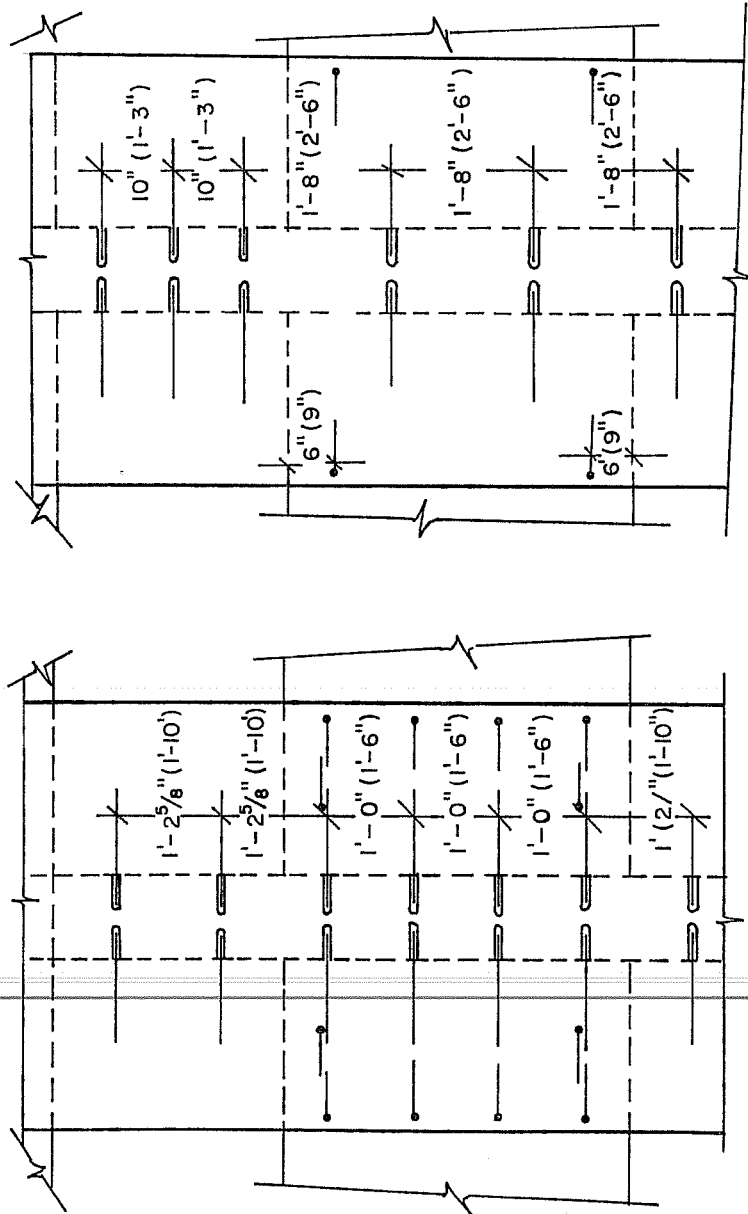
a. Original design.
