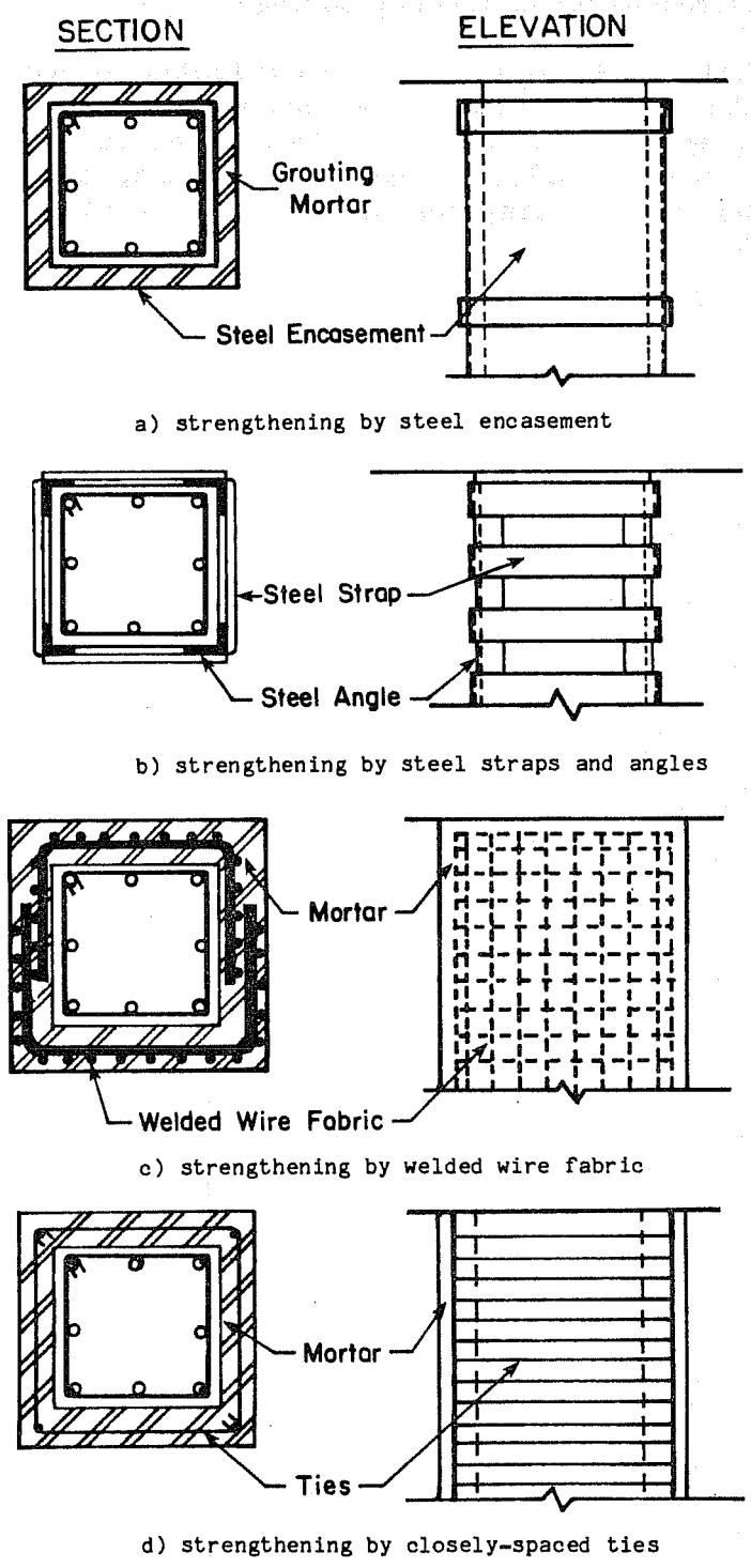
Fig. 1.4 Techniques to increase shear capacity [13].
