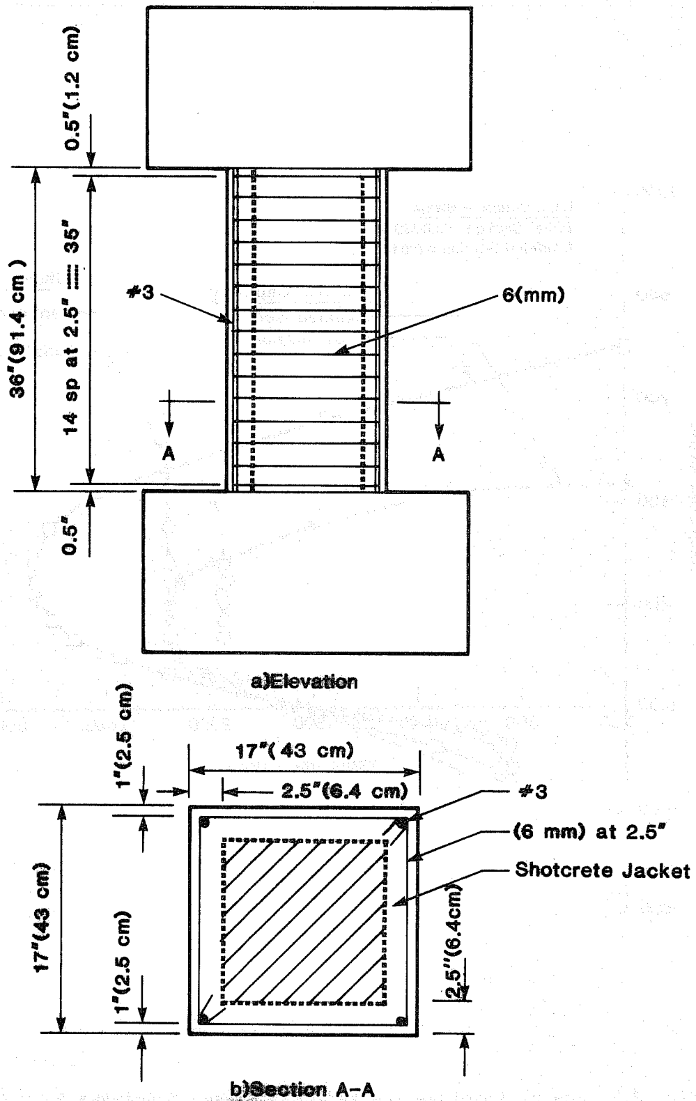
Fig. 2.6 Details of Specimen 1-2.
