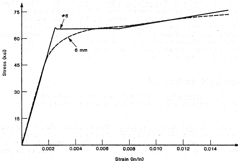
Fig. 2.5 Stress-strain curve for original specimen steel reinforcement
