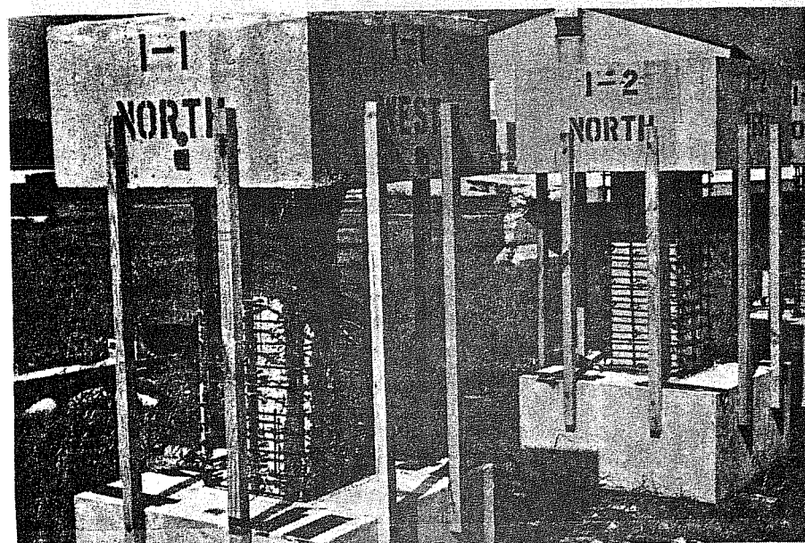
Fig. 2.13 Screed guides
