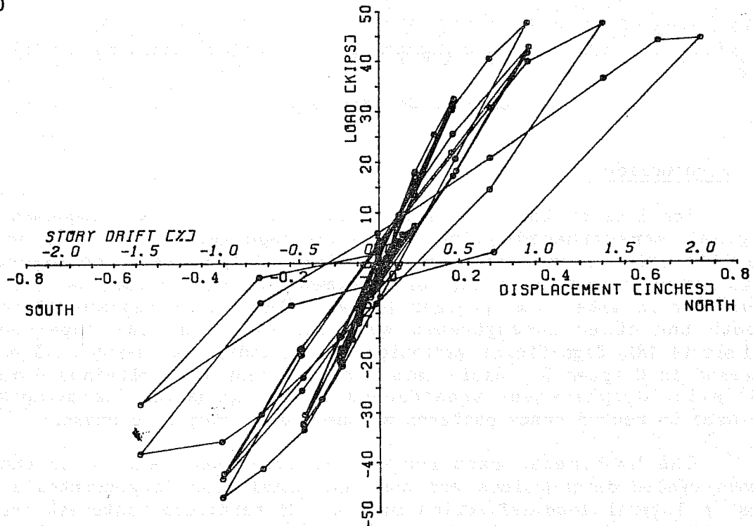
Fig. 4.1 Load-deflection curve, Specimen 1-1
