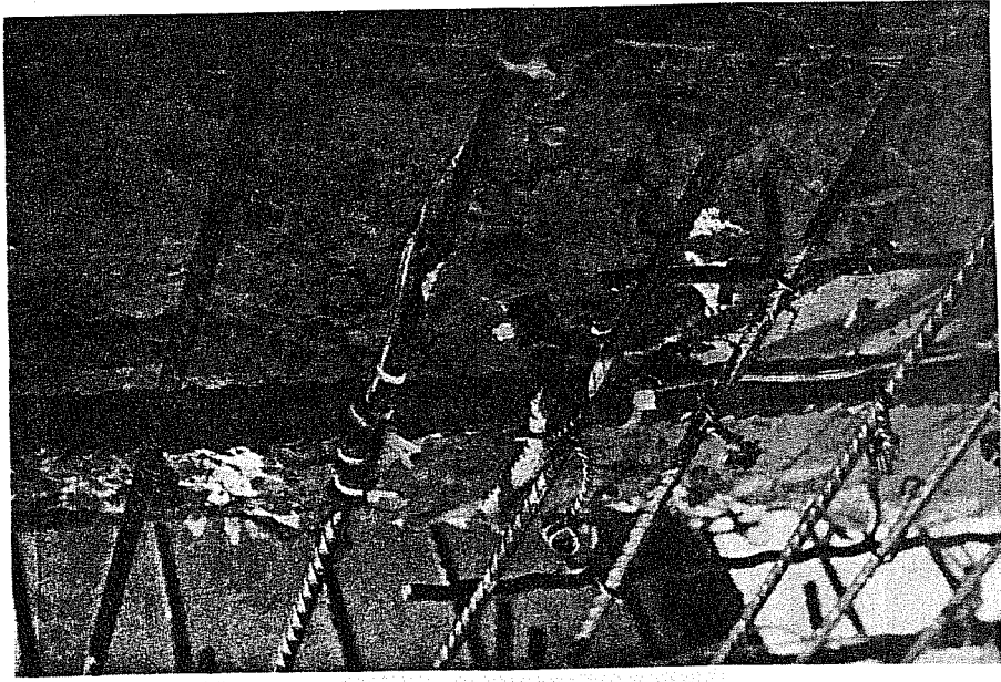
Fig. 2.12 Crossties secured by epoxy, Specimen 1-1
