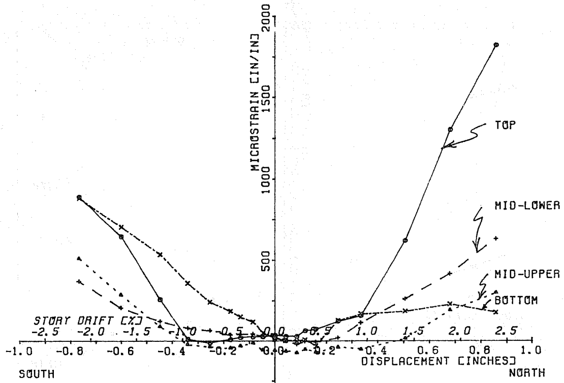
Fig. 4.17 Strain envelopes, N-S crossties, Specimen 1-3
