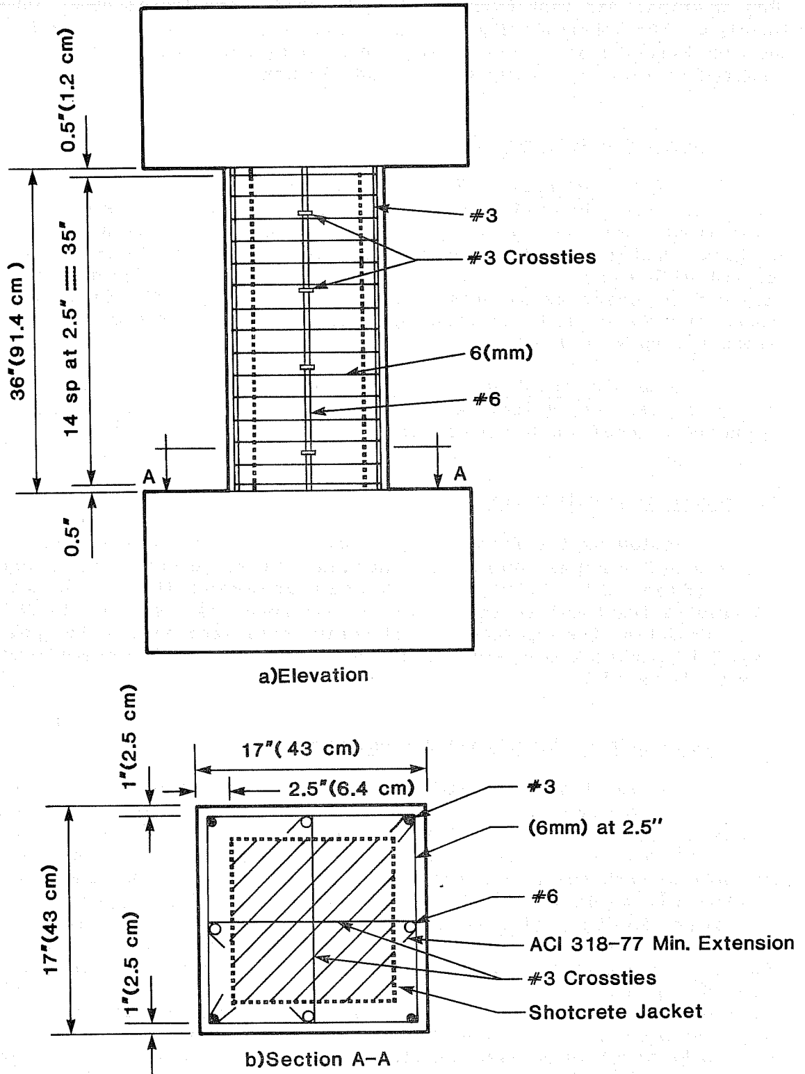
Fig. 2.8 Details of Specimen 1-3.
