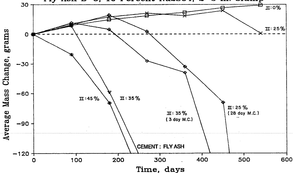
Figure 7.71 Sulfate mass loss of concrete containing fly ash B-5.
