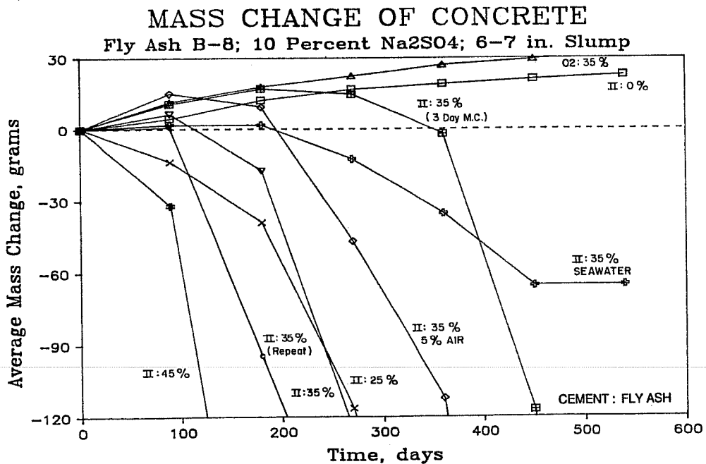
Figure 7.79 Sulfate mass loss of concrete containing fly ash B-8.
