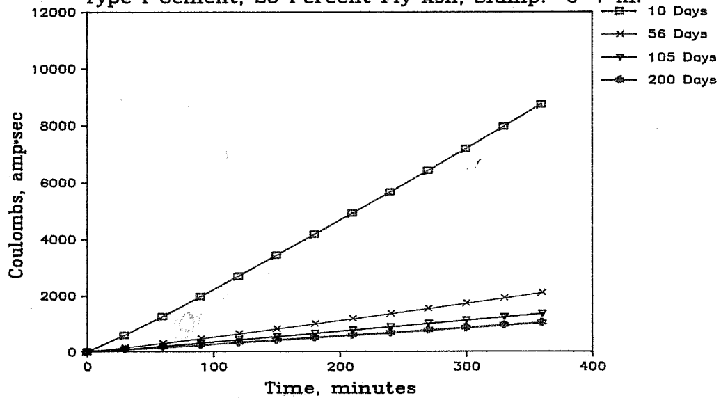
Figure D.4 Permeability of concrete containing fly ash A-4.
