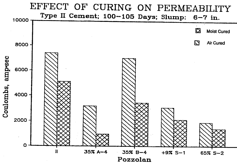
Figure 6.10 Comparison of 105-day permeability of concrete containing pozzolans.
