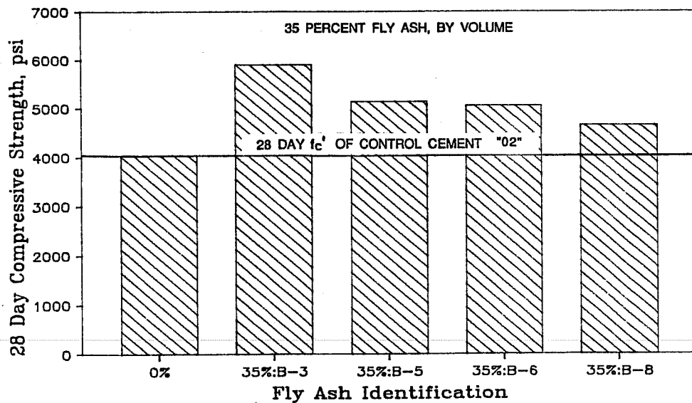
Figure 8.4 Compressive strength of concrete containing high calcium fly ash.
