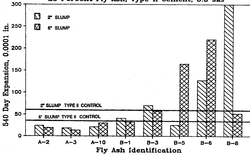
Figure 8.46 Effect of slump on the sulfate resistance of concrete containing 25 percent fly ash.
