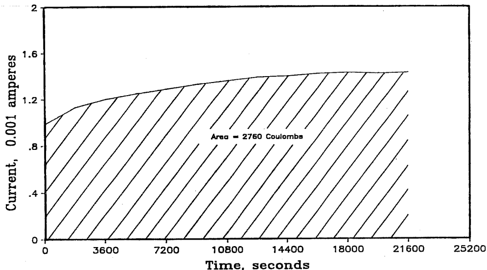
Figure 6.2 Integrated current-time function.
