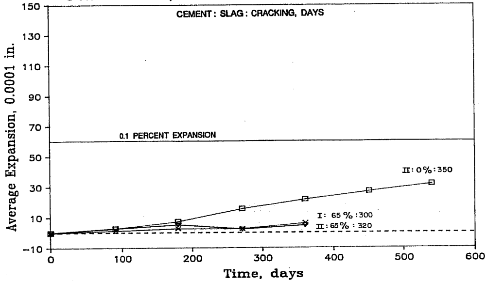
Figure 7.84 Sulfate expansion of concrete containing slag.
