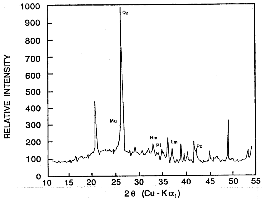
Figure C.7 X-ray diffractogram of fly ash A-7.
