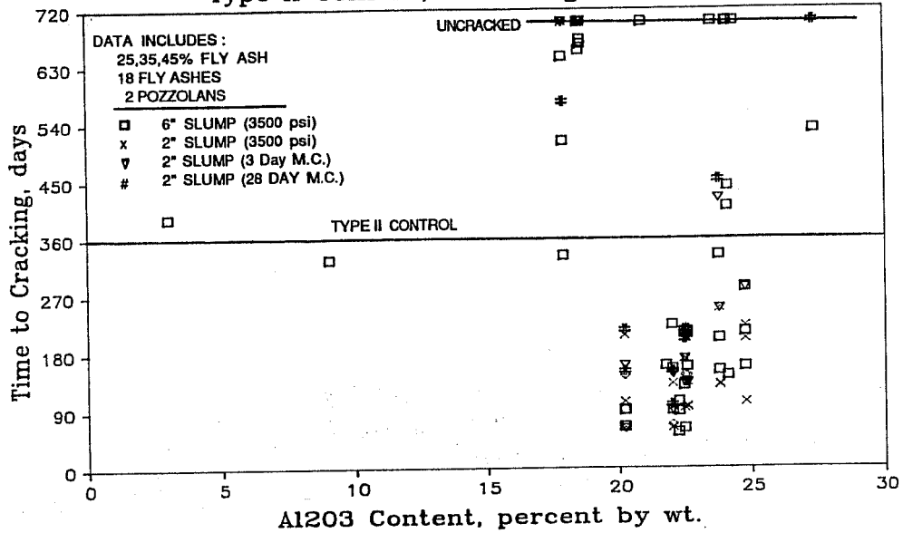
Figure 8.16 Effect of fly ash bulk Al 2 O 3 on sulfate cracking.
