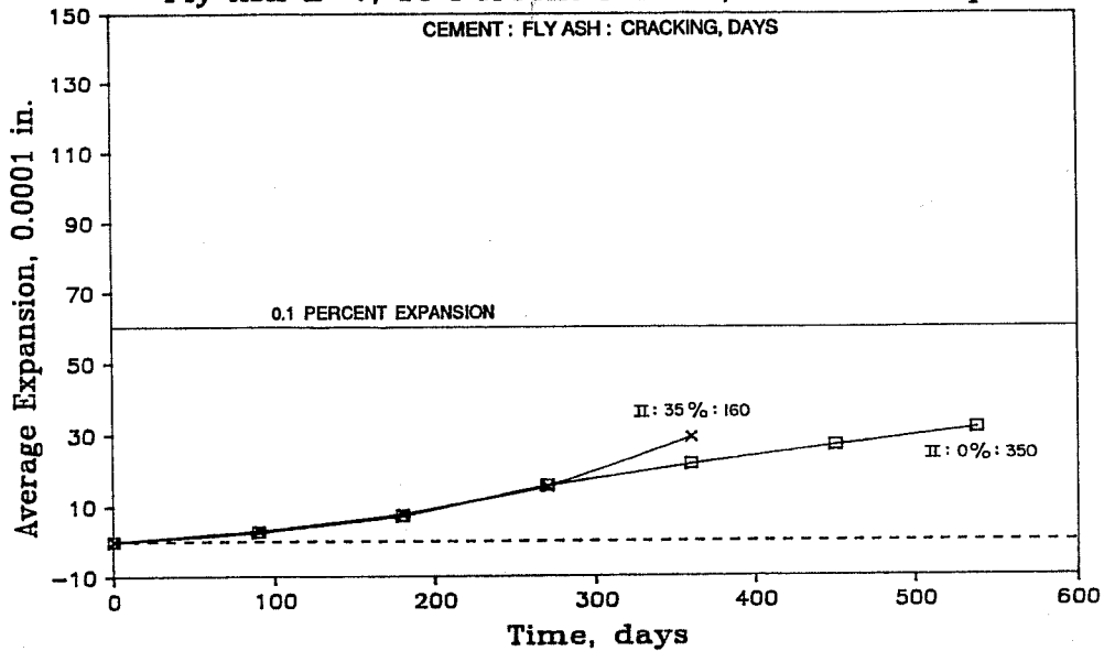
Figure 7.76 Sulfate expansion of concrete containing fly ash B-7.
