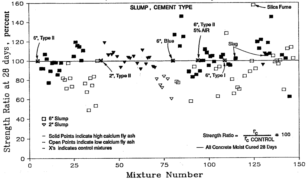
Figure 8.1 Distribution of strength ratios of concrete containing fly ash.
