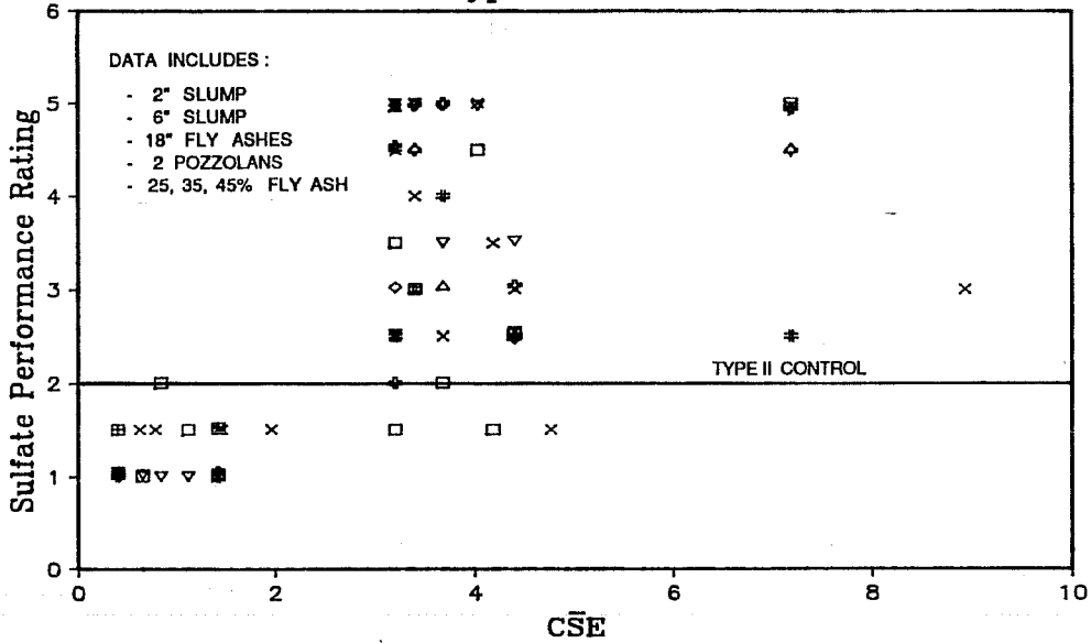
Figure 8.59 Calculate sulfate equivalence of concrete containing fly ash.
