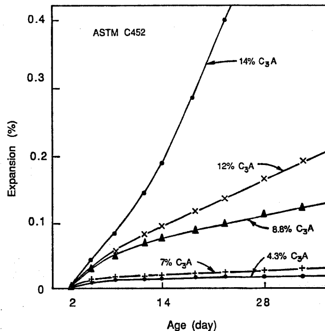
Figure 2.2 Effect of C 3 A content on sulfate resistance 74 .
