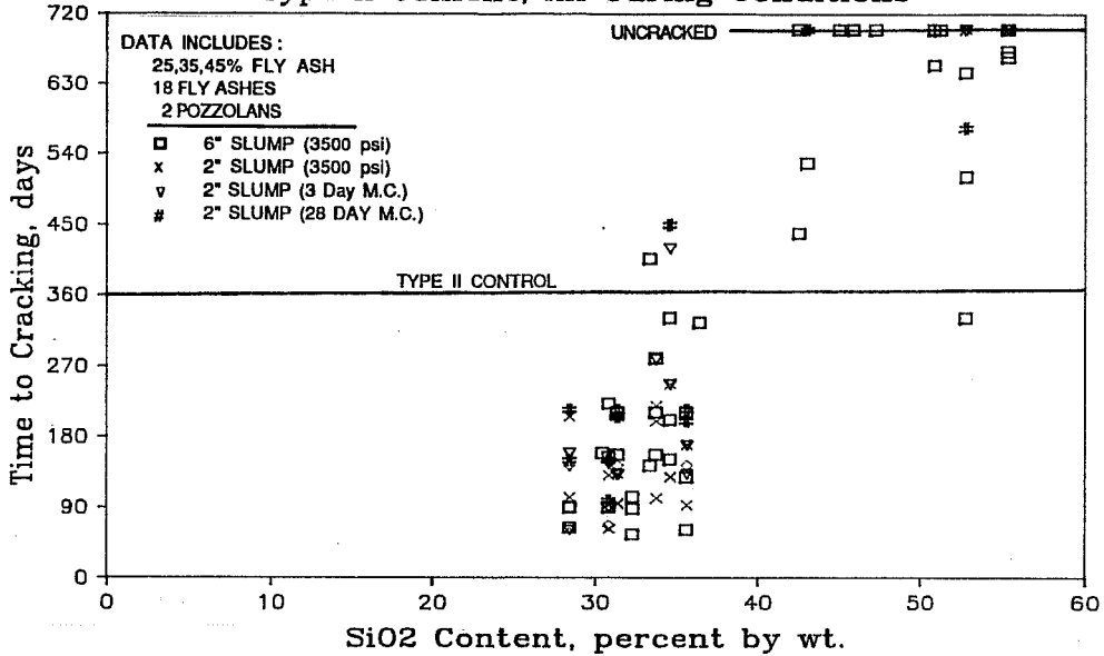
Figure 8.14 Effect of fly ash bulk SiO 2 on sulfate cracking.
