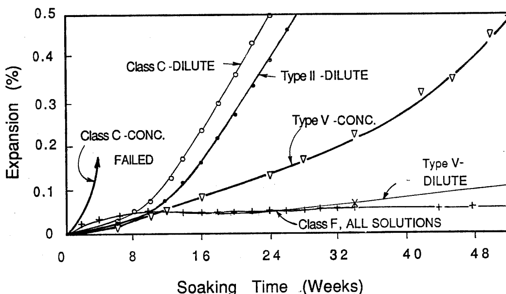
Figure 3.6 Mortar bar testing for sulfate resistance.
