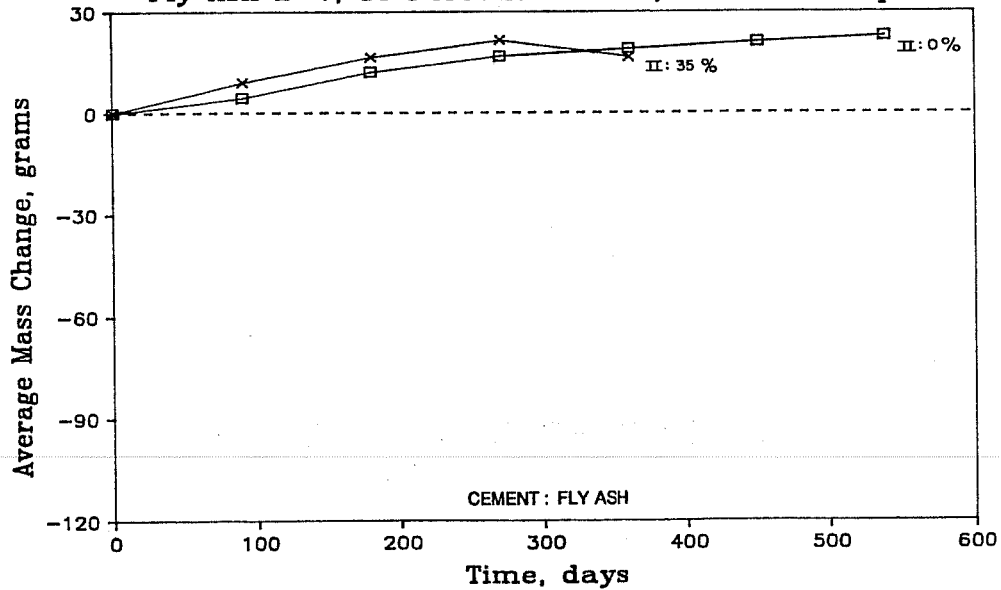
Figure 7.77 Sulfate mass loss of concrete containing fly ash B-7.
