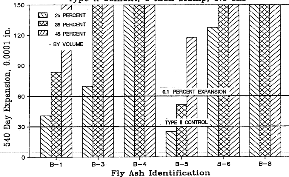
Figure 8.11 Effect of Type B fly ash content on sulfate expansion.
