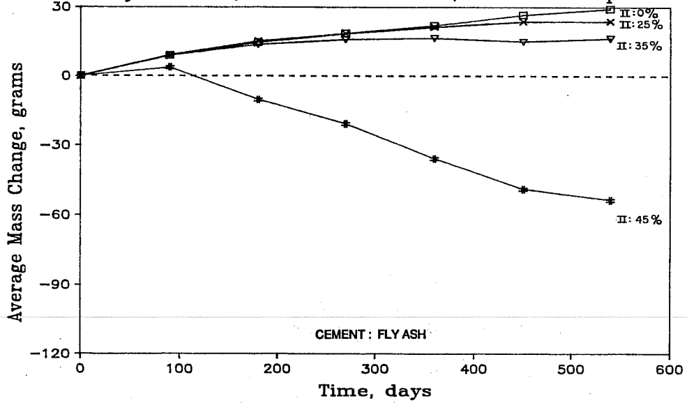
Figure 7.59 Sulfate mass loss of concrete containing fly ash B-1.
