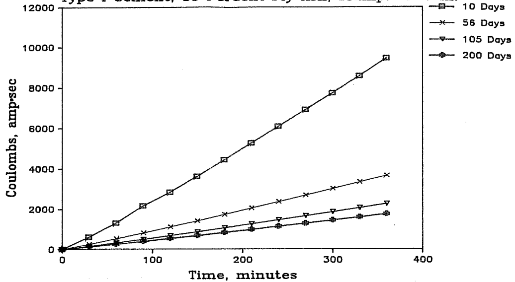
Figure D.3 Permeability of concrete containing fly ash B-4.
