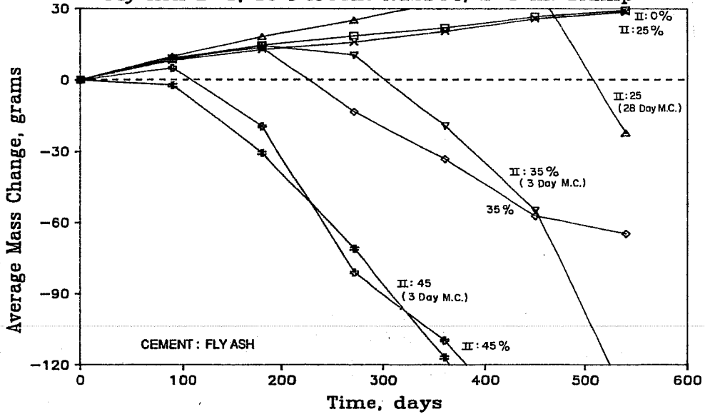
Figure 7.65 Sulfate mass loss of concrete containing fly ash B-3.
