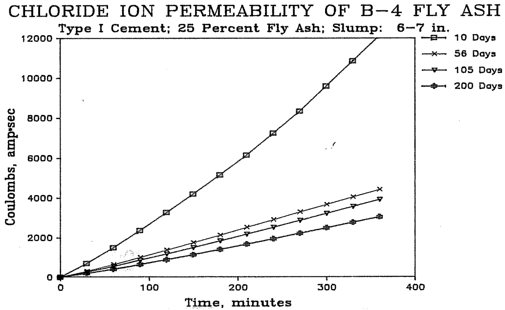
Figure D.2 Permeability of concrete containing fly ash B-4.
