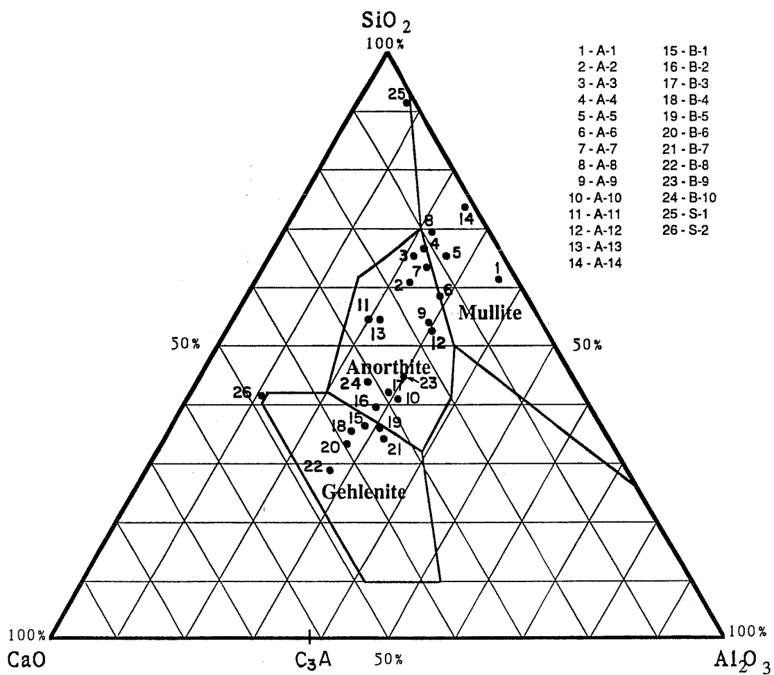
CaO • Al 2 O 3 • SiO 2 ternary oxide system diagram.
