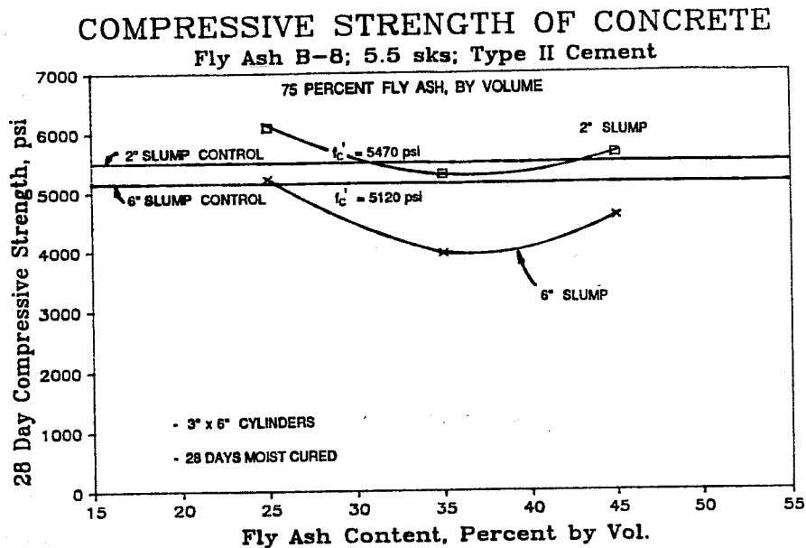
Figure 8.6 Effect of slump and fly ash content on the compressive strength of concrete.
