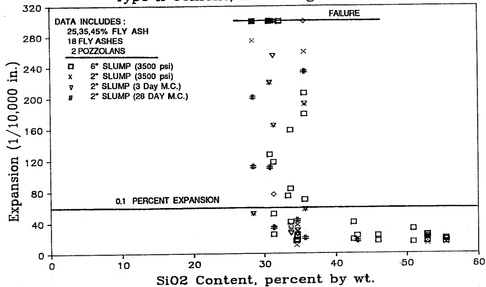
Figure 8.13 Effect of fly ash bulk SiO 2 on sulfate expansion.
