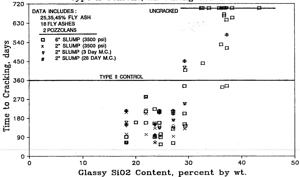
Figure 8.26 Effect of fly ash glassy SiO 2 on sulfate cracking.
