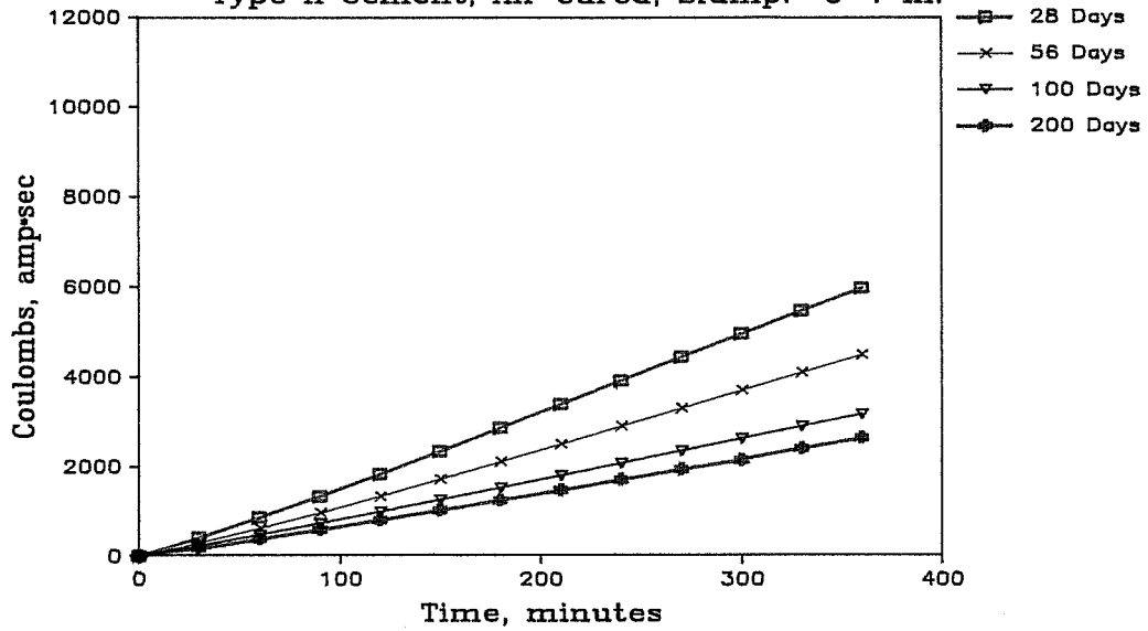
Figure D.14 Permeability of concrete containing fly ash A-4.
