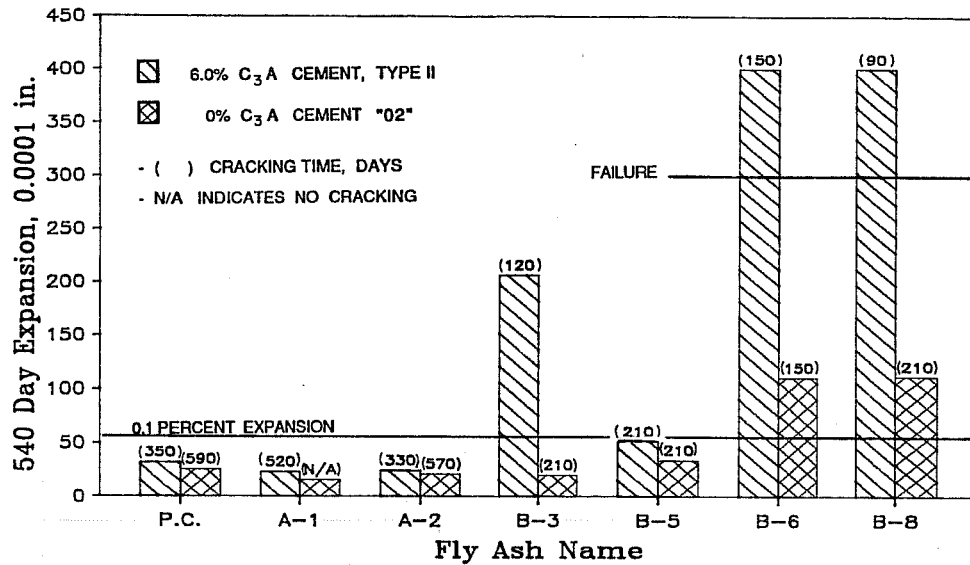
Figure 8.49 Effect of fly ash on the sulfate resistance of sulfate resistant cements.
