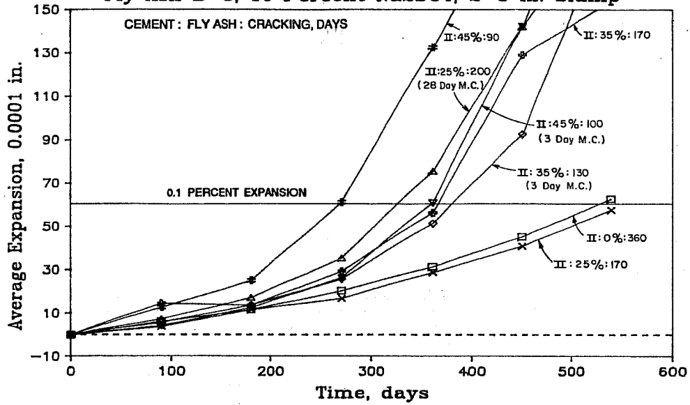
Figure 7.64 Sulfate expansion of concrete containing fly ash B-3.
