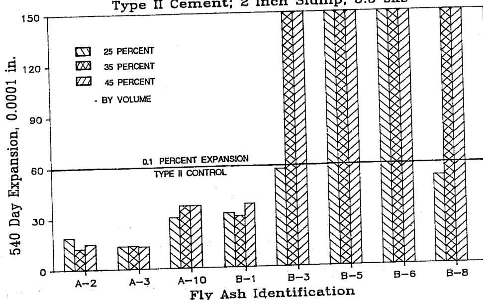
Figure 8.12 Effect of fly ash content on sulfate expansion.
