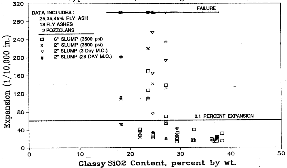
Figure 8.25 Effect of fly ash glassy SiO 2 on sulfate expansion.
