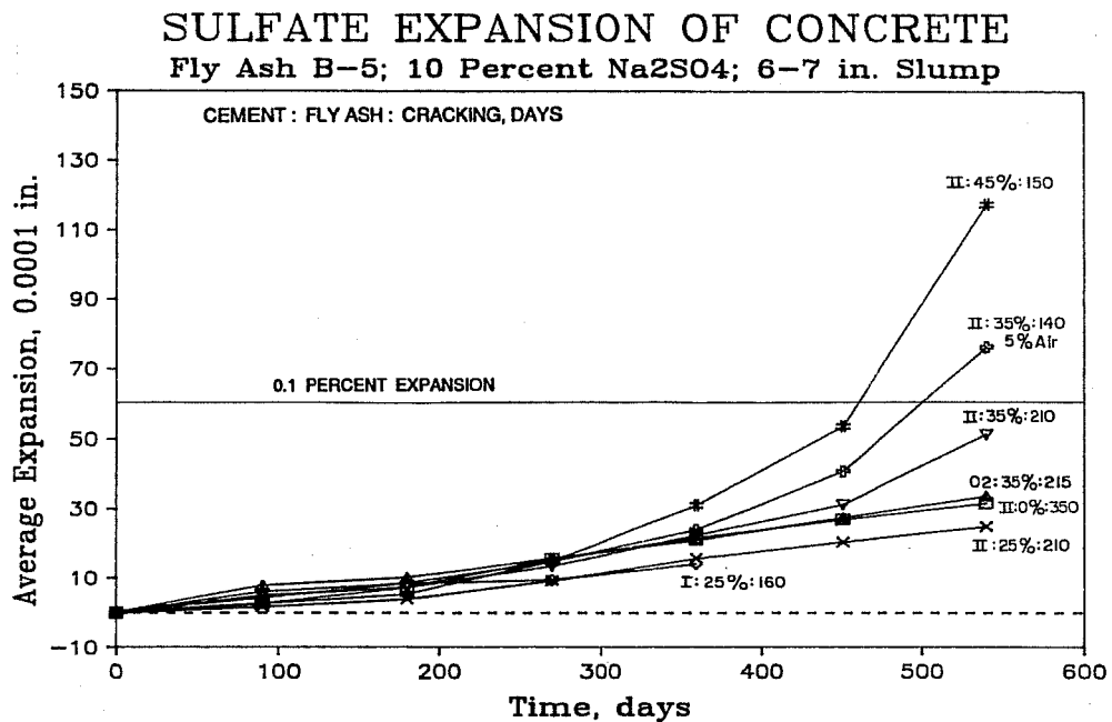
Figure 7.68 Sulfate expansion of concrete containing fly ash B-5.
