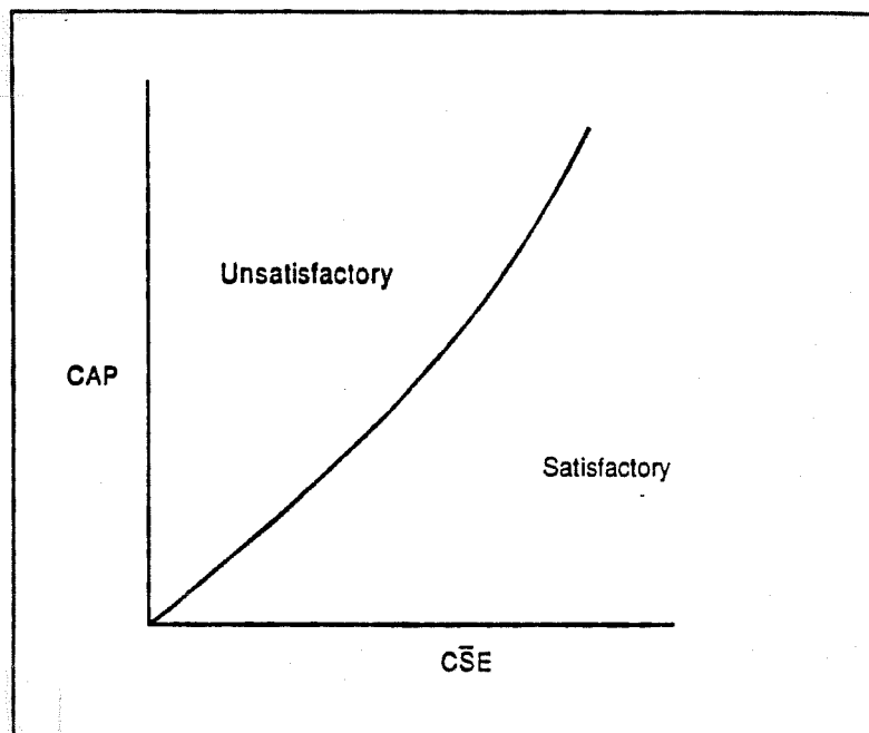
Figure 8.61 Proposed relationship between the CAP and \bar{CSE} factors.
