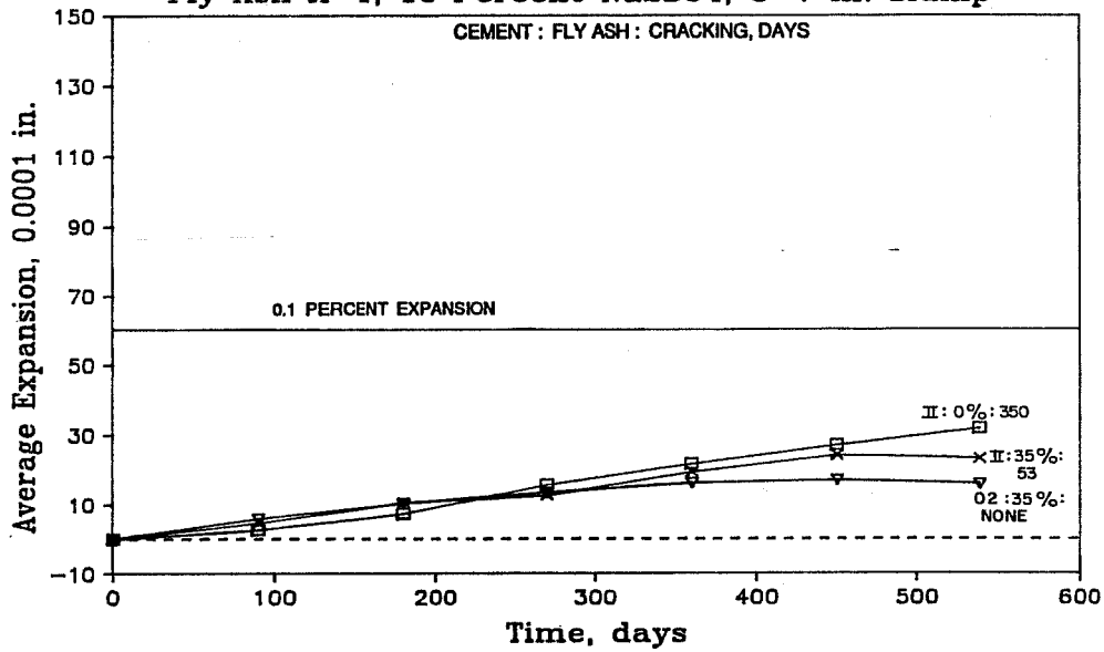
Figure 7.30 Sulfate expansion of concrete containing fly ash A-1.
