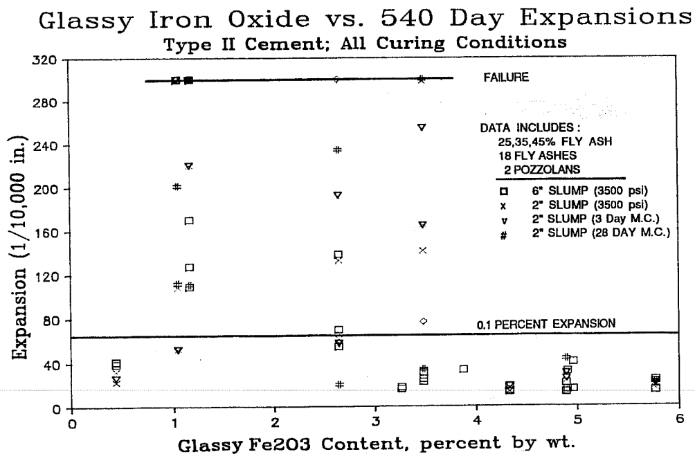
Figure 8.29 Effect of fly ash glassy Fe 2 O 3 on sulfate expansion.
