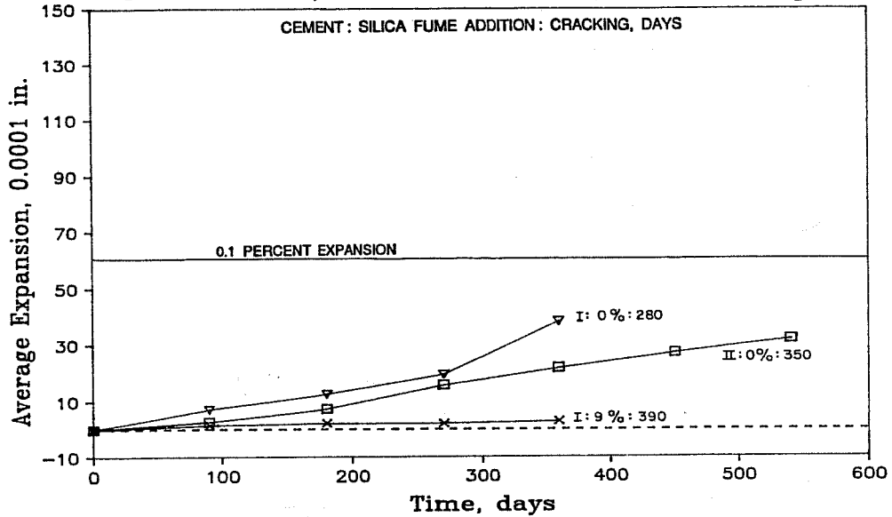
Figure 7.82 Sulfate expansion of concrete containing silica fume.
