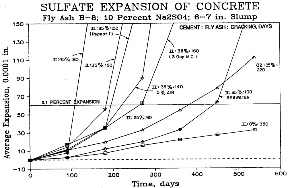
Figure 7.78 Sulfate expansion of concrete containing fly ash B-8.
