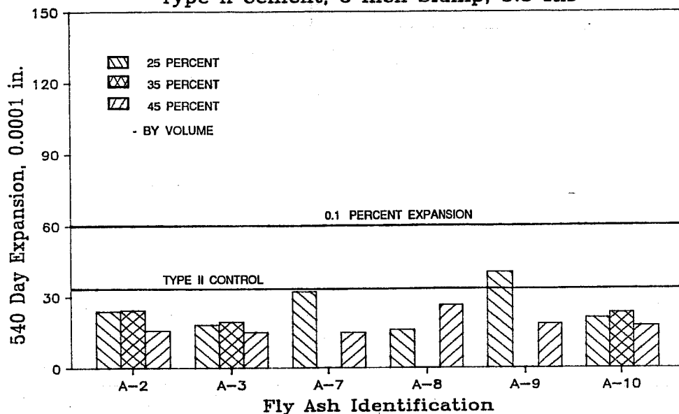
Figure 8.10 Effect of Type A fly ash content on sulfate expansion.
