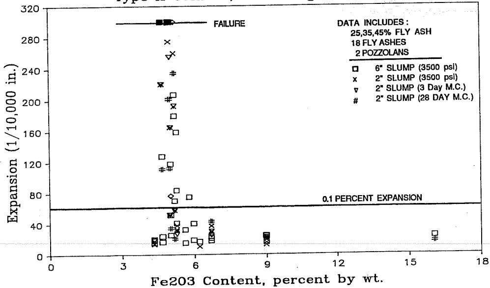
Figure 8.17 Effect of fly ash bulk Fe 2 O 3 on sulfate expansion.
