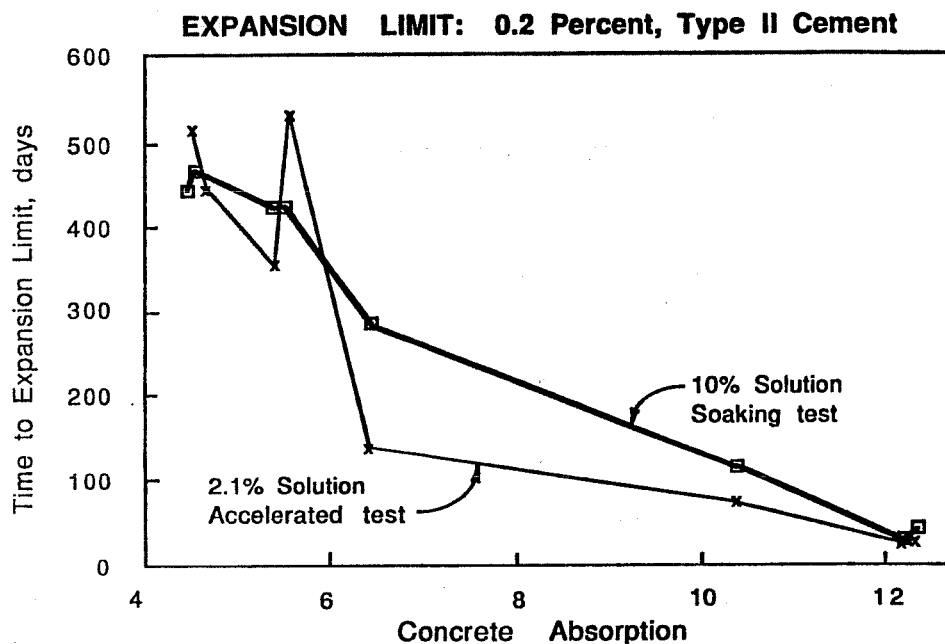
Figure 4.2 Comparison of accelerated sulfate testing methods.
