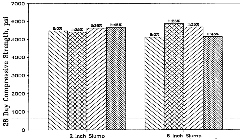
Figure 8.2 Comparison of the compressive strength of 2" and 6" slump concrete containing fly ash A-10.
