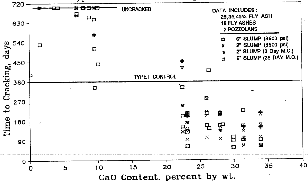
Figure 8.24 Effect of fly ash bulk CaO on sulfate cracking.
