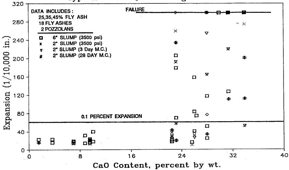
Figure 8.23 Effect of fly ash bulk CaO on sulfate expansion.
