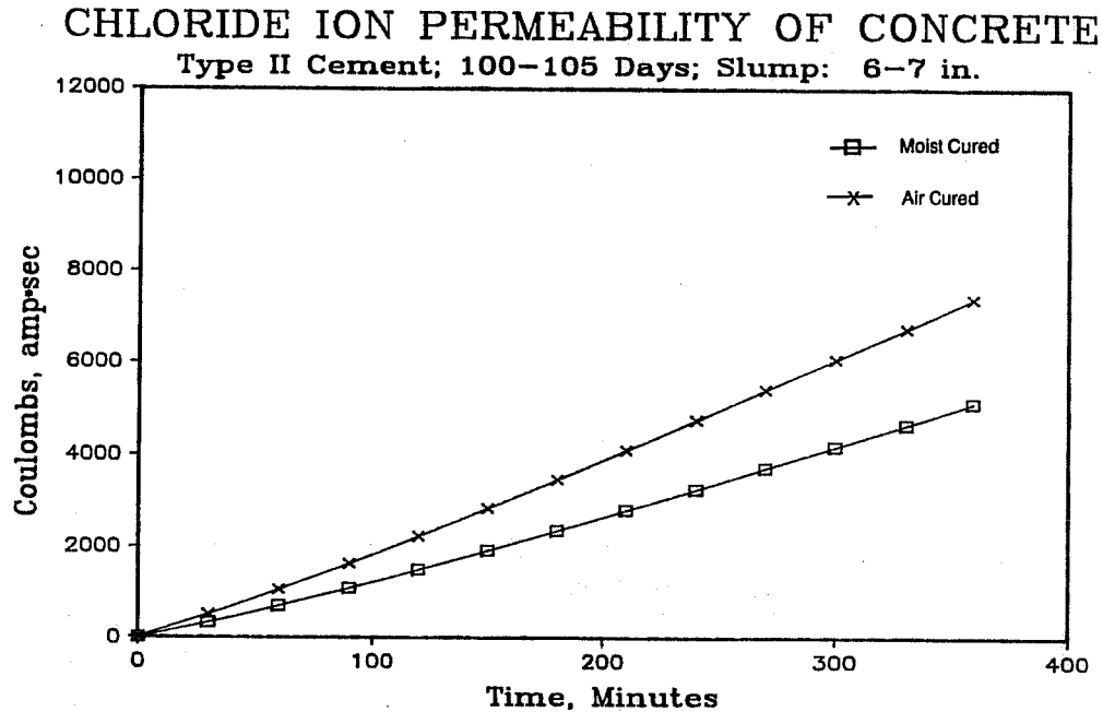
Figure 6.7 Comparison of the permeability of moist and air cured concrete.
