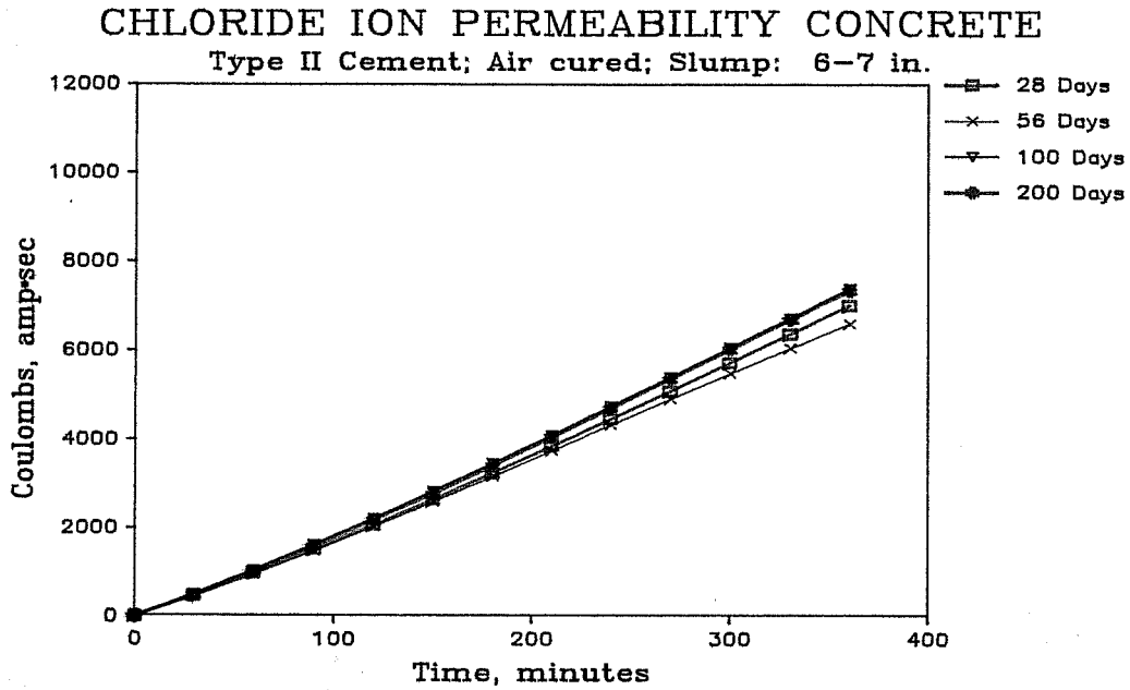
Figure D.12 Permeability of Type II cement concrete.
