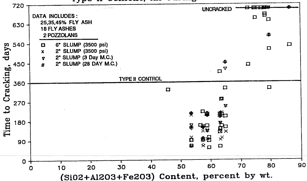
Figure 8.20 Effect of fly ash oxides on sulfate cracking.
