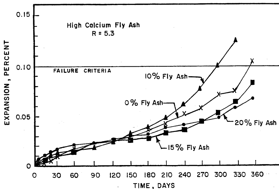
Figure 3.4 Sulfate resistance of concrete containing high calcium fly ash 86 .
