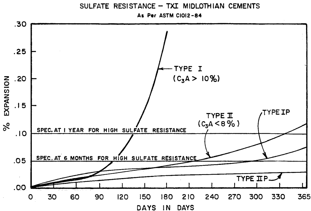
Figure 3.9 Sulfate resistance of blended cements 95 .
