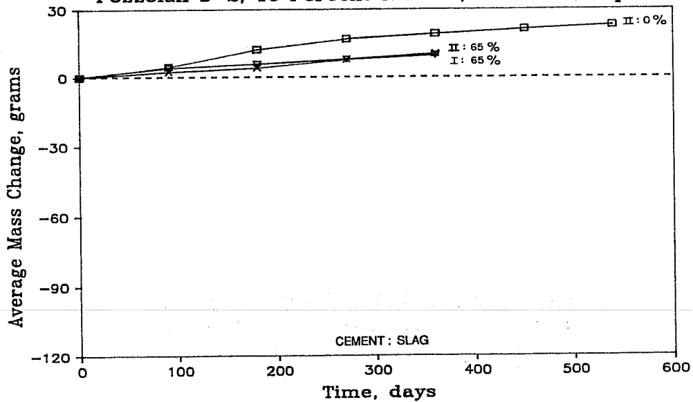
Figure 7.85 Sulfate mass loss of concrete containing slag.
