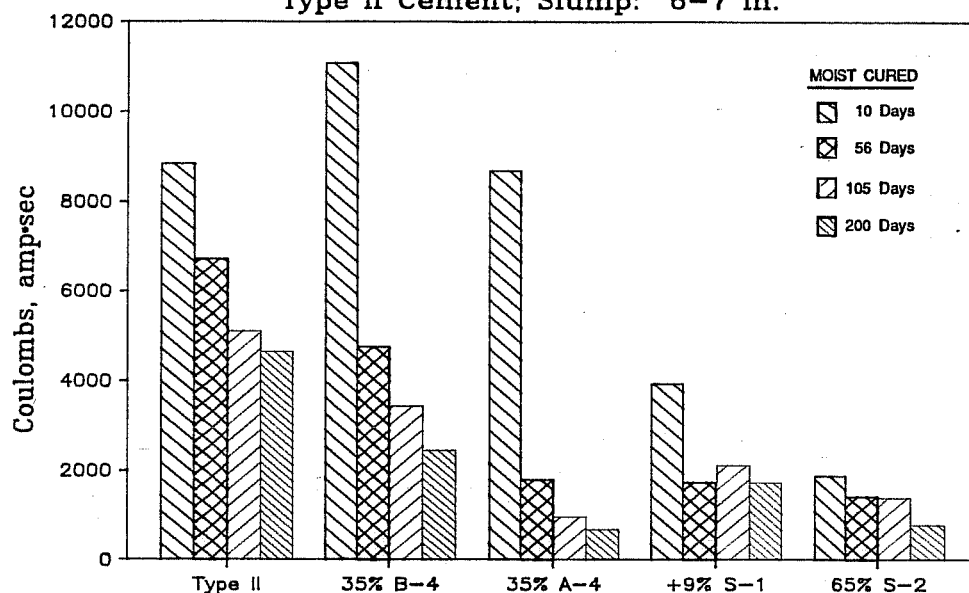
Figure 6.6 Chloride ion permeability of concrete containing pozzolans.
