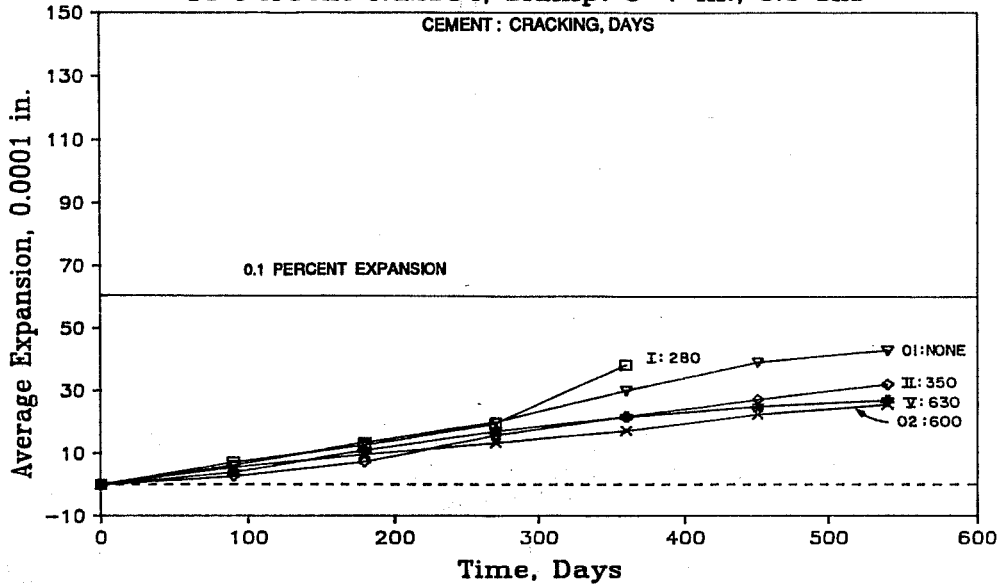
Figure 7.26 Effect of cement type on sulfate resistance.
