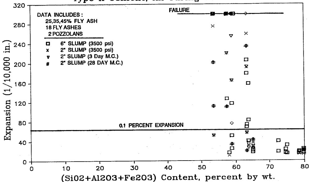
Figure 8.19 Effect of fly ash oxides on sulfate expansion.
