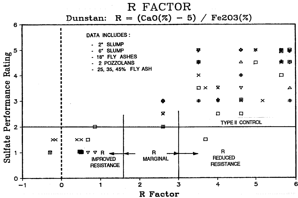
Figure 8.54 Sulfate resistance of fly ashes with the R factor method.
