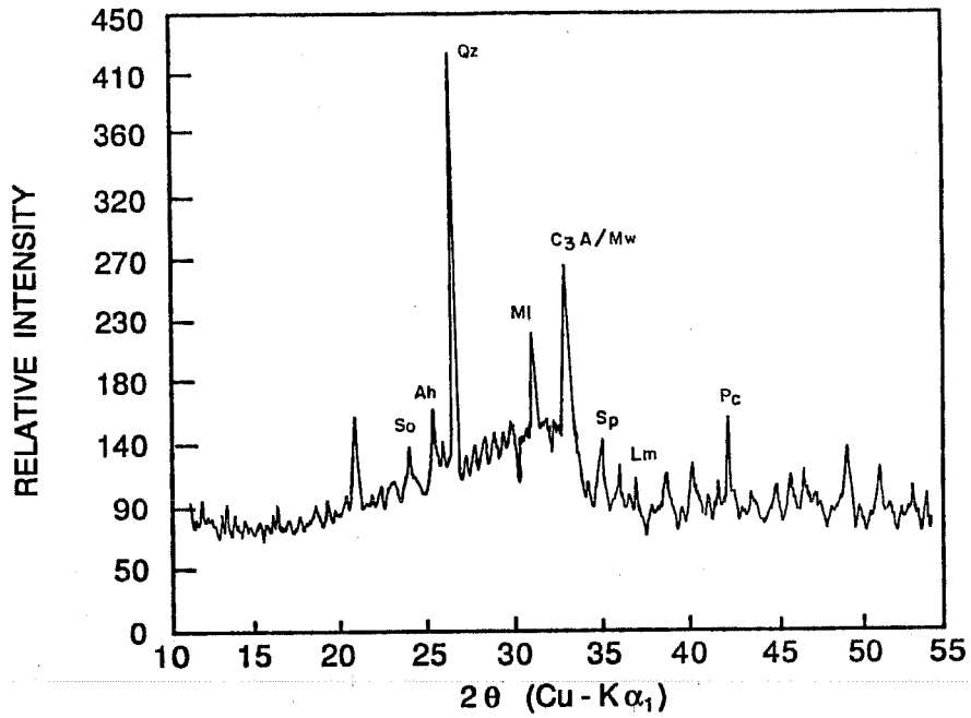
Figure C.15 X-ray diffractogram of fly ash B-5.
