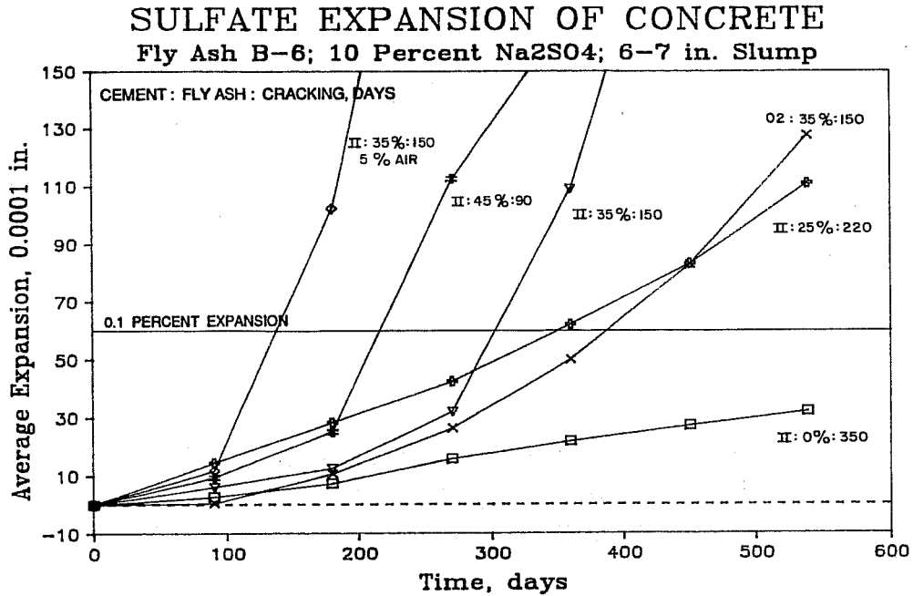
Figure 7.72 Sulfate expansion of concrete containing fly ash B-6.
