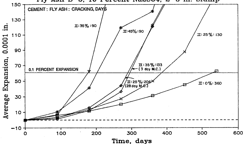
Figure 7.70 Sulfate expansion of concrete containing fly ash B-5.
