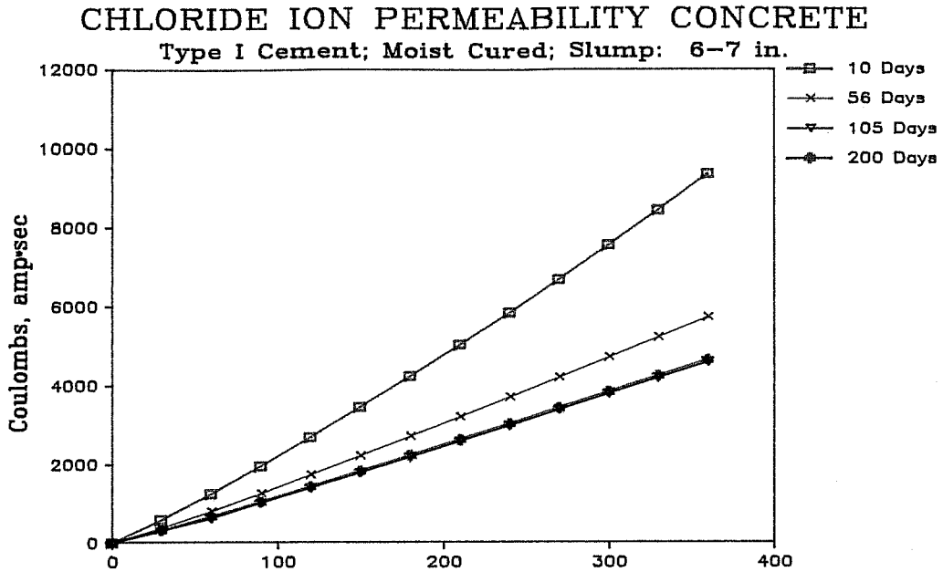
Figure D.1 Permeability of Type I cement concrete.
