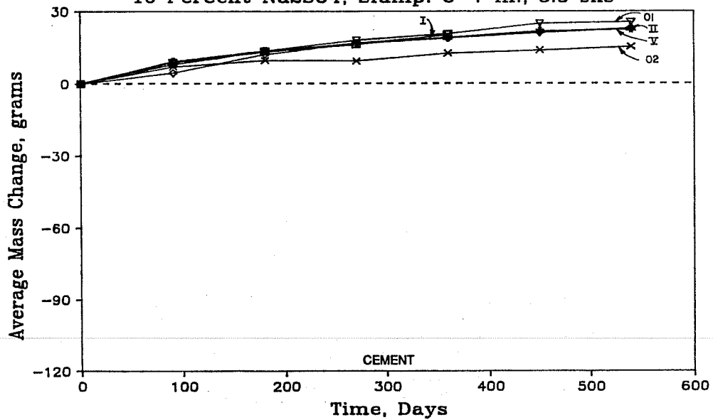
Figure 7.27 Effect of cement type on sulfate resistance.
