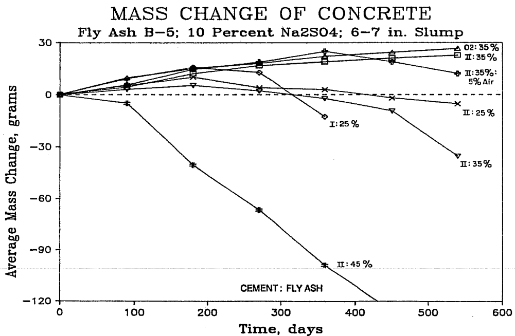
Figure 7.69 Sulfate mass loss of concrete containing fly ash B-5.
