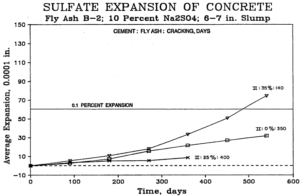
Figure 7.60 Sulfate expansion of concrete containing fly ash B-2.
