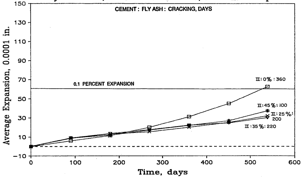
Figure 7.58 Sulfate expansion of concrete containing fly ash B-1.
