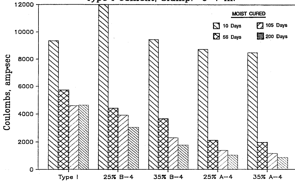
Figure 6.3 Chloride ion permeability of concrete containing Type I cement.
