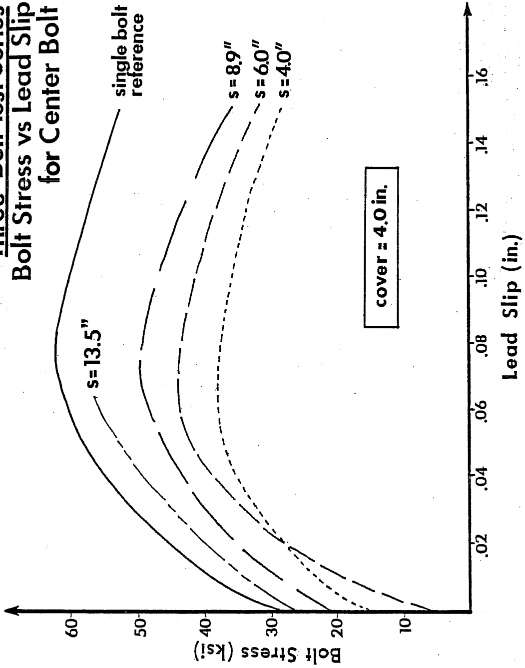
Fig. 5.10 Stress-slip curve for center bolts of 3-bolt groups
