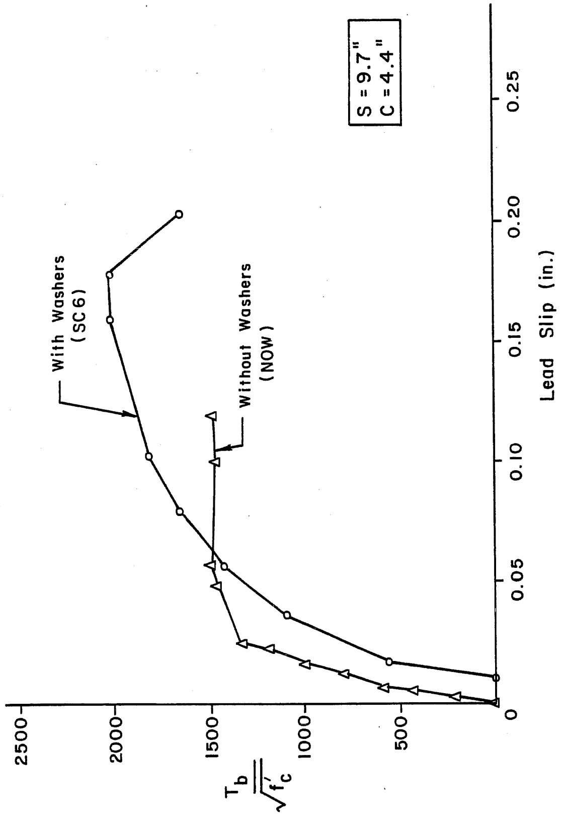
Fig. 5.13 Effect of reduced bearing area: SC6, NOW
