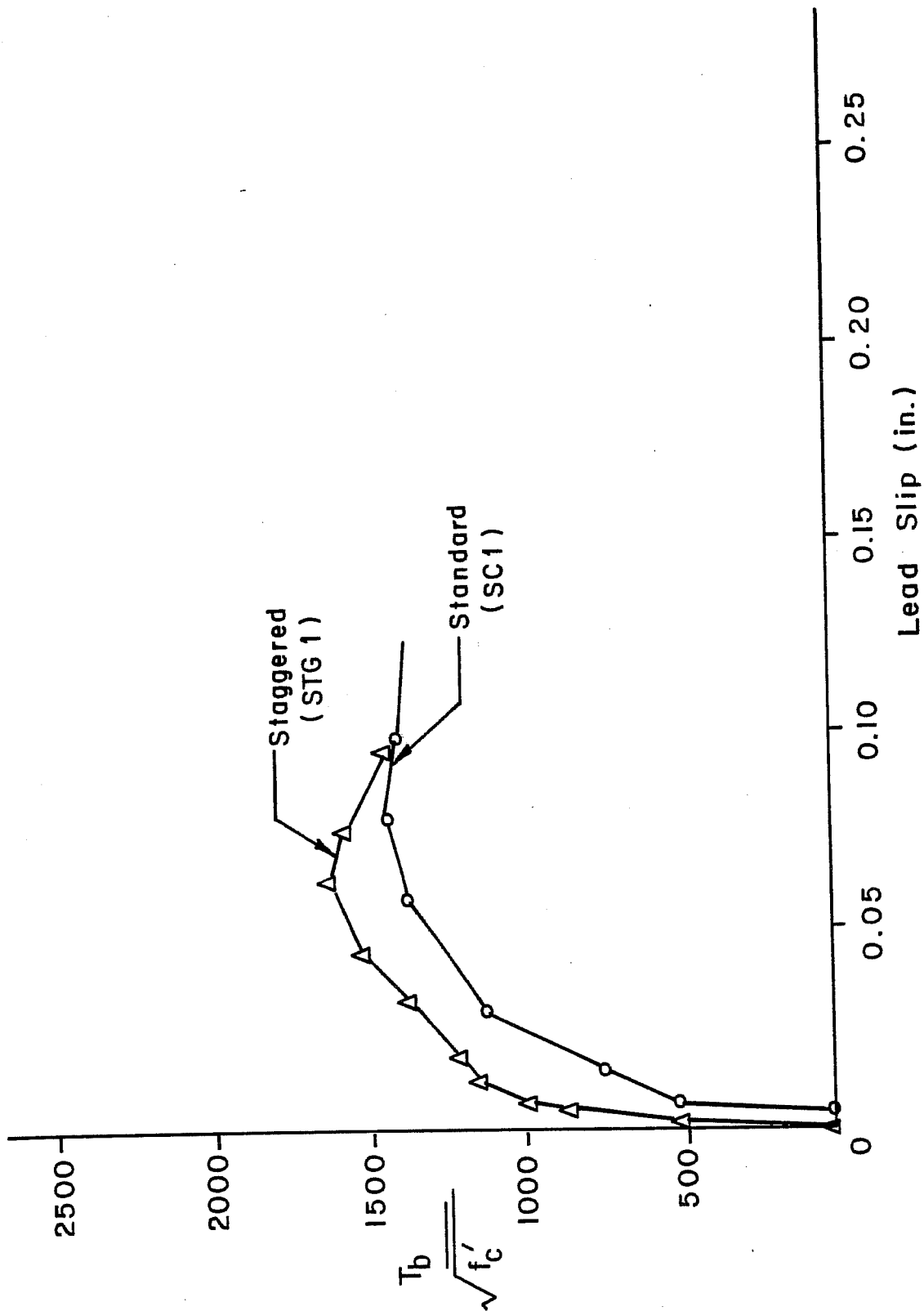
Fig. 5.11 Effect of bolt staggering: SC1, STG1
