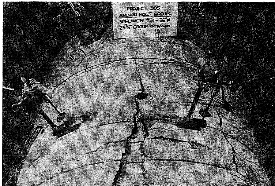
Fig. 4.19 Splitting and uplift of cover, SC6
