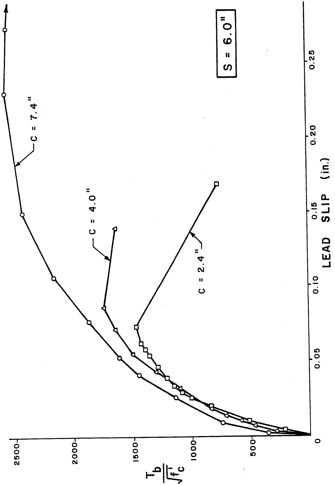
Fig. 5.5 Effect of clear cover: TB5, TB7, TB9
