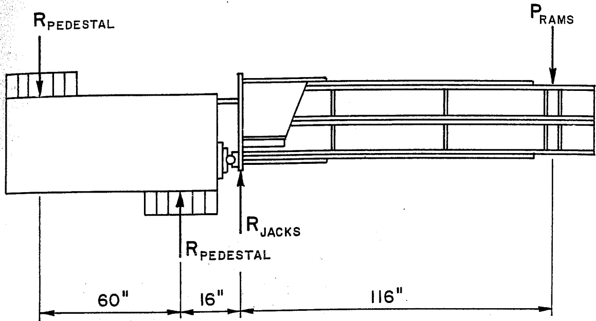
(a) Specimen and loading beam
