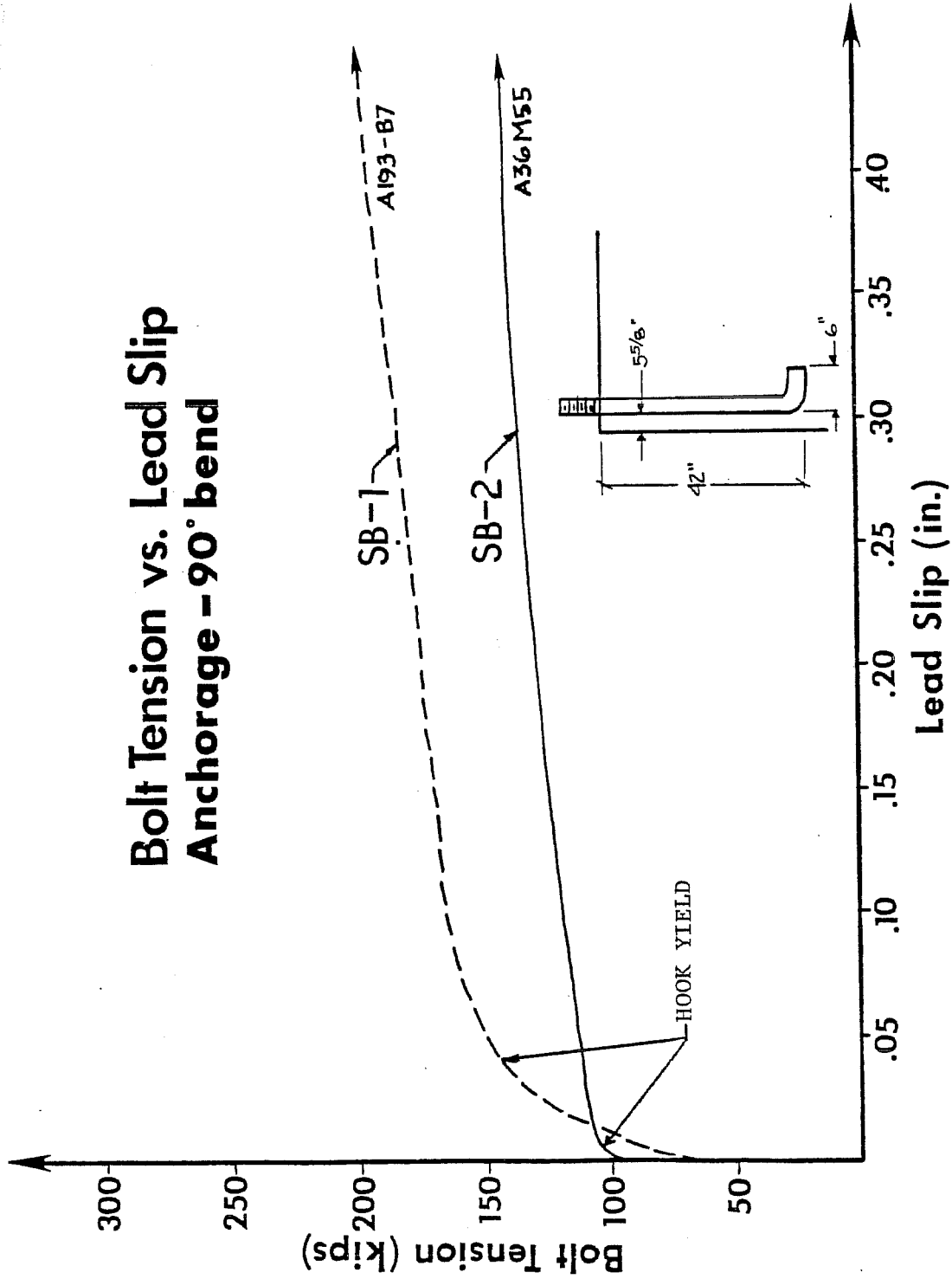
Fig. 7.7 Load-slip curves for tests SB1 and SB2
