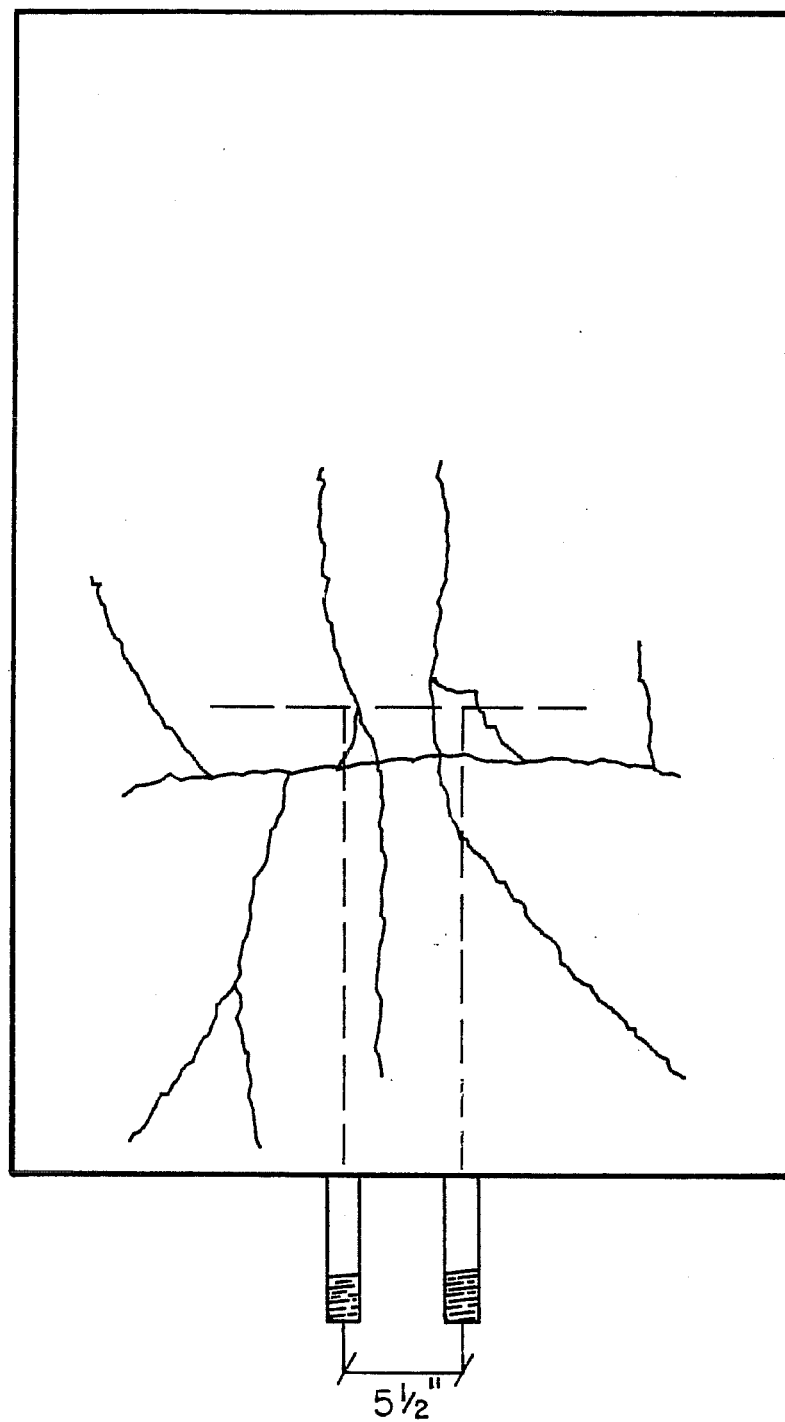
Fig. 7.12 Crack pattern of test TBI
