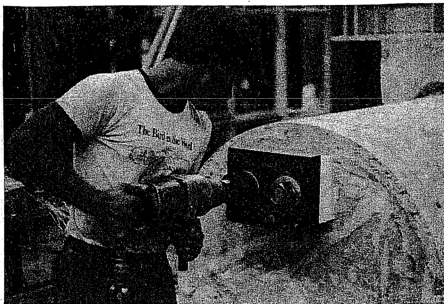
(c) Tightening with pneumatic wrench
