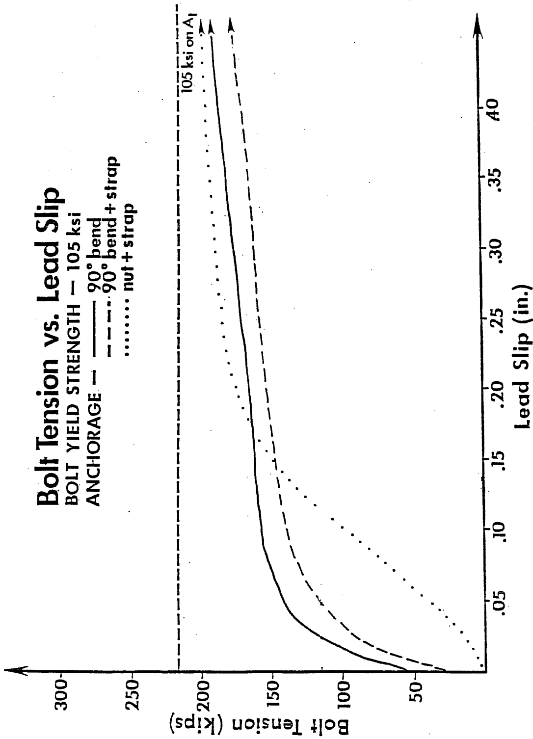
Fig. 7.13 Load-slip curves for tests SB1, SB3 and SB5
