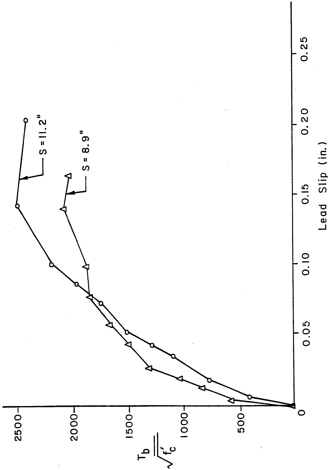
Fig. 5.4 Effect of bolt spacing: SC2, SC4
