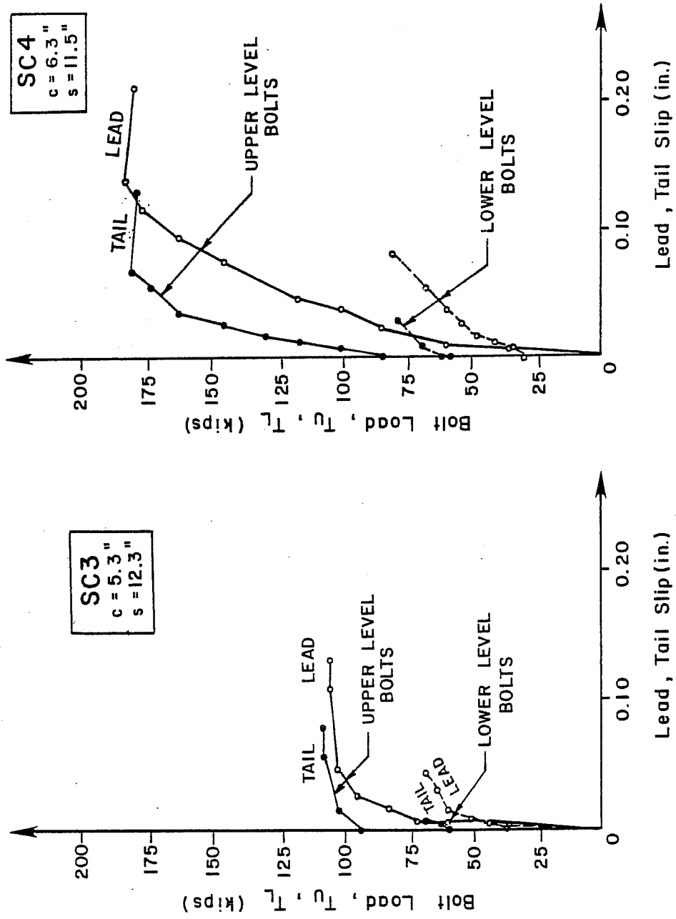
Fig. 4.6 Load-slip curves, SC3 and SC4
