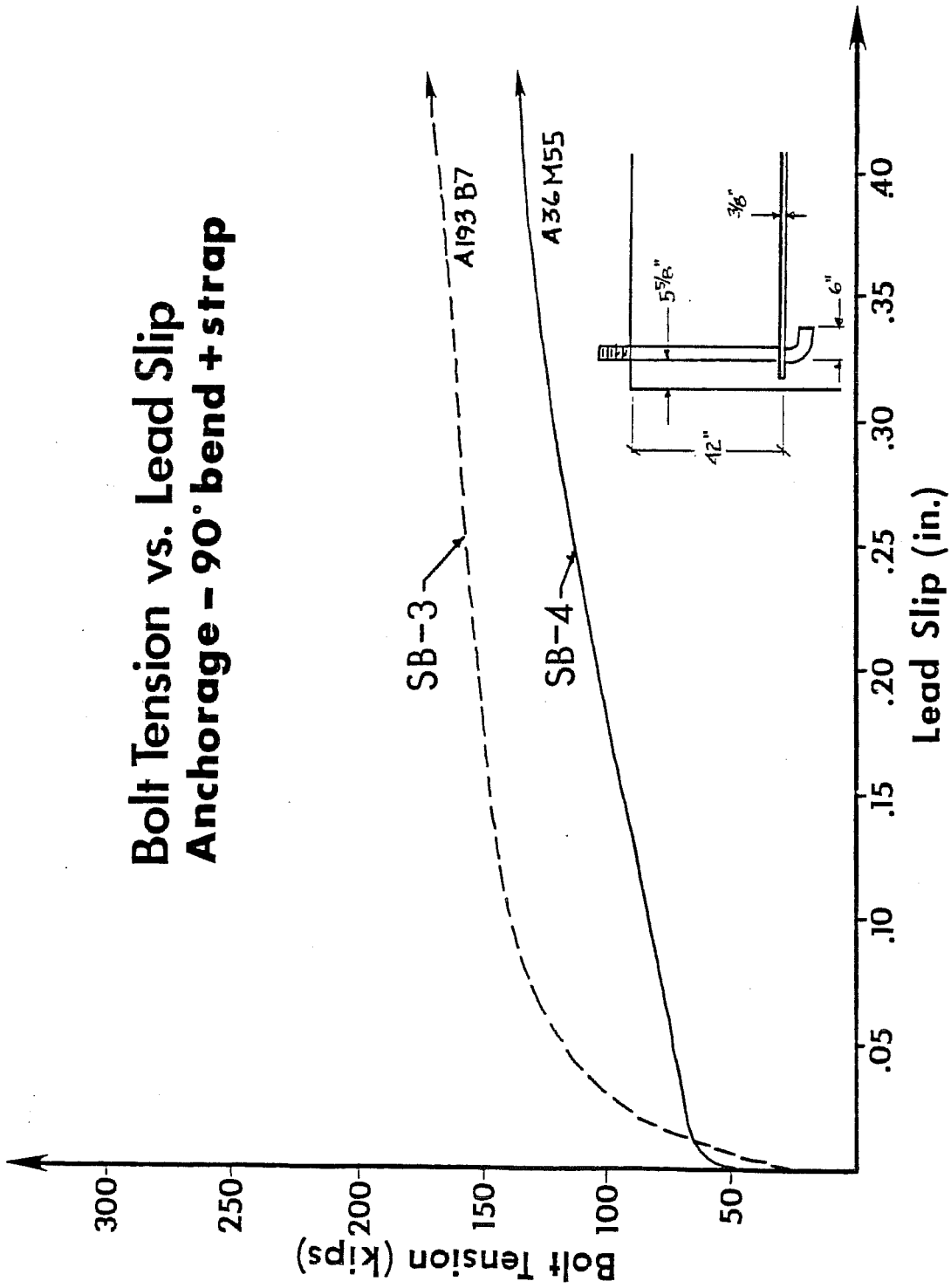
Fig. 7.8 Load-slip curves for tests SB3 and SB4
