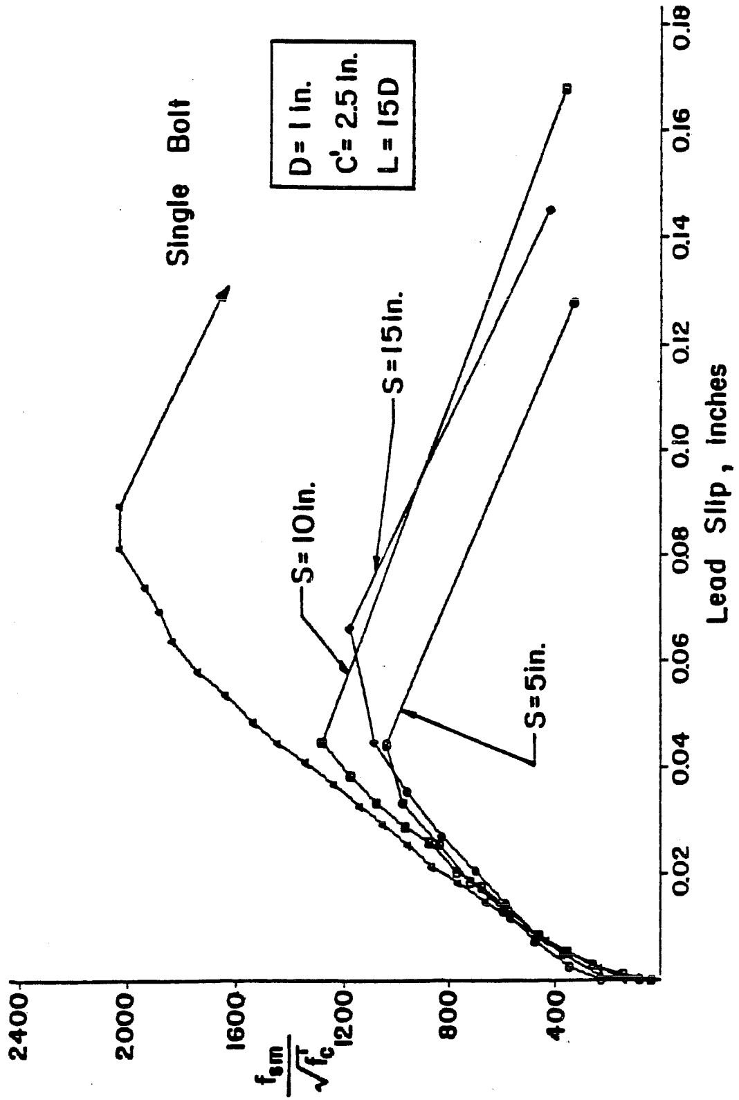
Fig. 1.2 Comparison of lead slip-lead stress curves of bolts in a group
