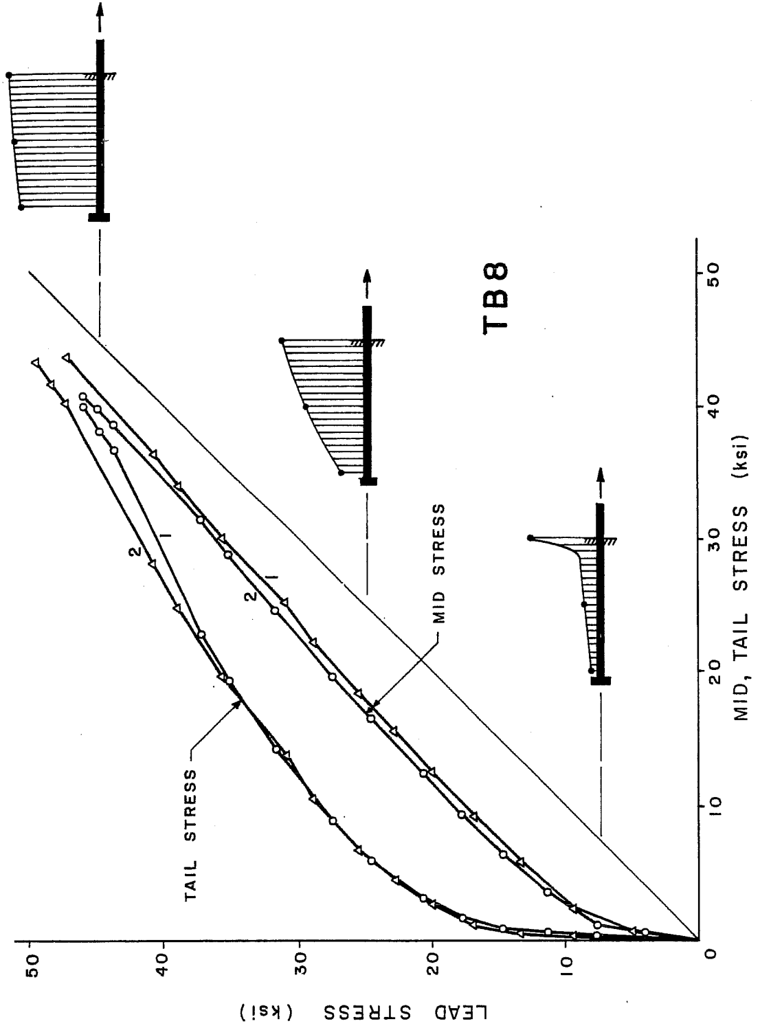
Fig. 4.4 Stress variation along bolt
