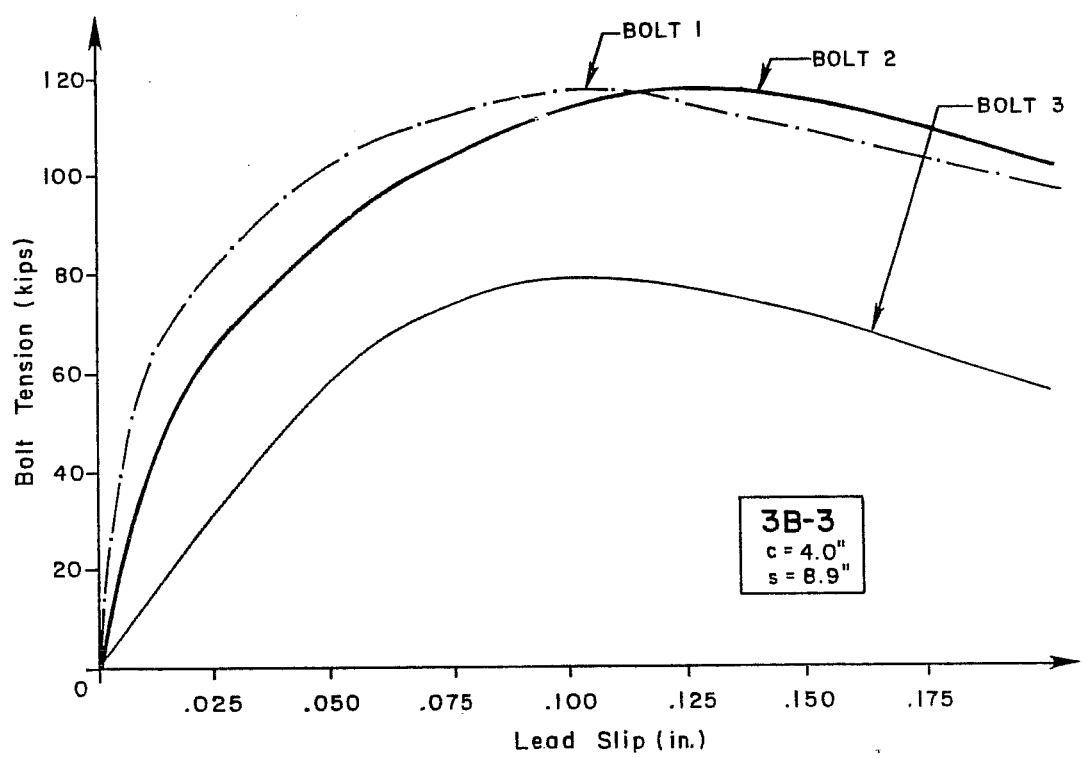
Fig. 4.14 Load-slip curves, 3B-1 and 3B-3
