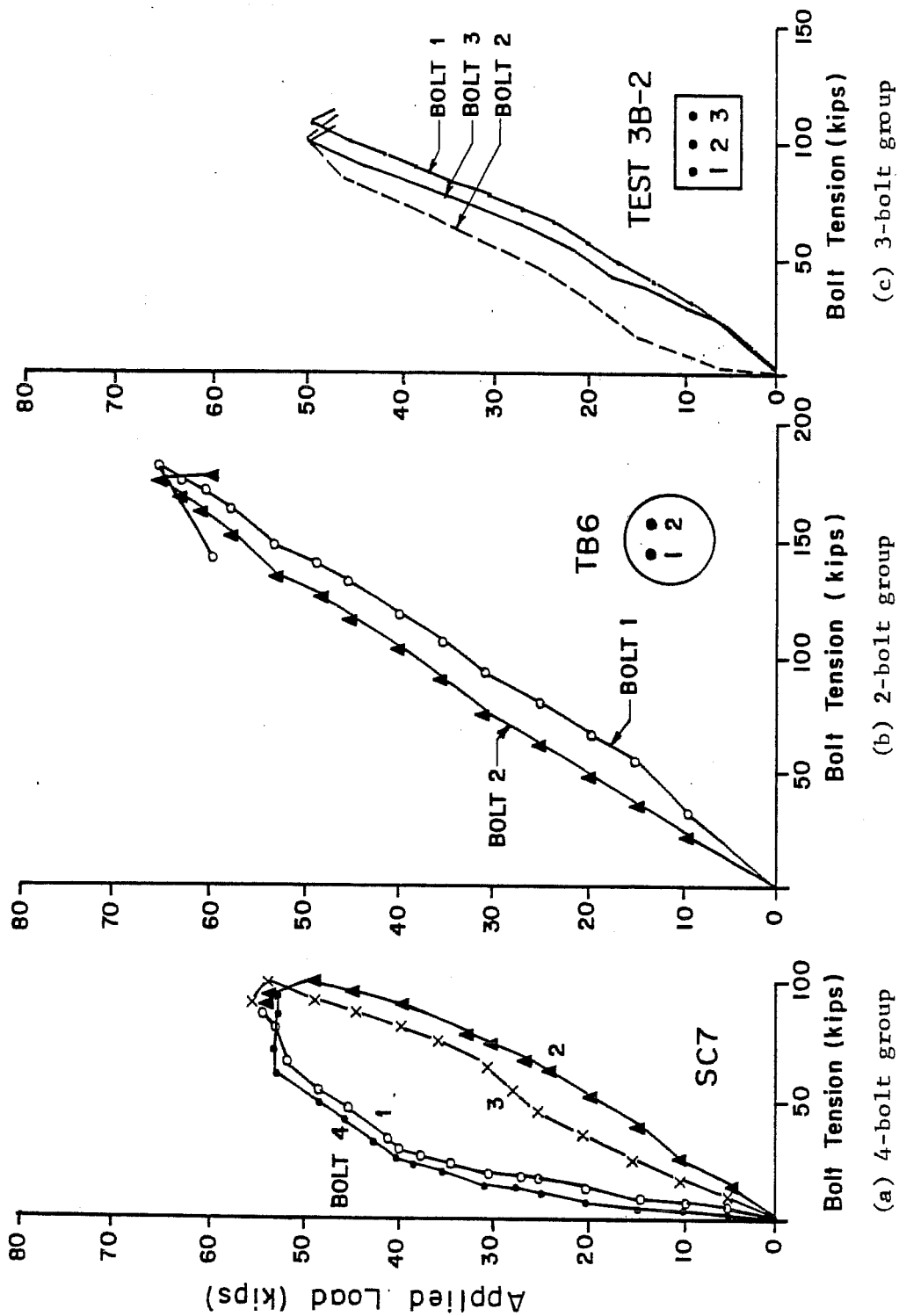
Fig. 4.3 Bolt stress variation during testing
