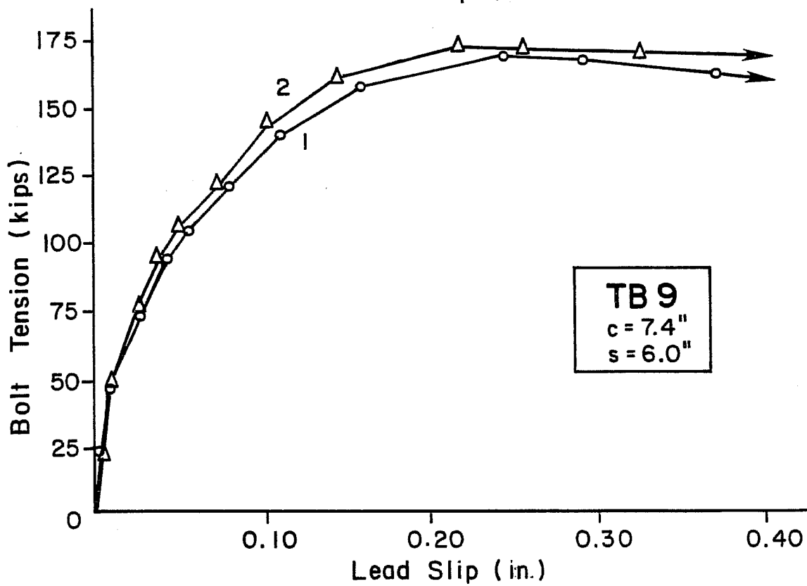
Fig. 4.13 Load-slip curves, TB8 and TB9
