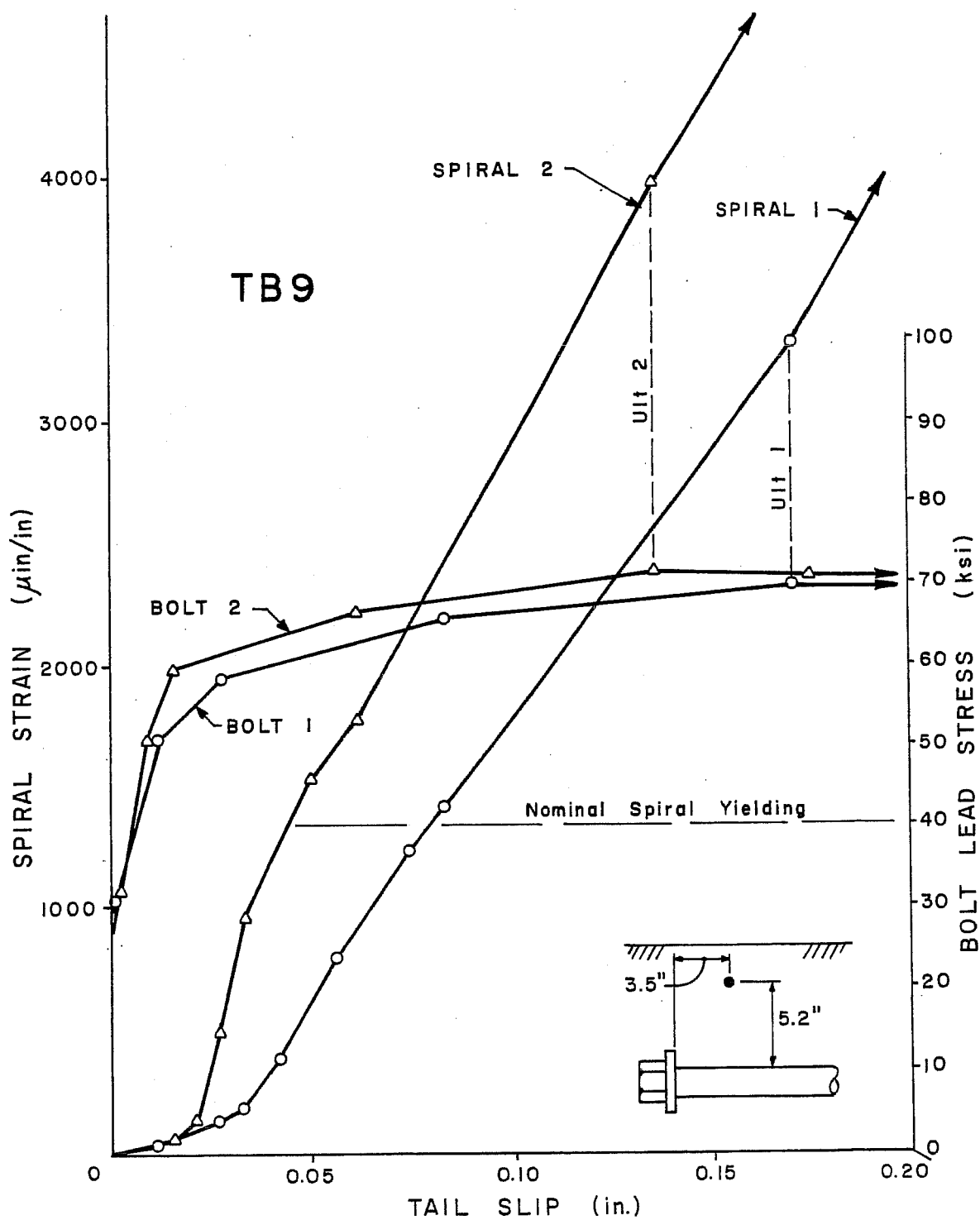
Fig. 4.26 Strains in spiral reinforcement, TB9
