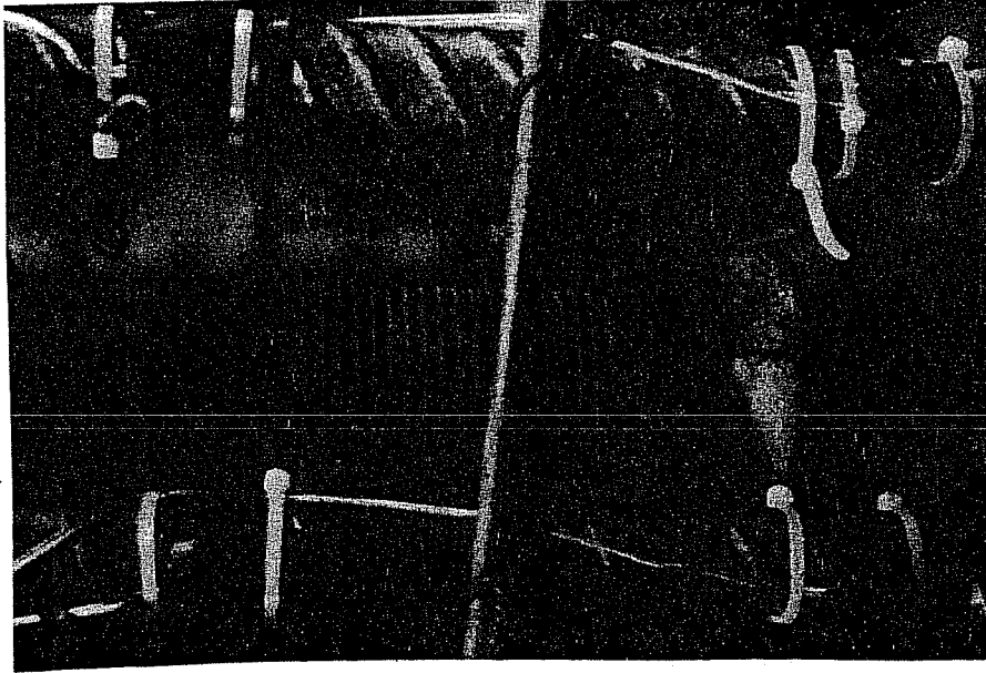
(b) Nut/steel strap anchorage
