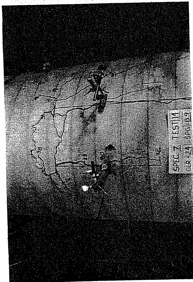
(a) Small cover, TB4
