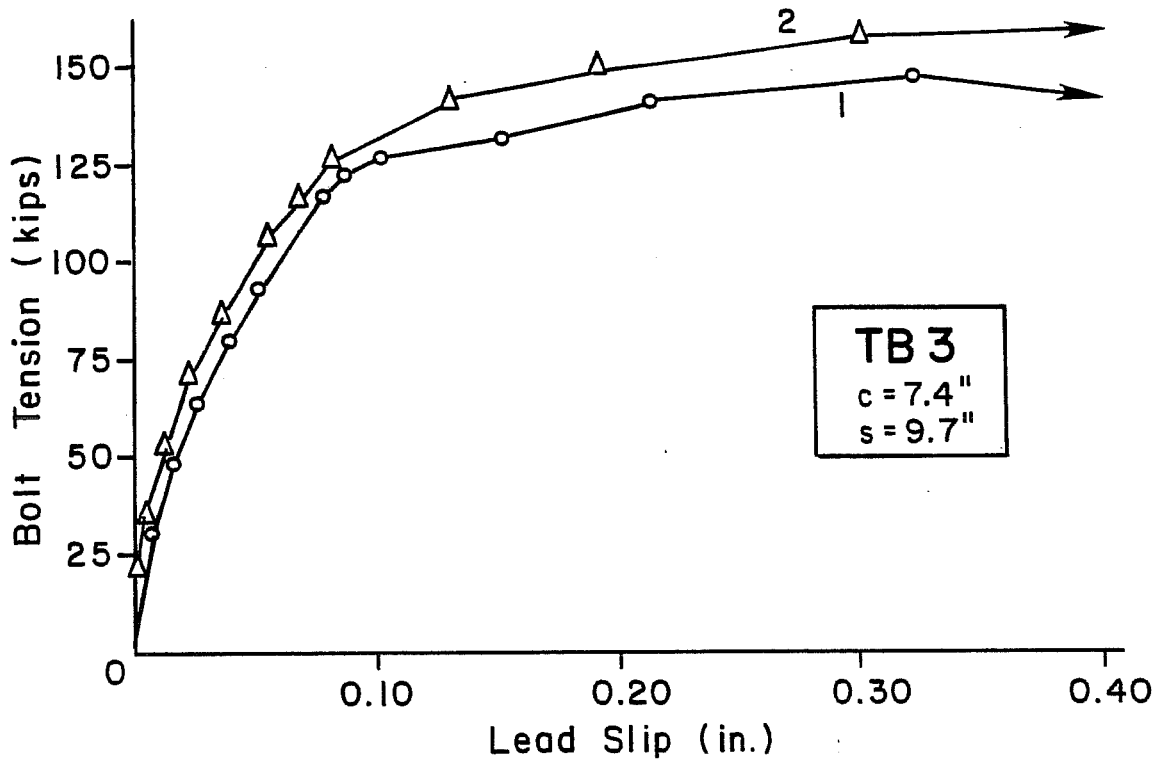
Fig. 4.10 Load-slip curves, TB1 and TB3
