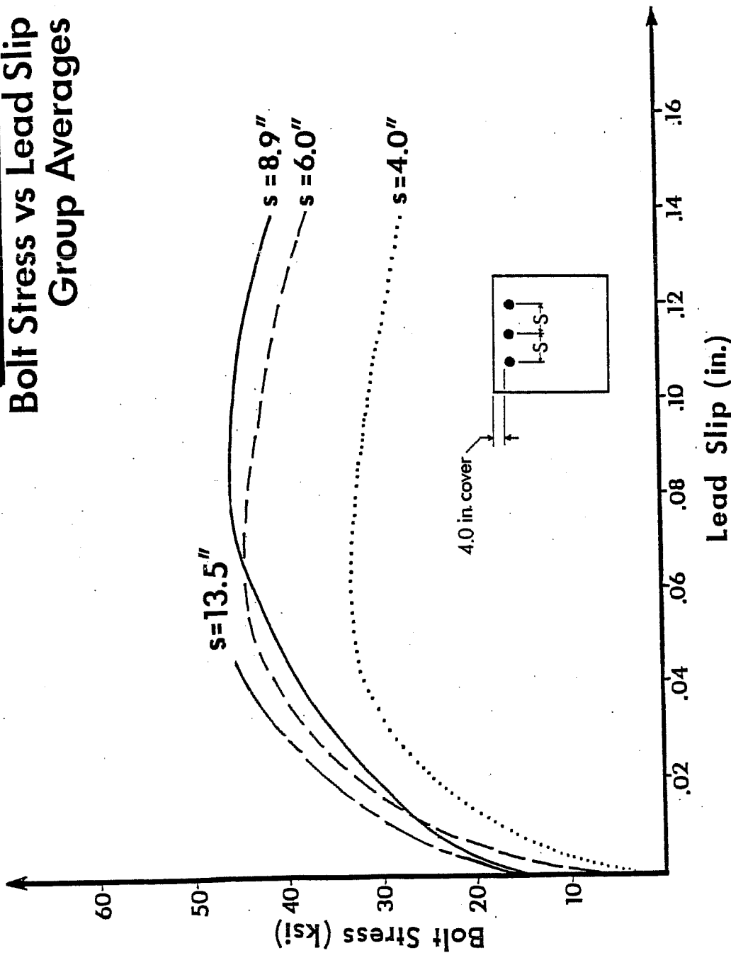
Fig. 5.9 Average stress-slip curves for 3-bolt groups
