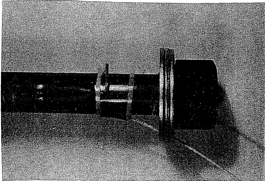
(b) Tail slip wire and gages
