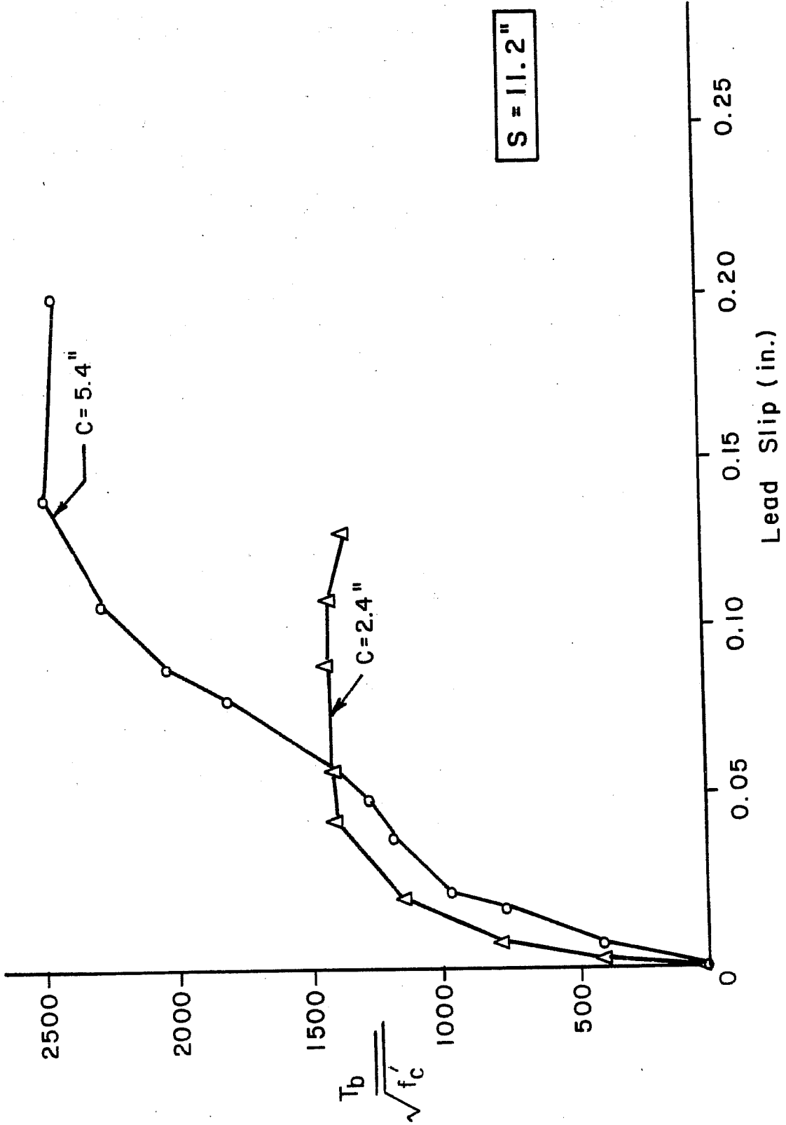
Fig. 5.8 Effect of clear cover: SCI, SC4
