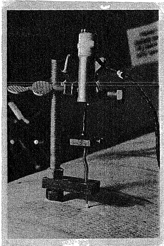
Fig. 3.16 Slip measurement device mounted on specimen
