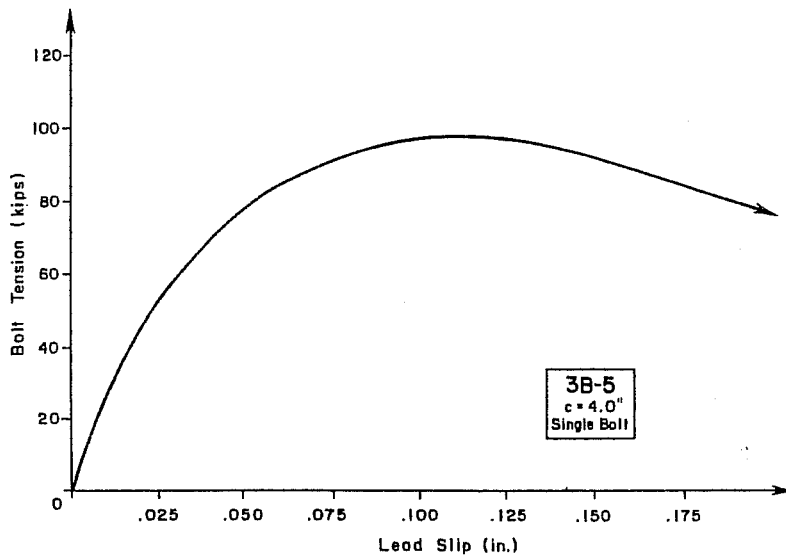
Fig. 4.15 Load-slip curves, 3B-2, 3B-4 and 3B-5
