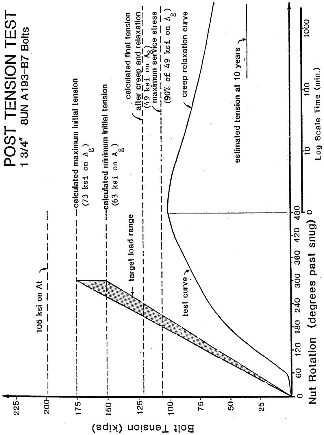
Fig. 7.18 Results of post-tension test
