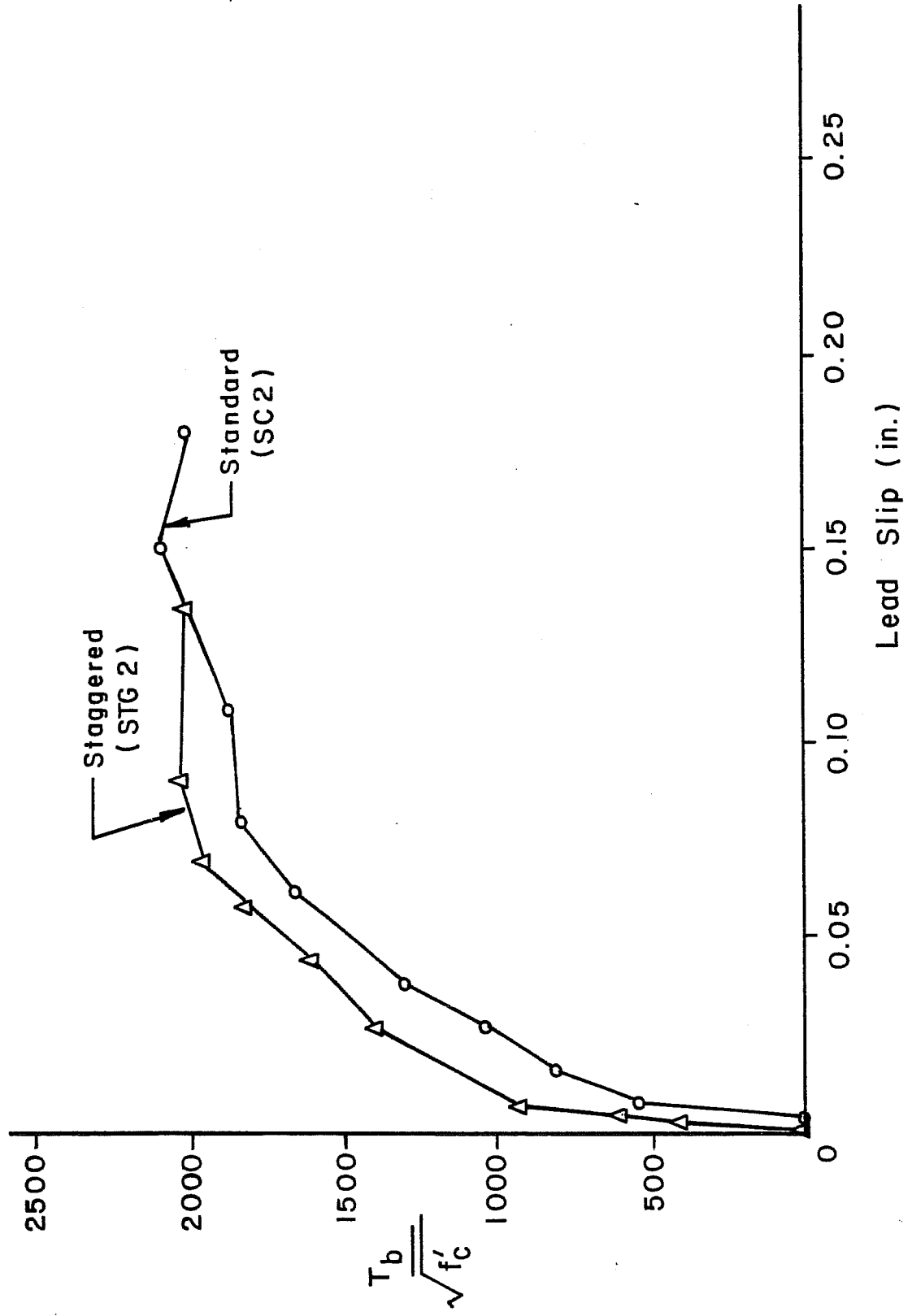
Fig. 5.12 Effect of bolt staggering: SC2, STG2
