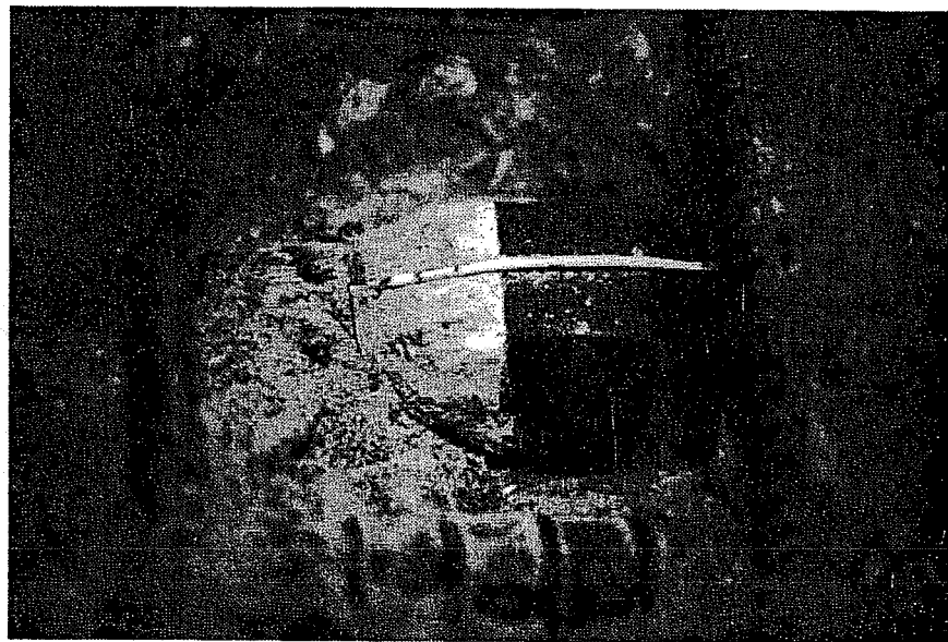
Fig. 4.16 Cone of crushed and compacted concrete in front of anchorage device
