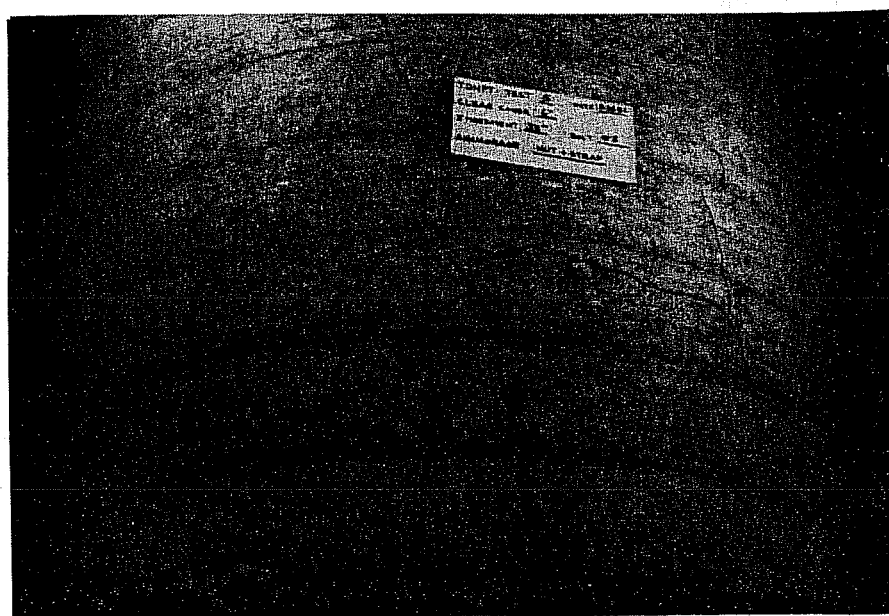
Fig. 7.11 Crack pattern of test SB5
