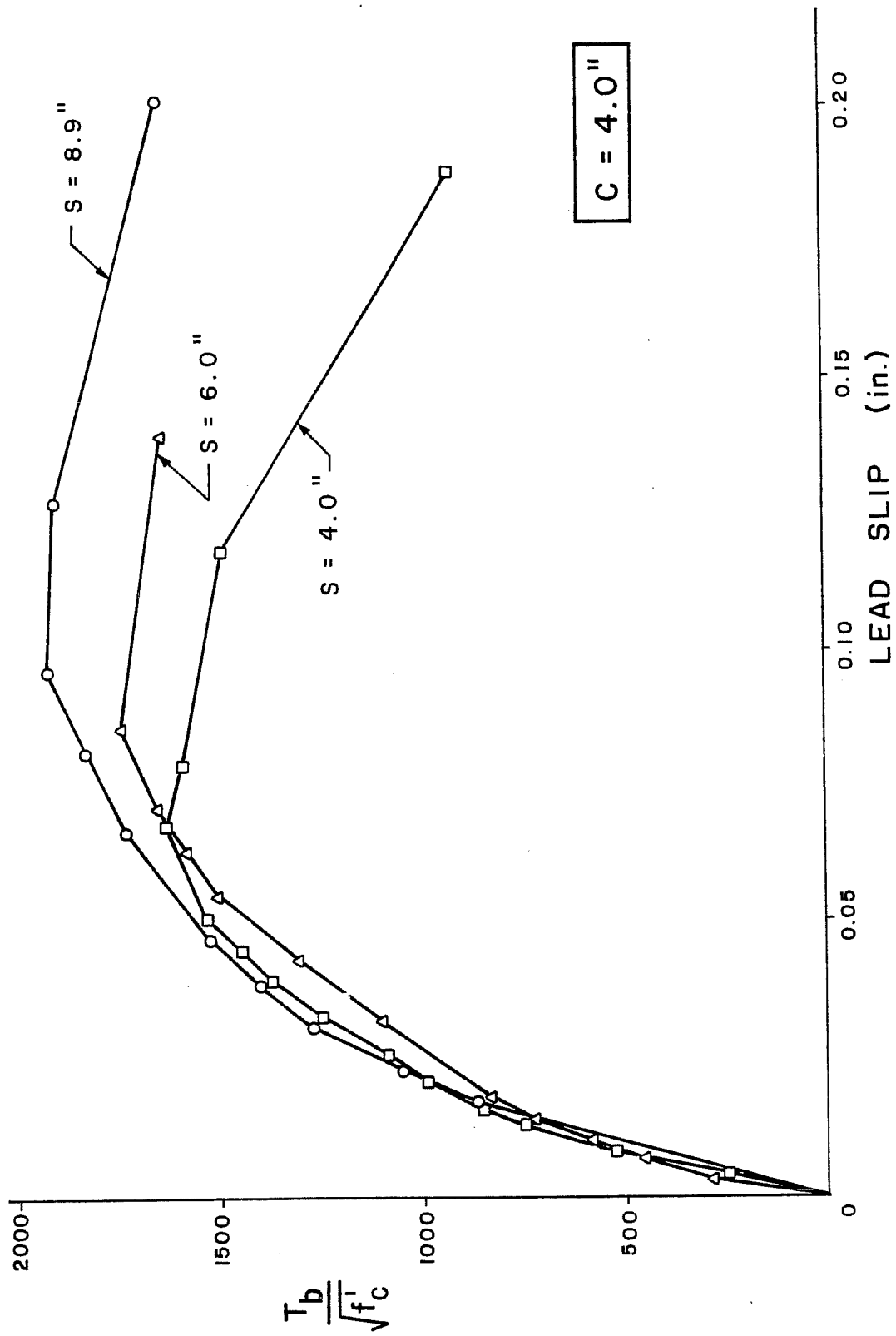
Fig. 5.2 Effect of bolt spacing: TB1, TB5, TB8
