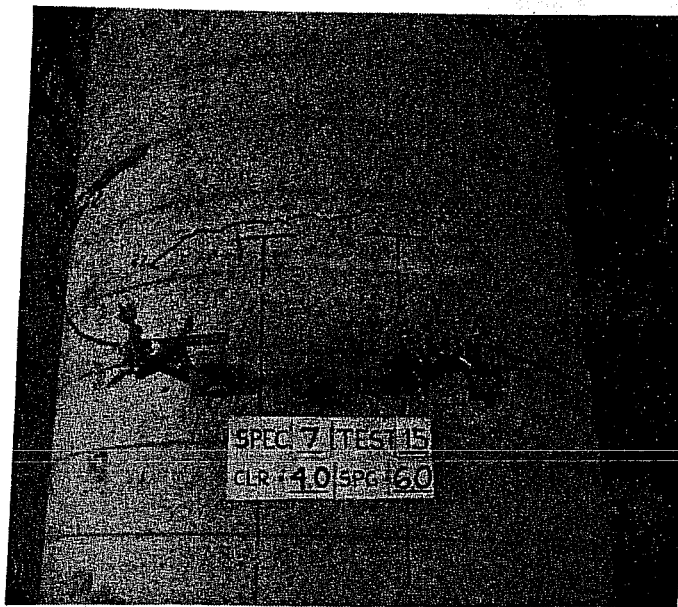
(a) Initial cracking
