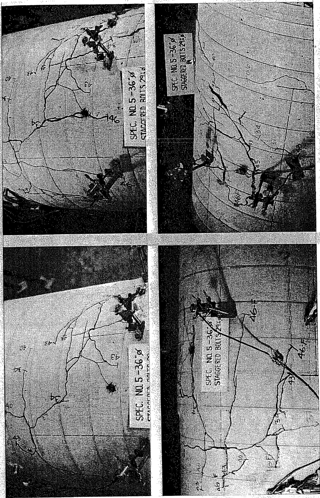
Fig. 4.20 Crack patterns, staggered bolts: STG1
