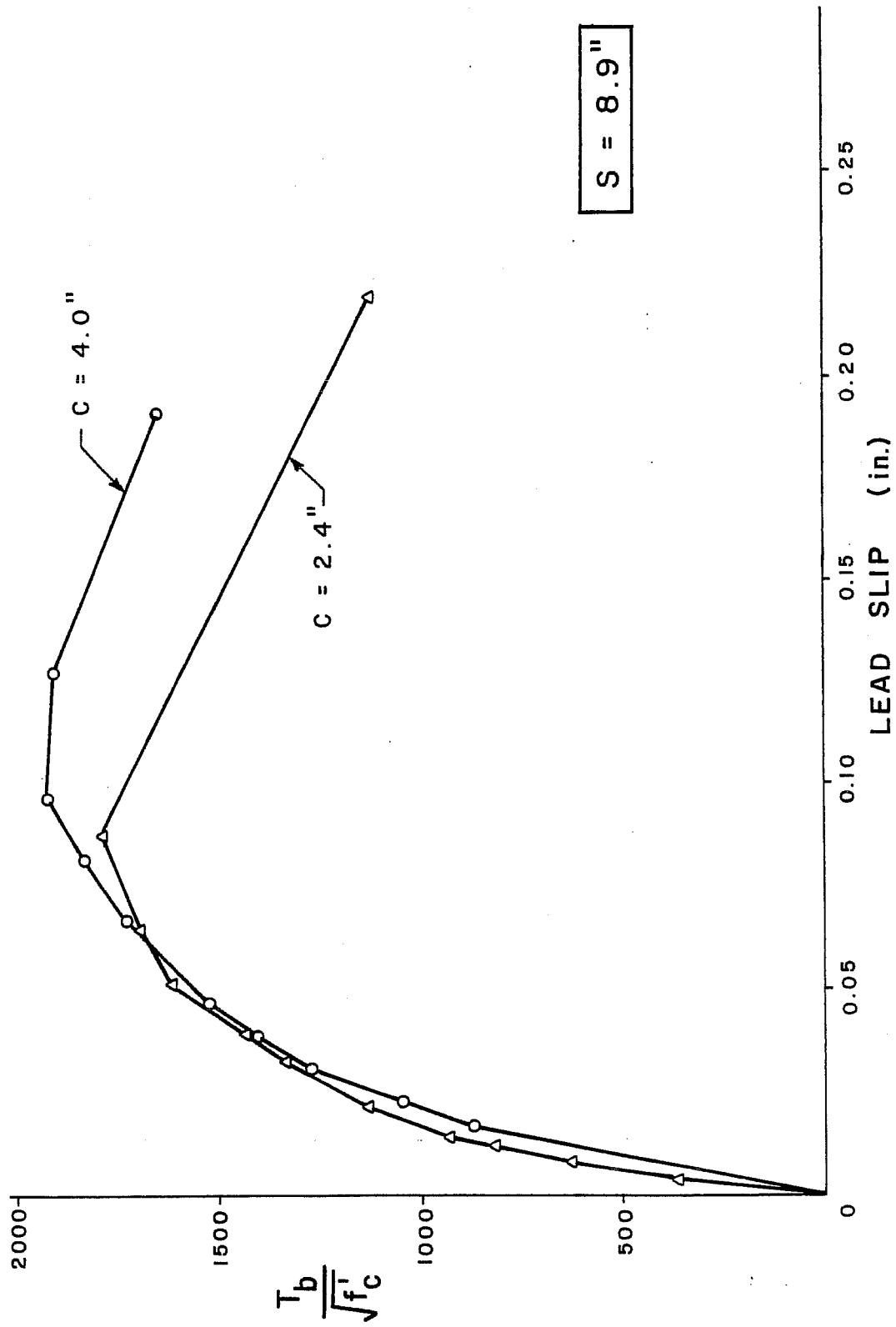
Fig. 5.6 Effect of clear cover: TB1, TB4
