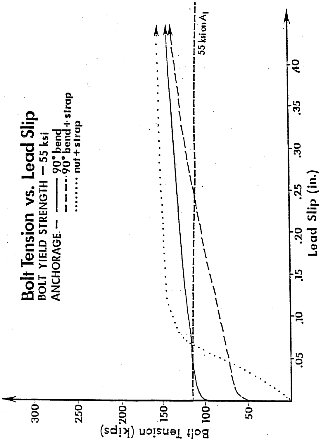
Fig. 7.14 Load-slip curves for tests SB2, SB4 and SB6
