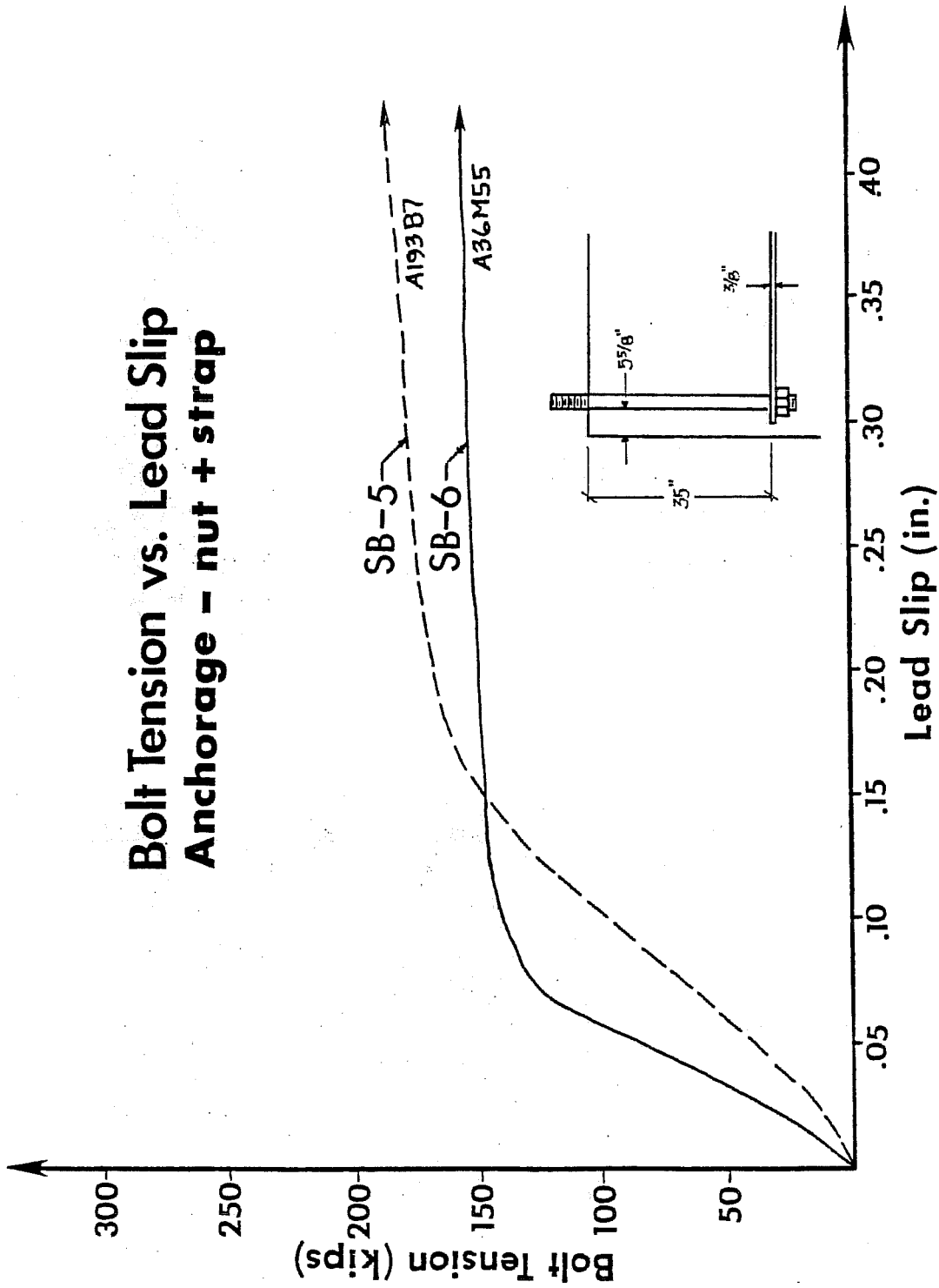
Fig. 7.9 Load-slip curves for tests SB5 and SB6
