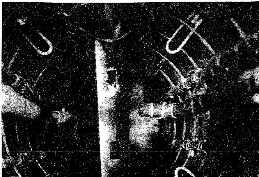
(b) Plan view of specimen 1 prior to casting
