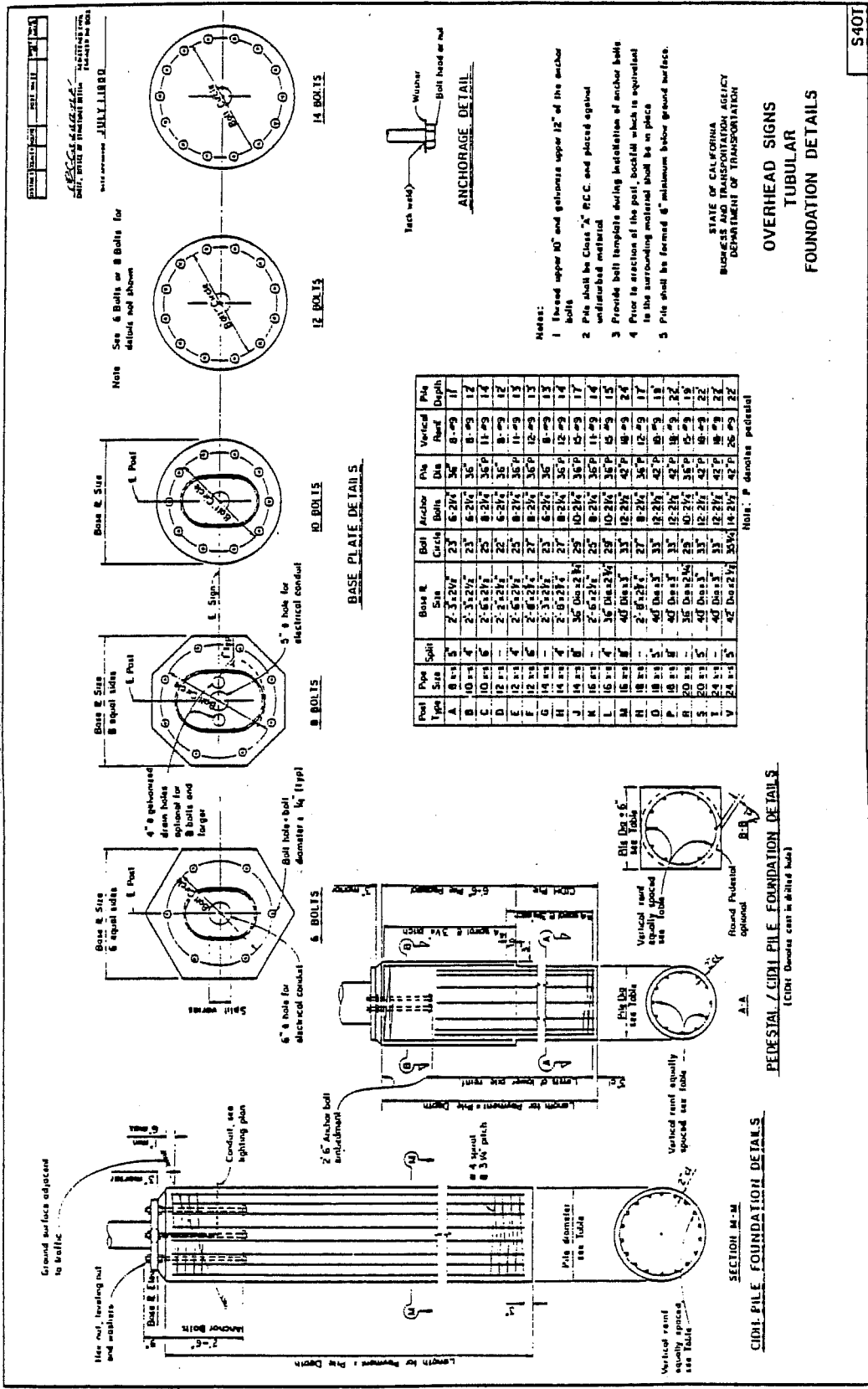
Fig. 2.2 Overhead sign support (California Department of Transportation)
