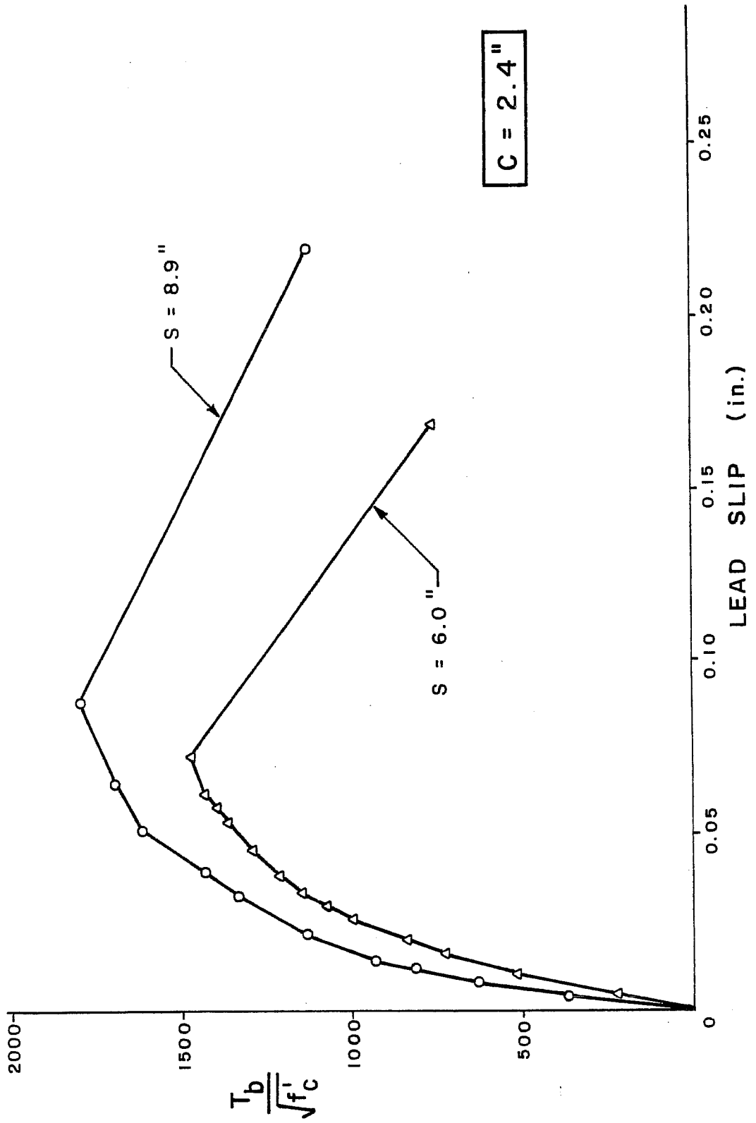
Fig. 5.3 Effect of bolt spacing: TB4, TB7
