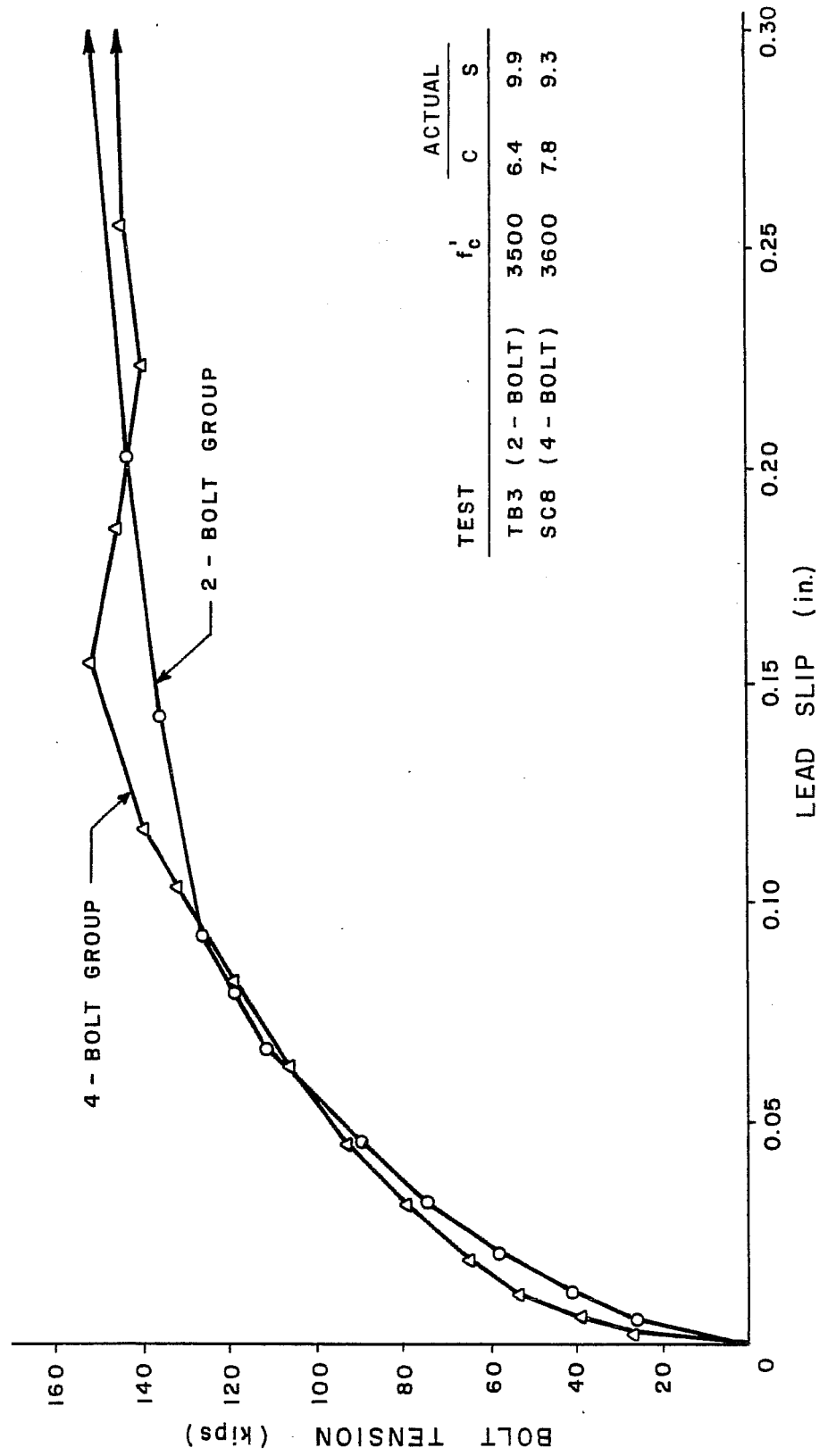
Fig. 5.1 Bolt tension vs. lead slip for 2-bolt and upper bolts in 4-bolt groups
