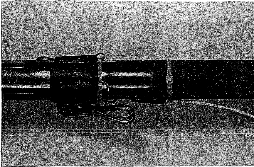
(a) Lead slip wire and gages
