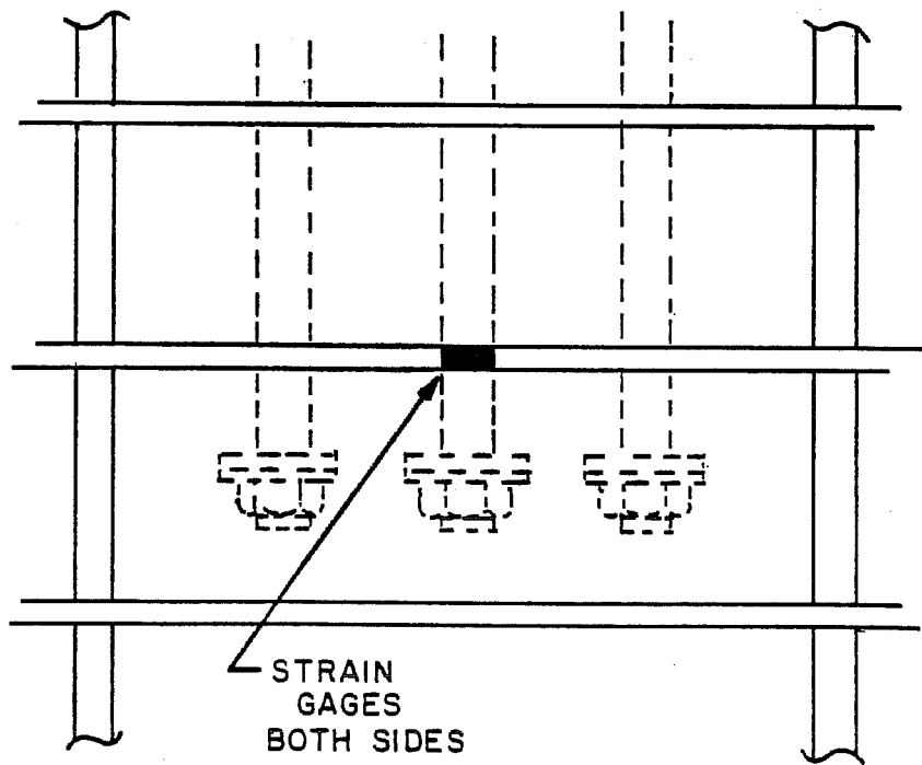
Fig. 3.14 Location of transverse reinforcement instrumentation
