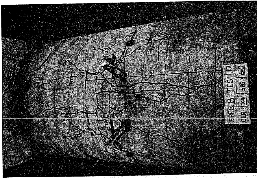
(b) Large cover, TB9
