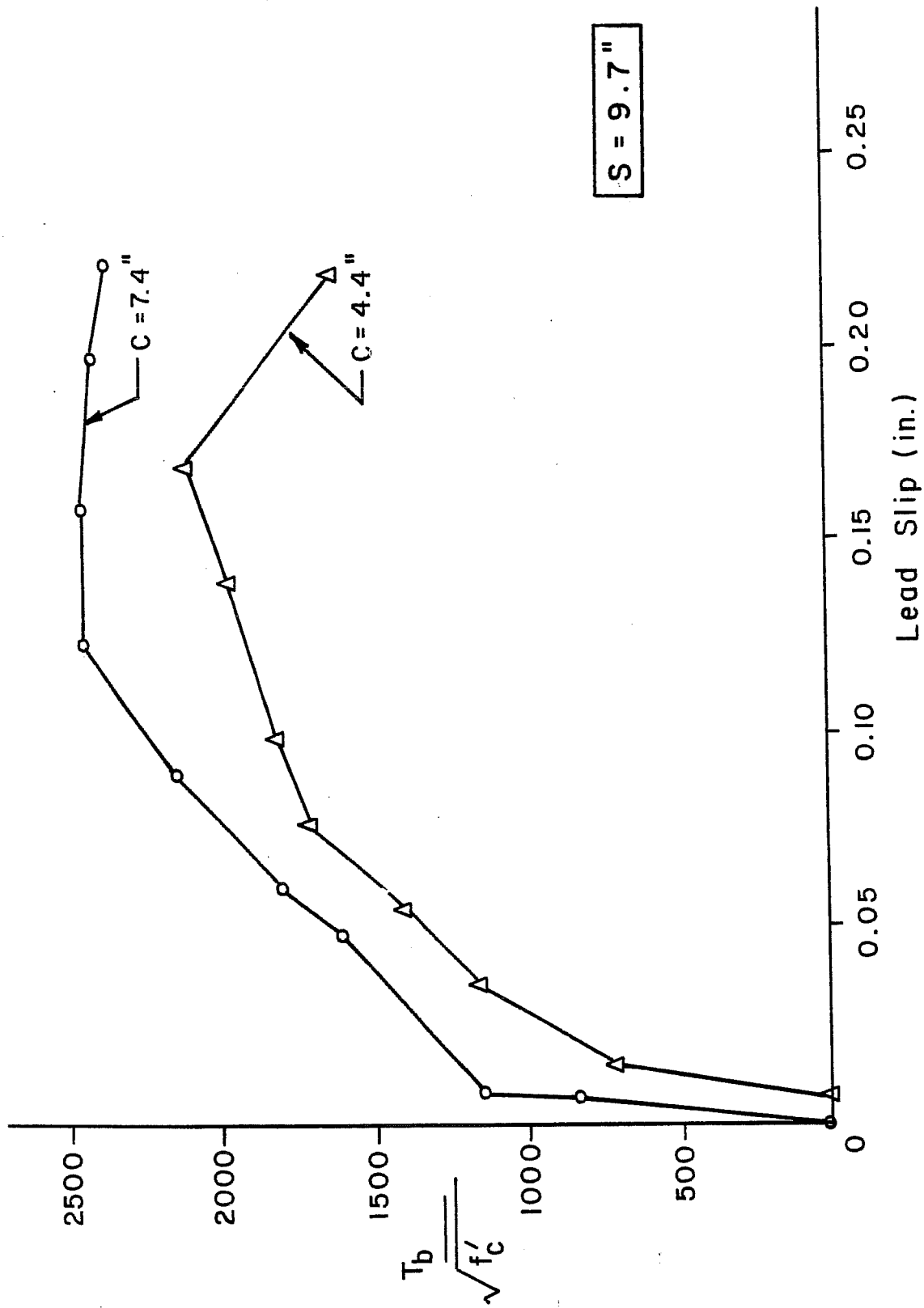
Fig. 5.7 Effect of clear cover: SC6, SC8
